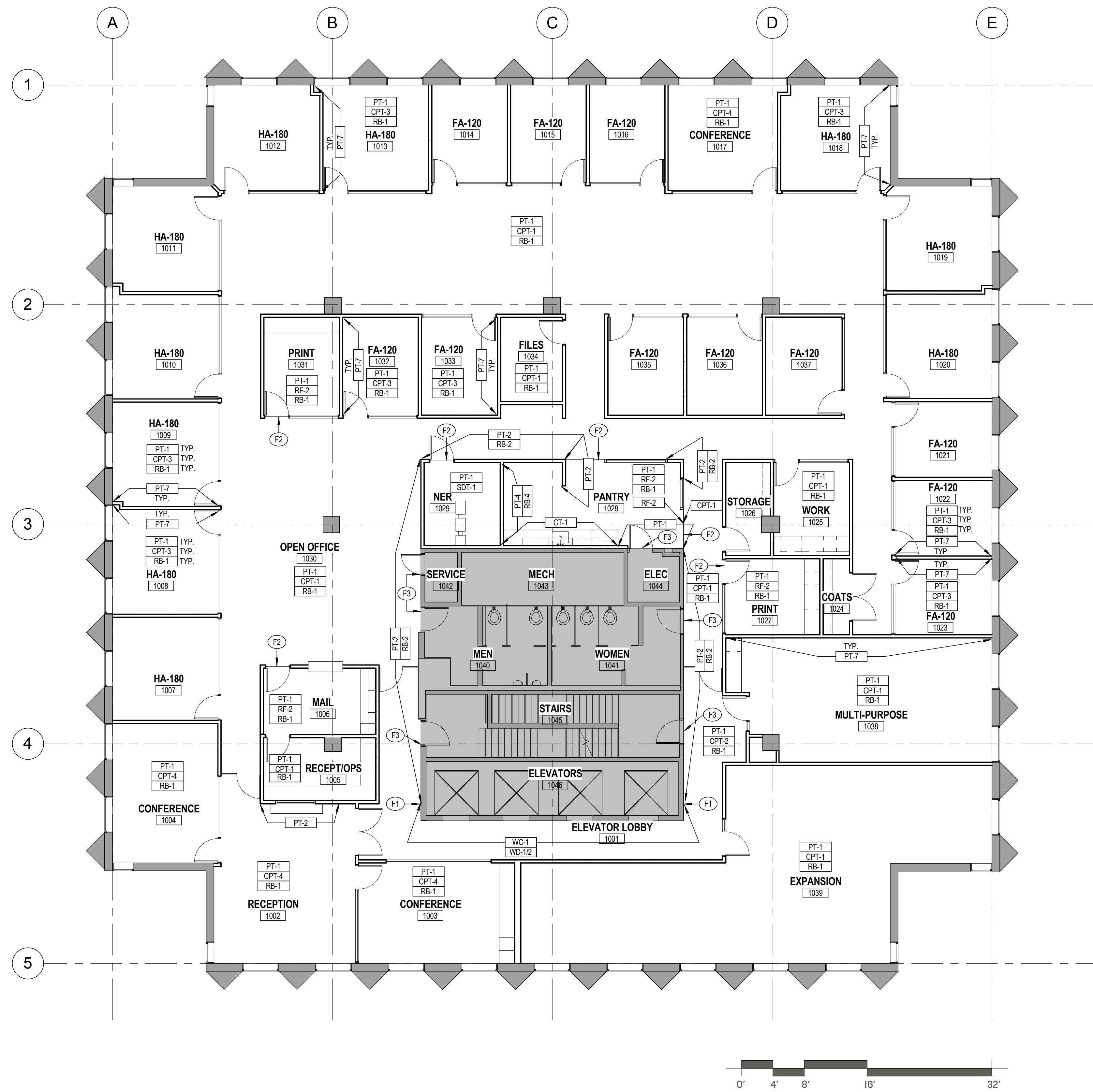
1 10th FLOOR FINISH PLAN 1/8" = 1'-0"
