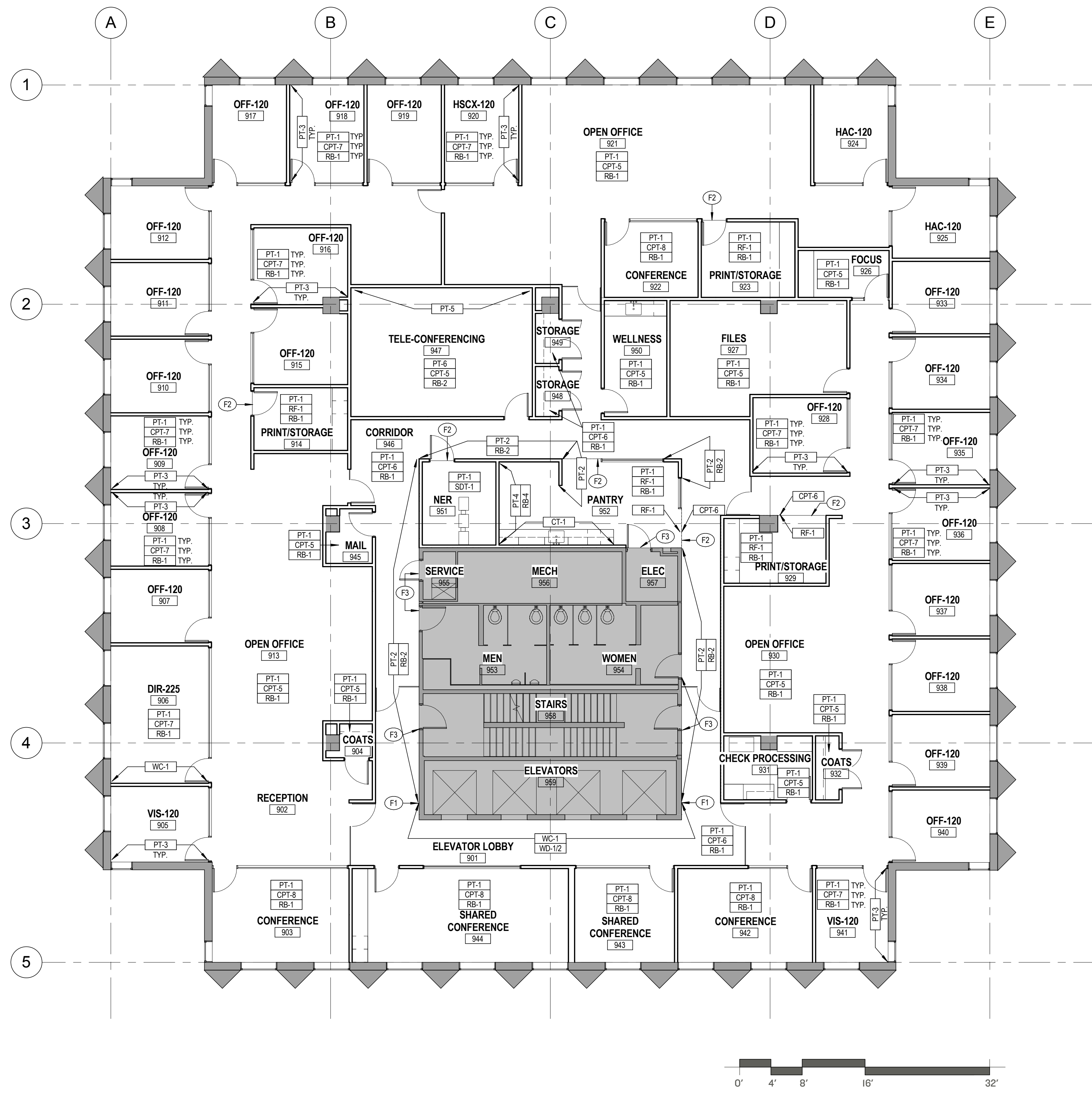
1 9th FLOOR FINISH PLAN 1/8" = 1'-0"
