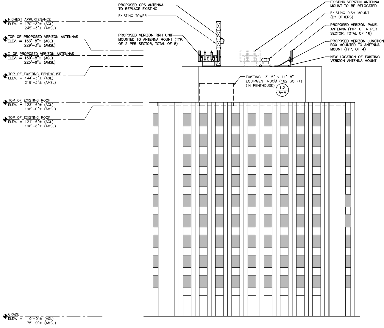
SOUTHWEST ELEVATION 1 A-3 11x17 SCALE: 3/64"=1'-0" 22x34 SCALE: 3/32"=1'-0" GRAPHIC SCALE 0 5'-4" 10'-8" 21'-4" 32'-0"
