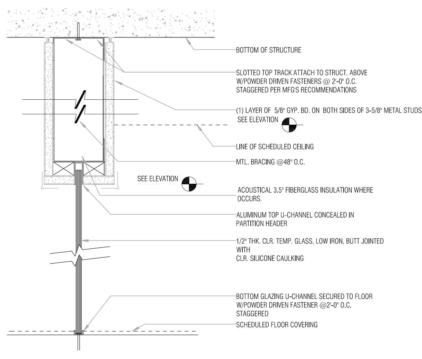
② FULL HT GLASS PARTITION-FRAMELESS 3" = 1'-0"
