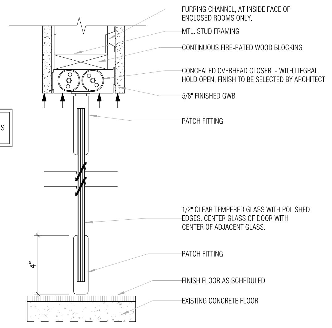
④ CONCEALED CLOSER 3" = 1'-0"
