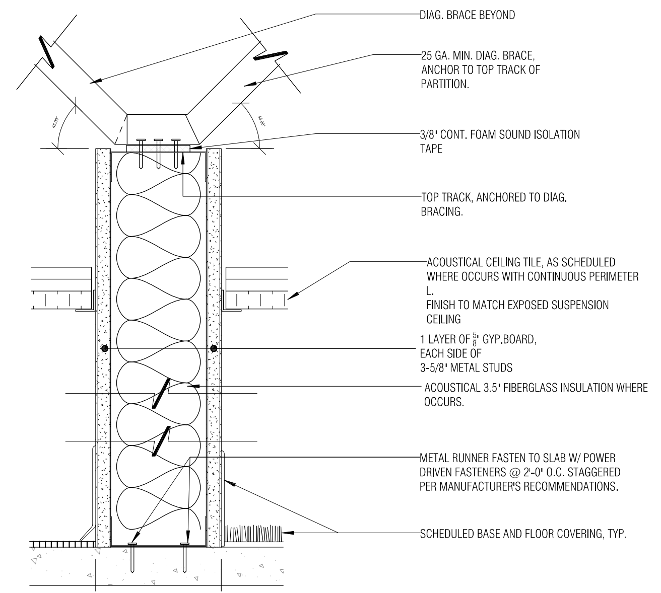
③ NON RATED PARTITION - 6 IN ABOVE CEILING 3" = 1'-0"
