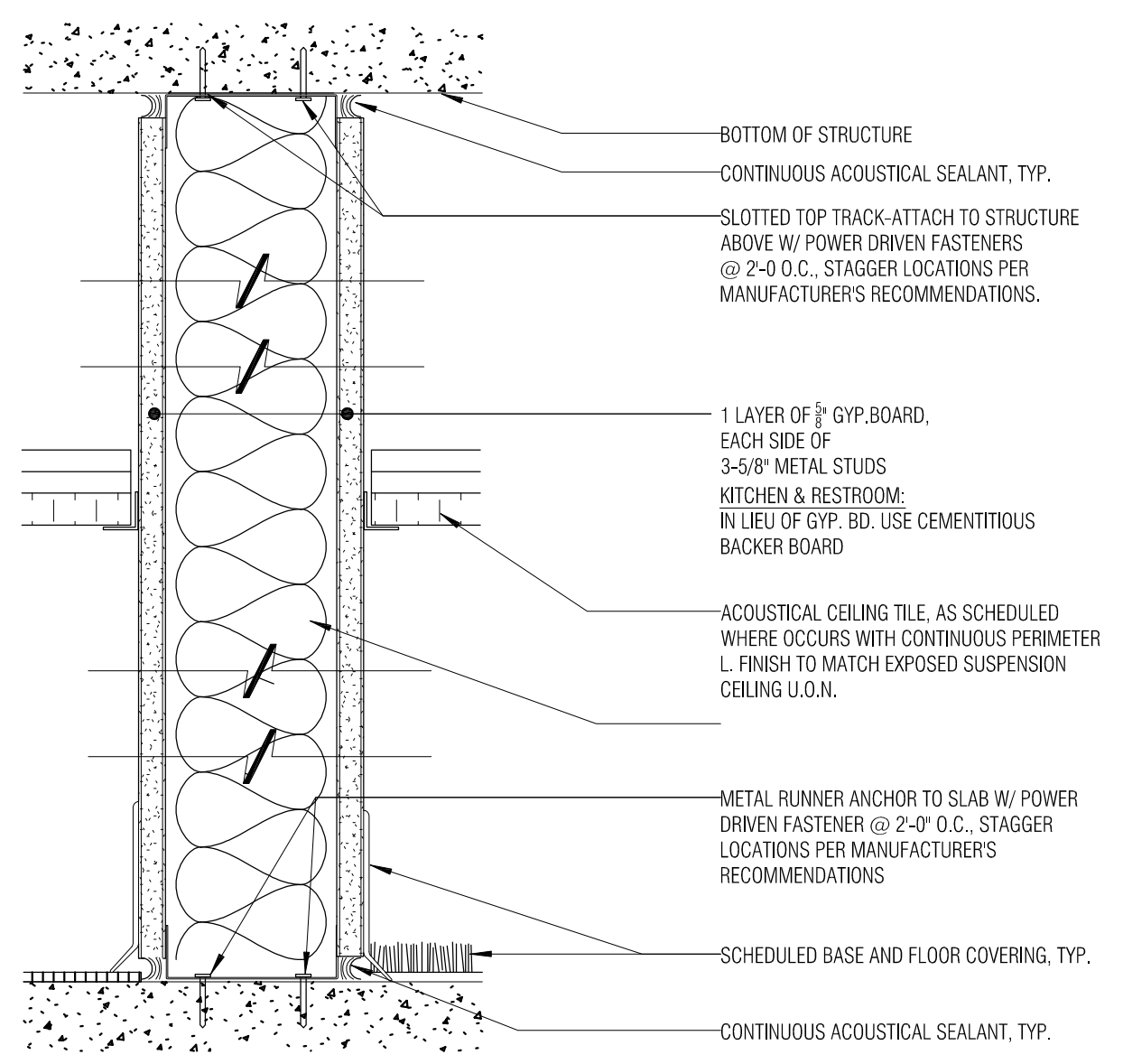
① NON RATED FULL HEIGHT PARTITION 3" = 1'-0"
