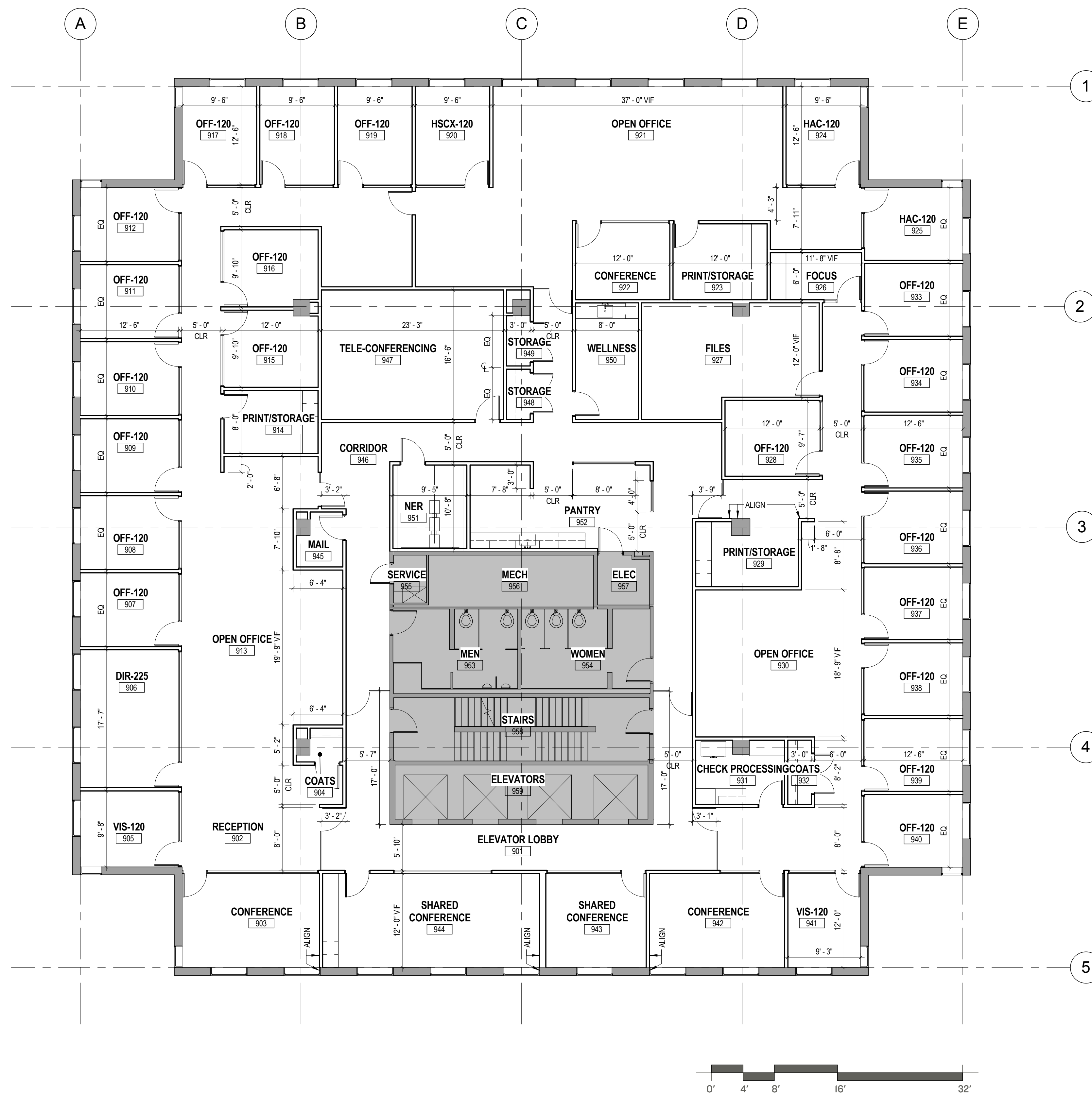
① 9th FLOOR DIMENSION PLAN 1/8" = 1'-0"
