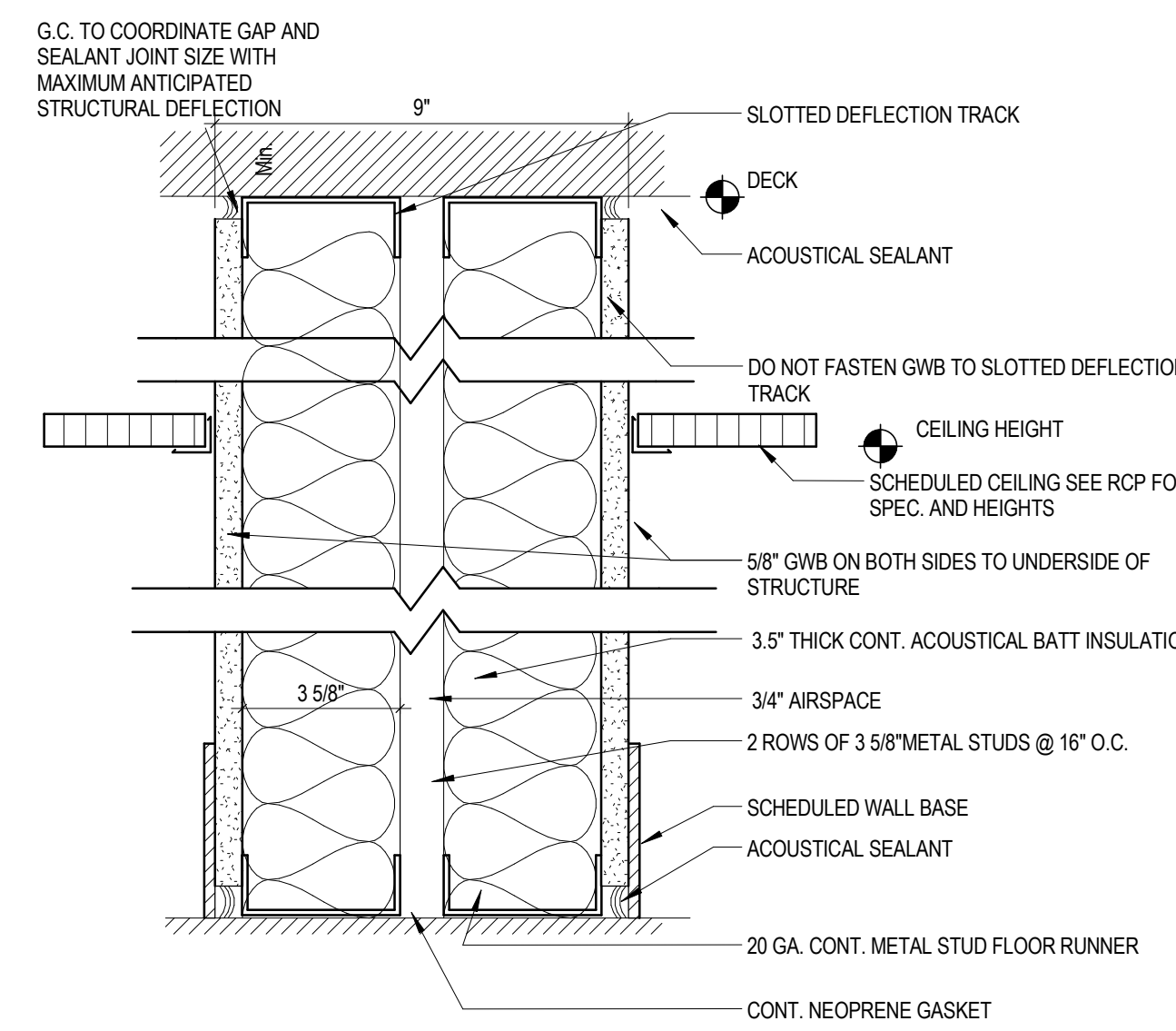
N PARTITION TYPE ACOUSTICAL
