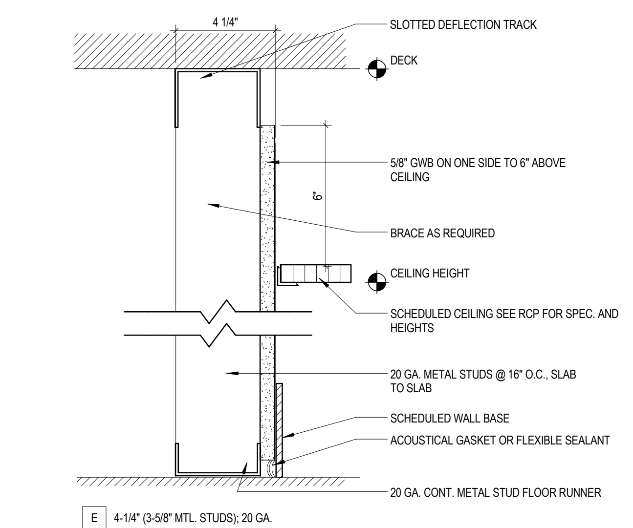
E PARTITION TYPE FURRED
