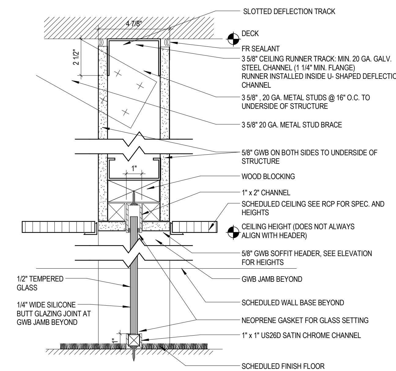
L GLASS PARTITION TYPE
