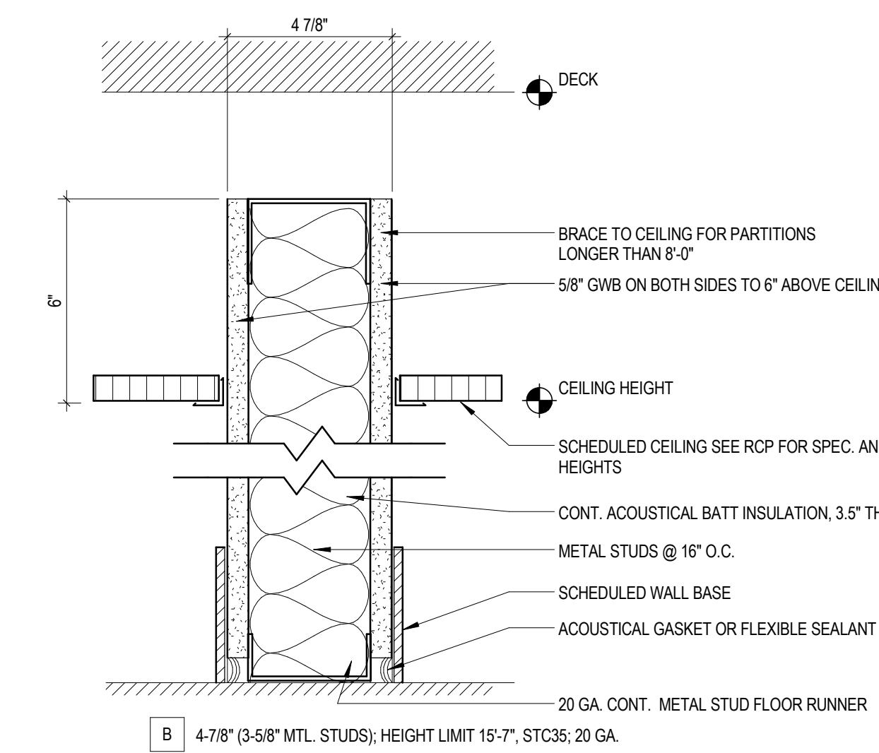
B PARTITION TYPE TO 6" ABOVE CEILING
