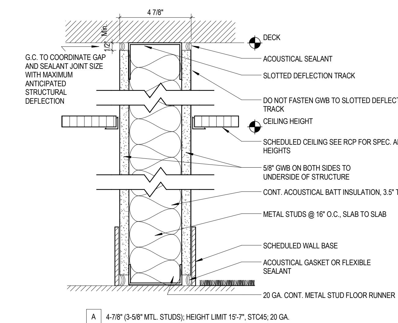
A PARTITION TYPE TO DECK
