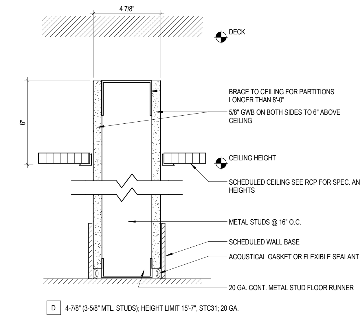
D PARTITION TYPE NON-INSULATED 6" ABOVE CEILING
