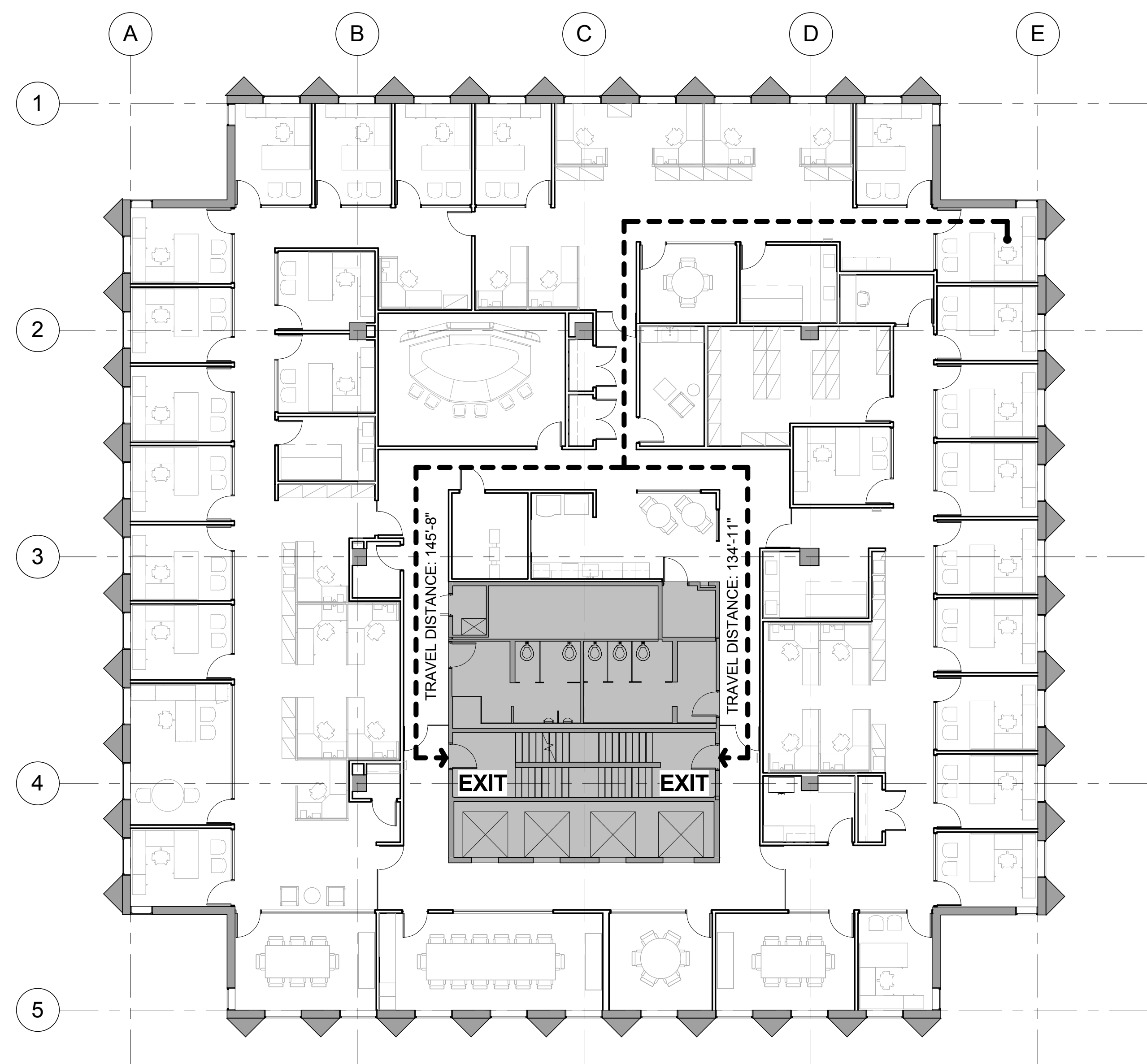
1 9th FLOOR LIFE SAFETY 3/32" = 1'-0"
