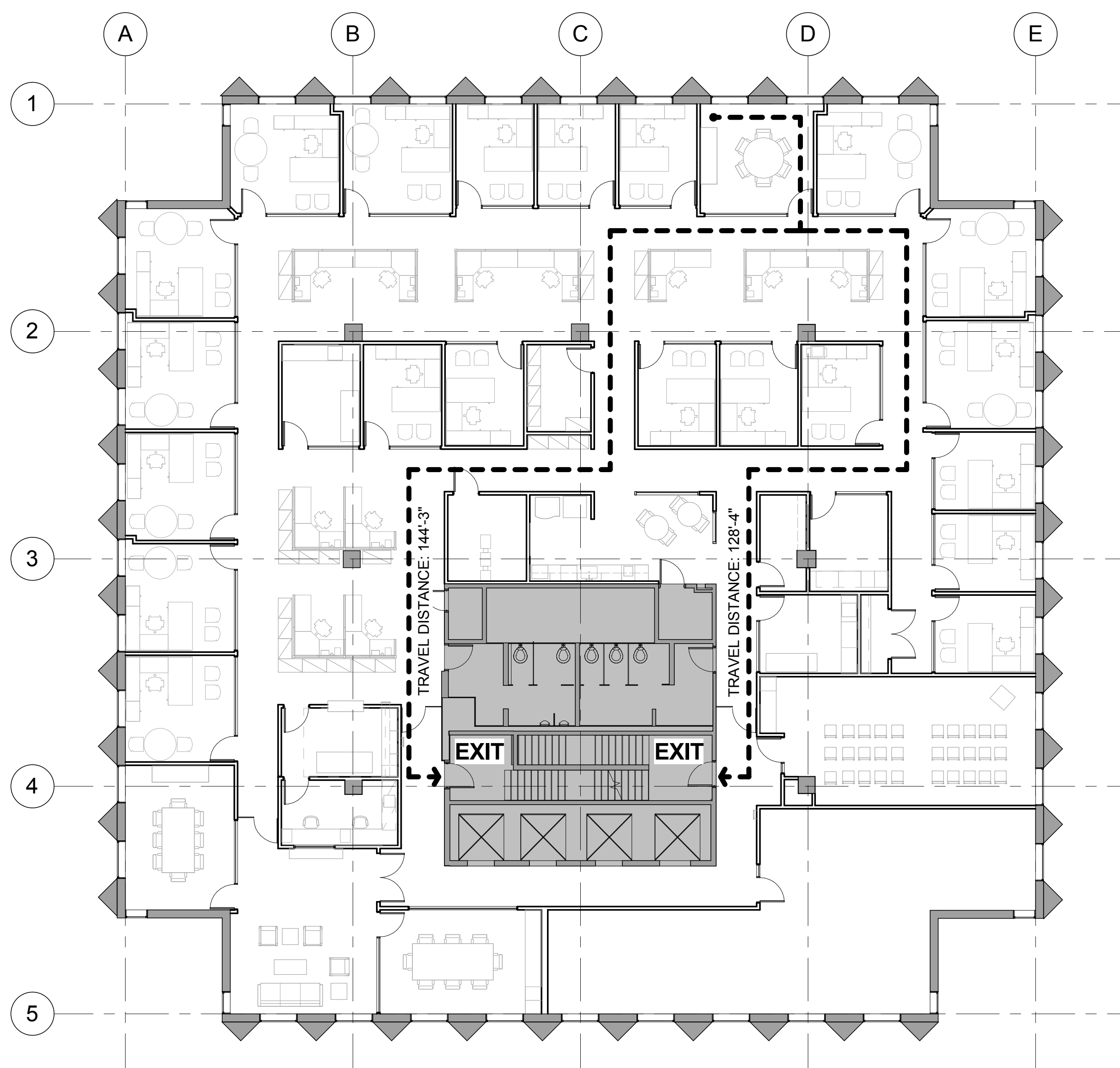
2 10th FLOOR LIFE SAFETY 3/32" = 1'-0"
