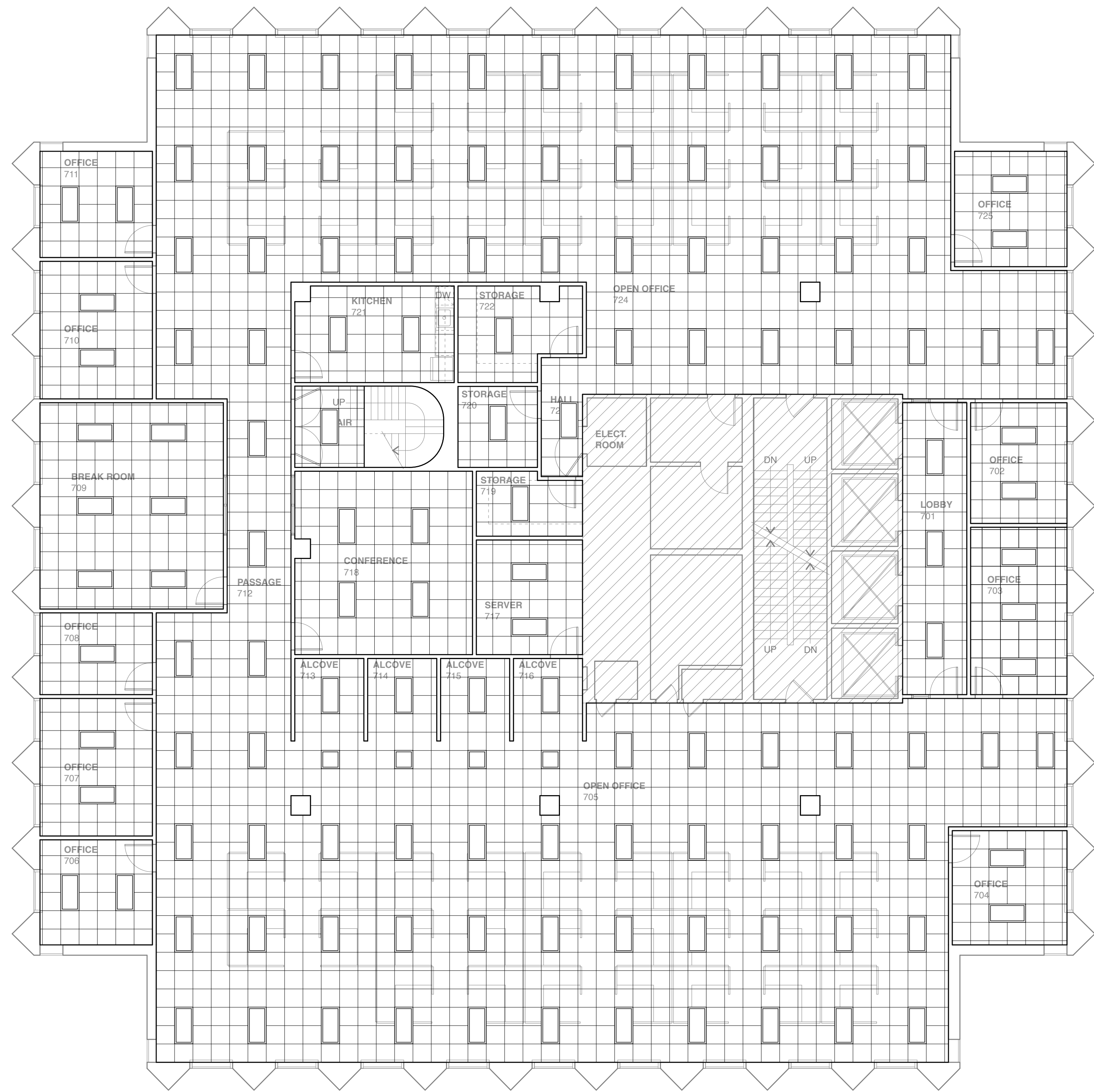
1 7TH FLOOR REFLECTED CEILING PLAN SCALE: 1/8" = 1'-0" 2' 4' 8' 16' AREA N.I.C.
