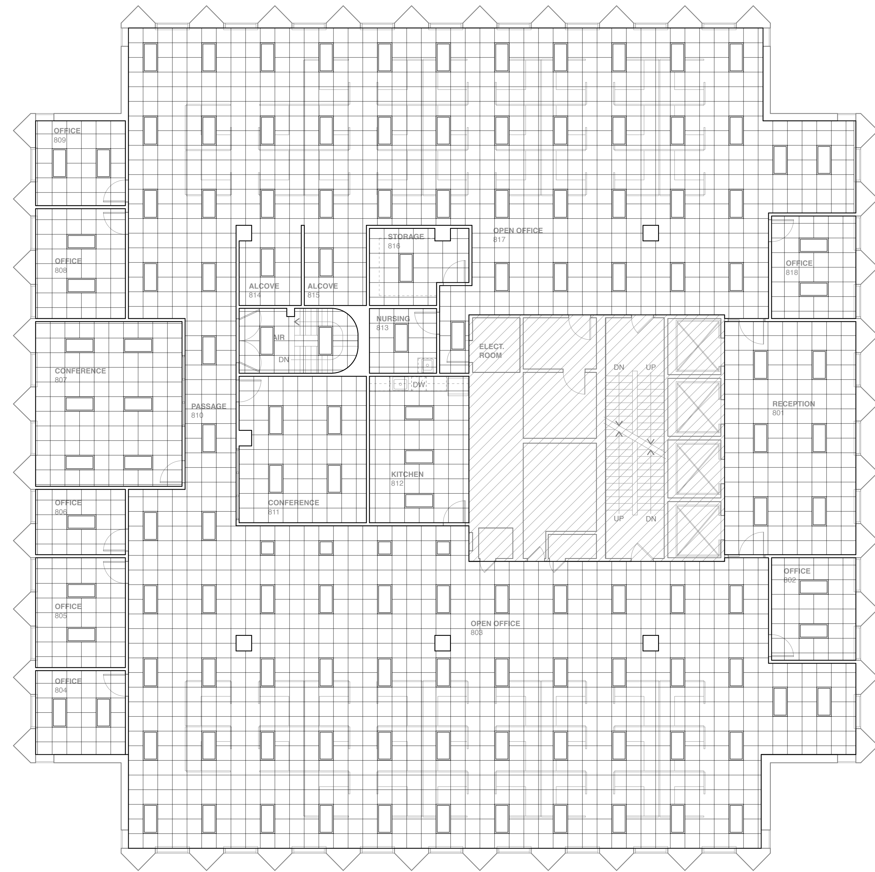
1 8TH FLOOR REFLECTED CEILING PLAN SCALE: 1/8" = 1'-0" 2' 4' 8' 16' AREA N.I.C.
