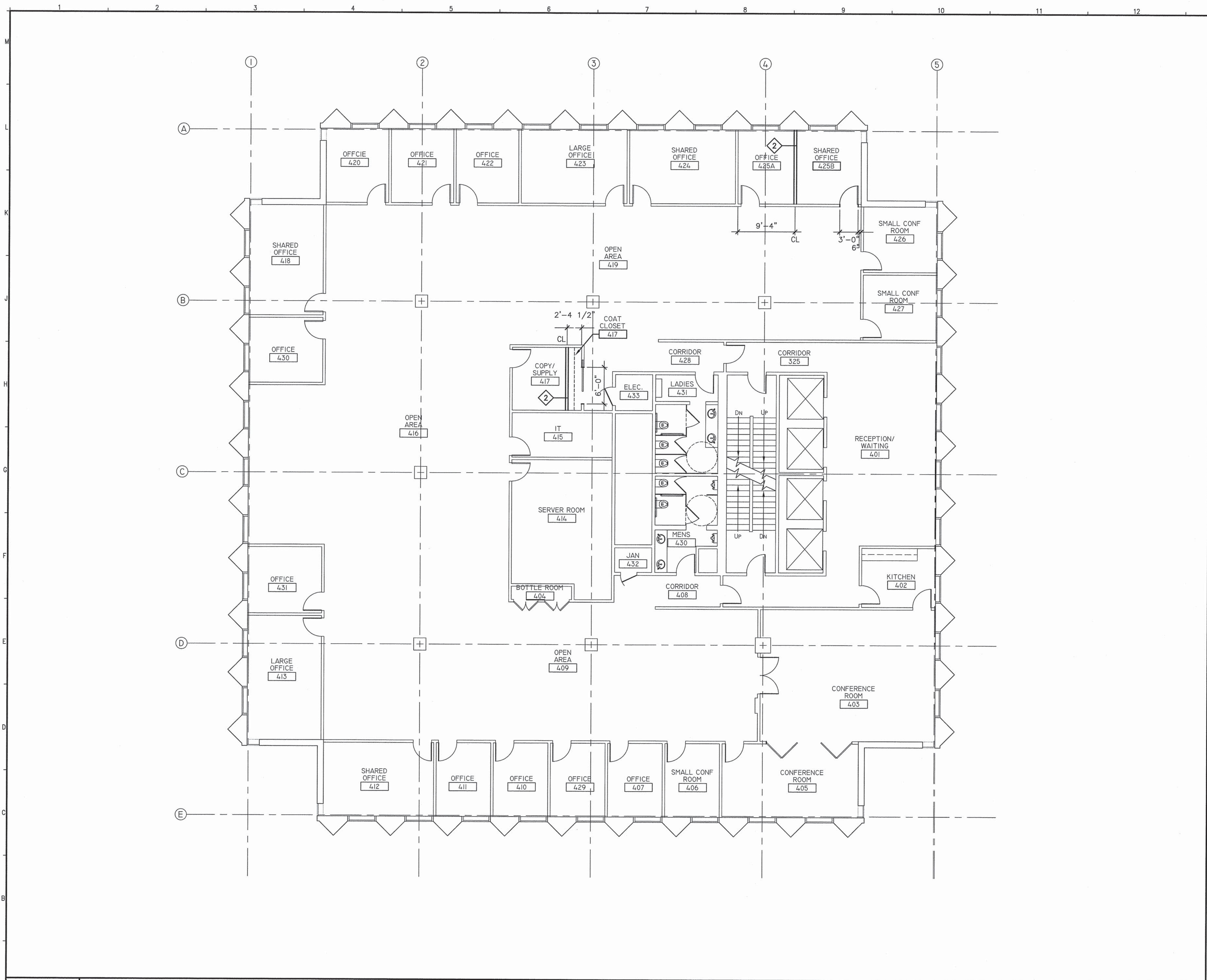
A1 FOURTH FLOOR PLAN 1/8"=1'-0"
