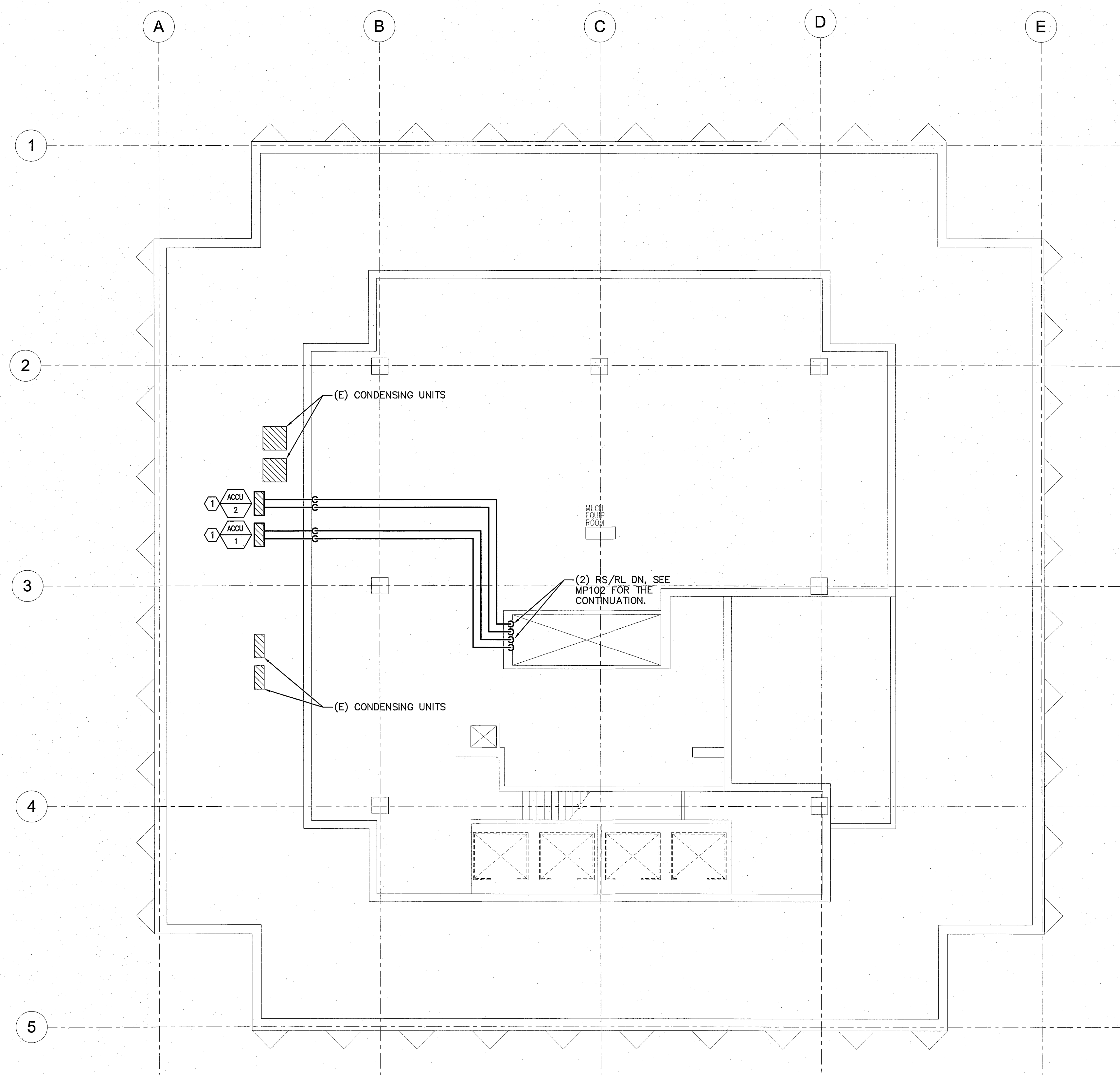
1 PENTHOUSE AND ROOF FLOOR PLAN 1/8" = 1'-0"
