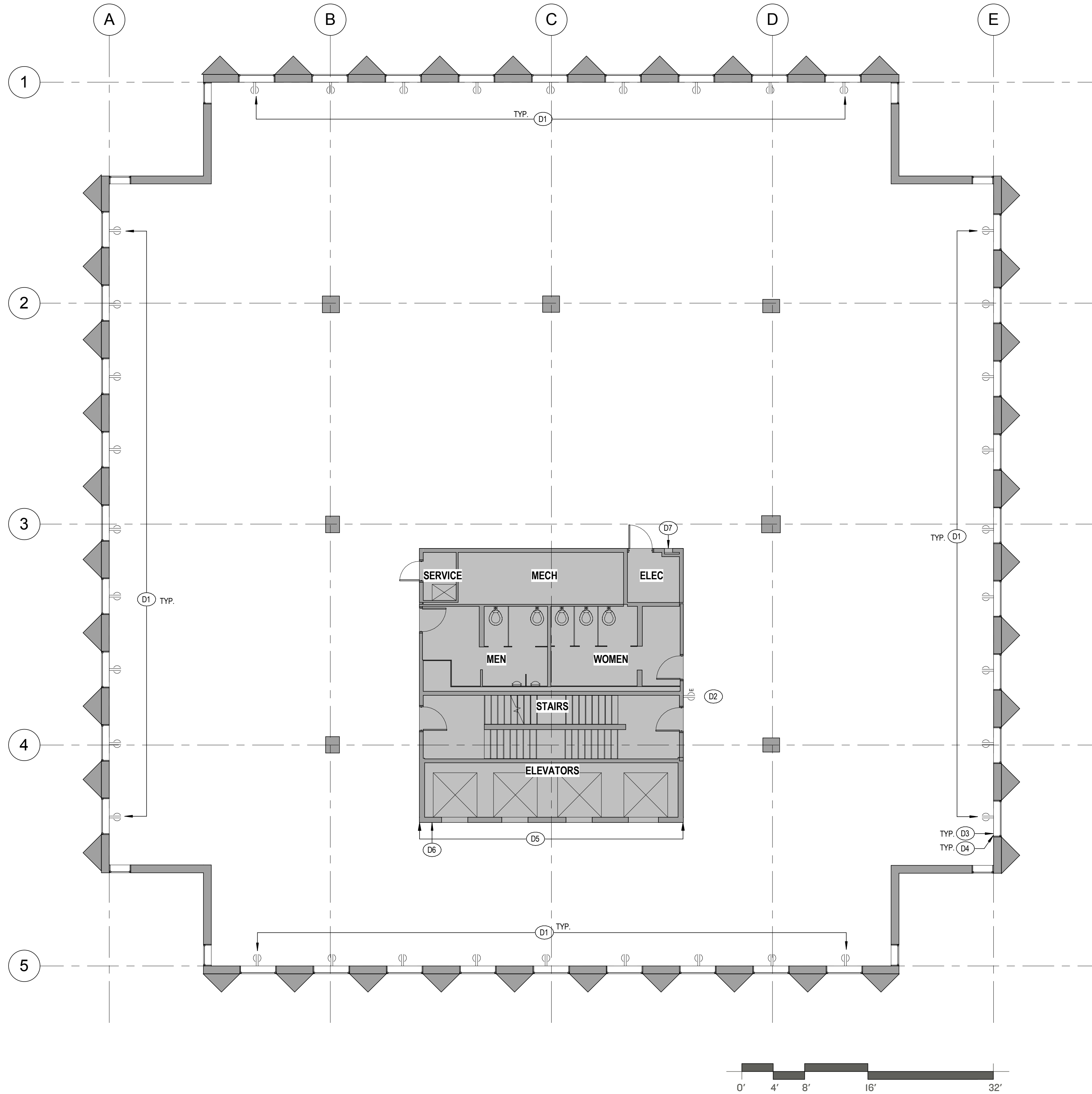
1 9th FLOOR DEMOLITION PLAN 1/8" = 1'-0"
