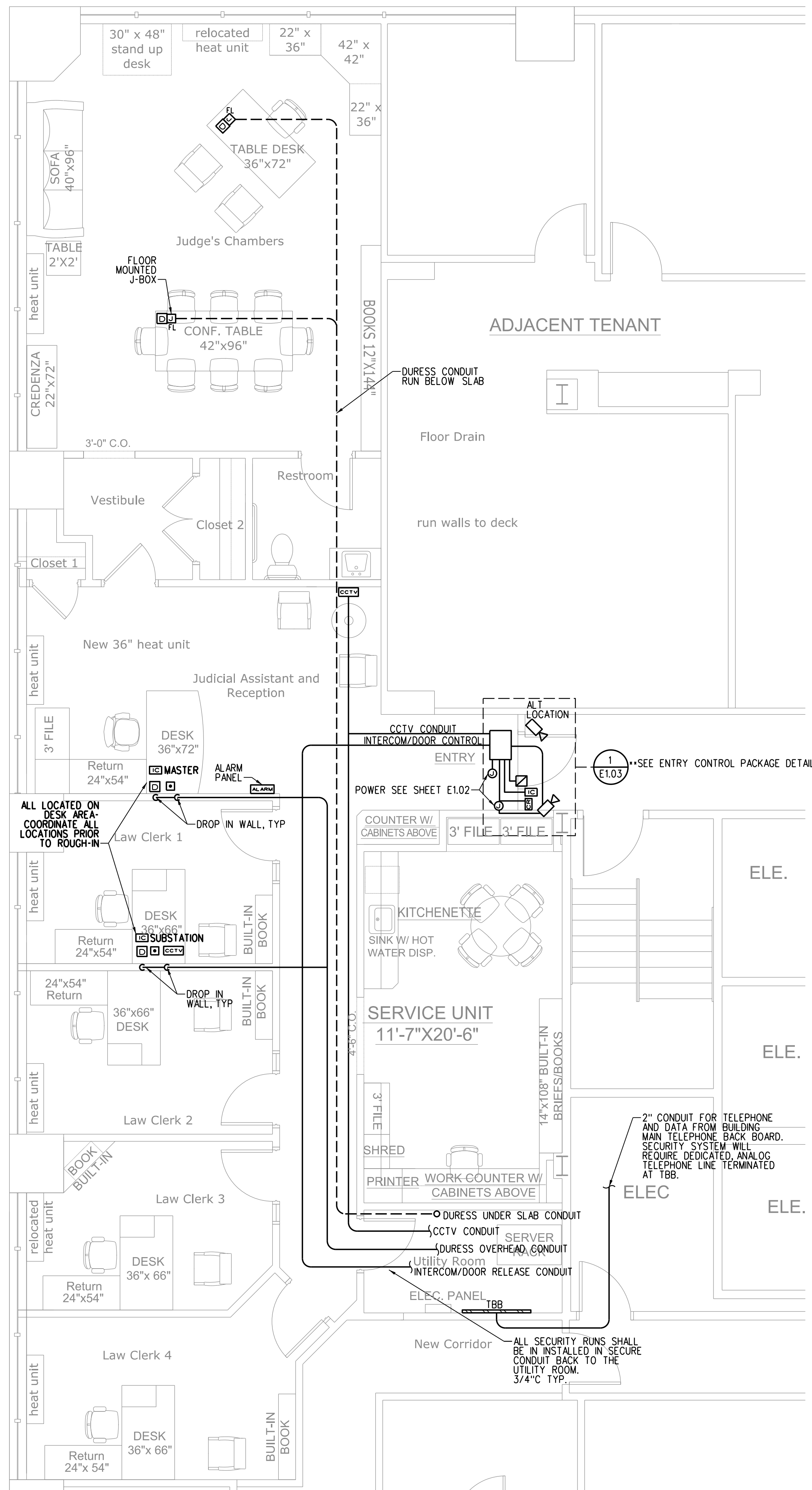
1 | SIXTH FLOOR SECURITY PLAN SCALE: 1/4"=1'-0"
