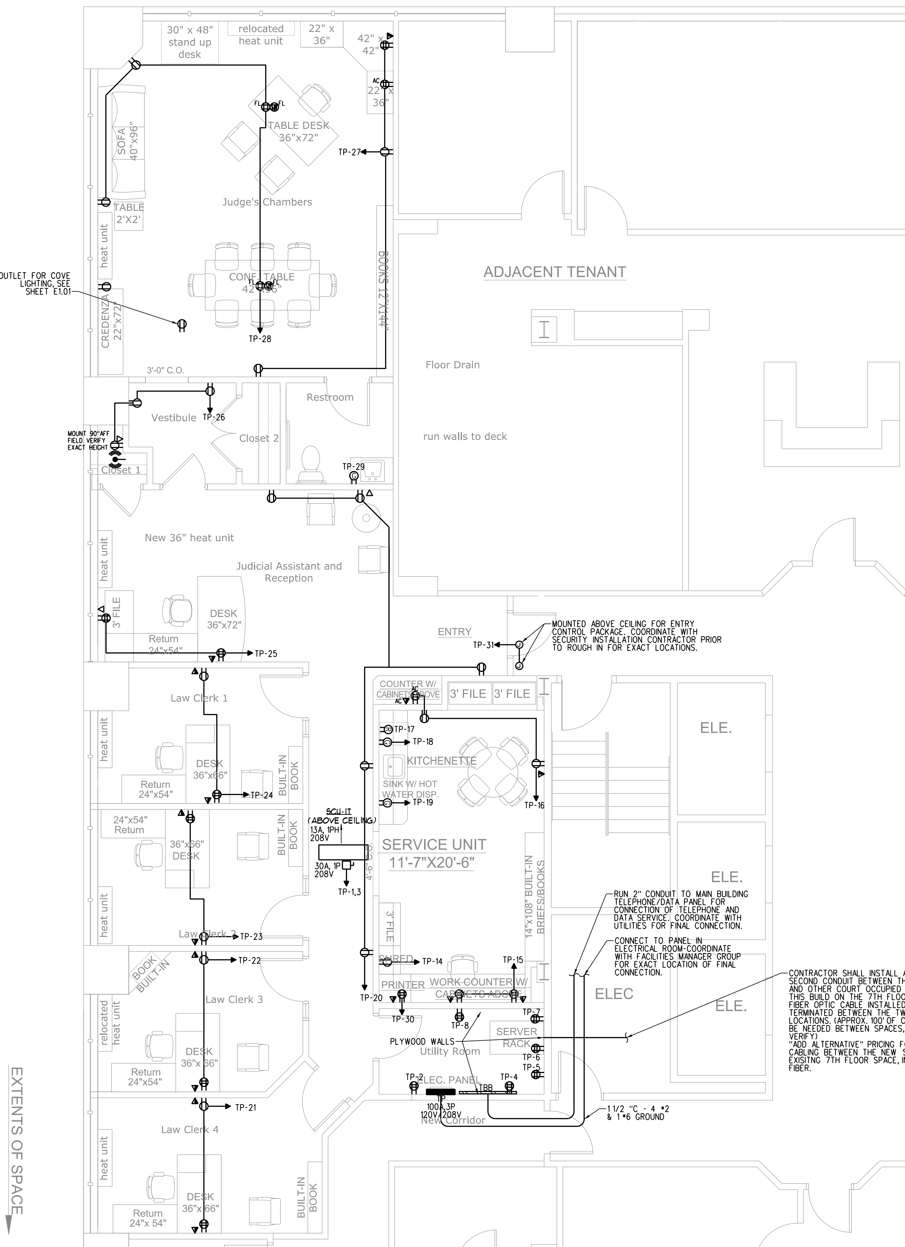
1 SIXTH FLOOR POWER PLAN SCALE: 1/4"=1'-0"
