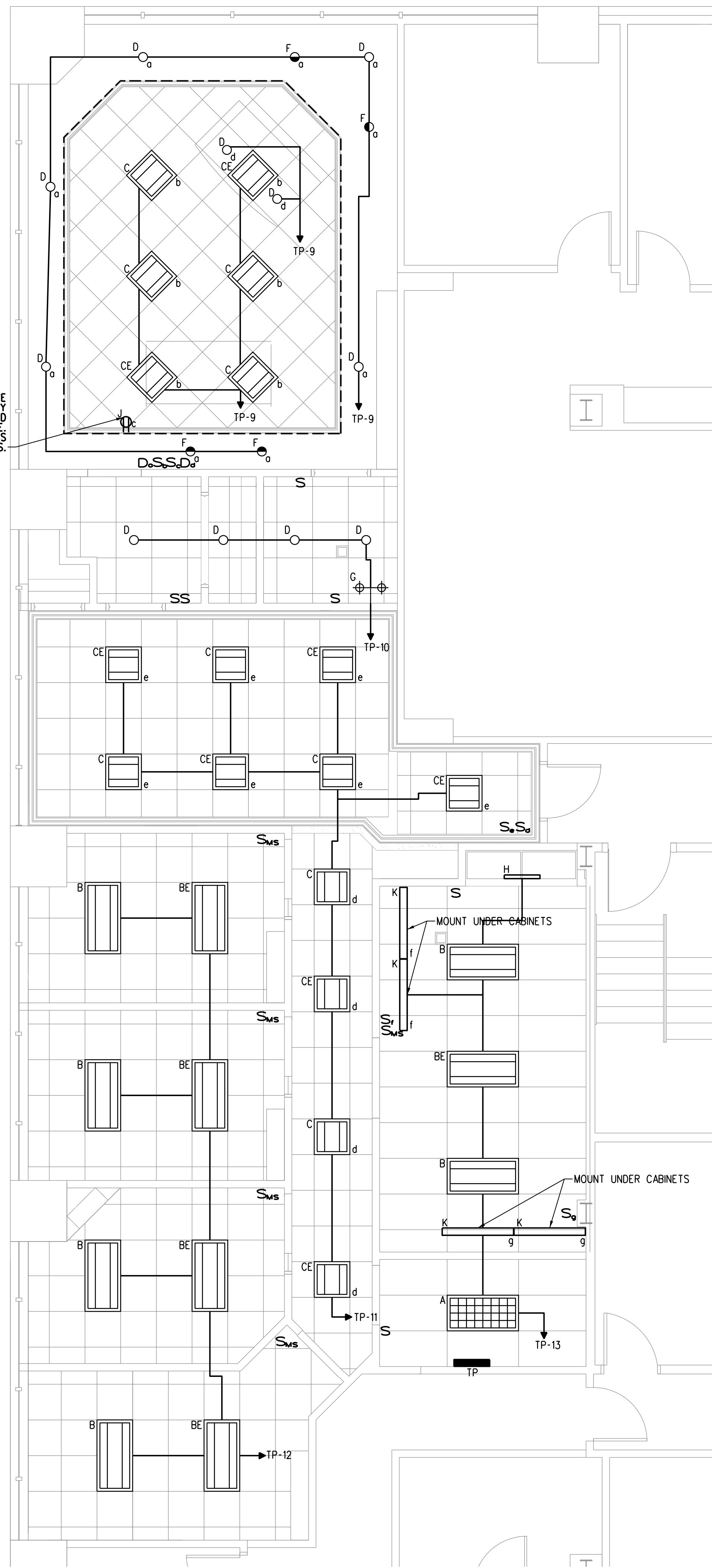
1 | SIXTH FLOOR LIGHTING PLAN SCALE: 1/4"=1'-0"
