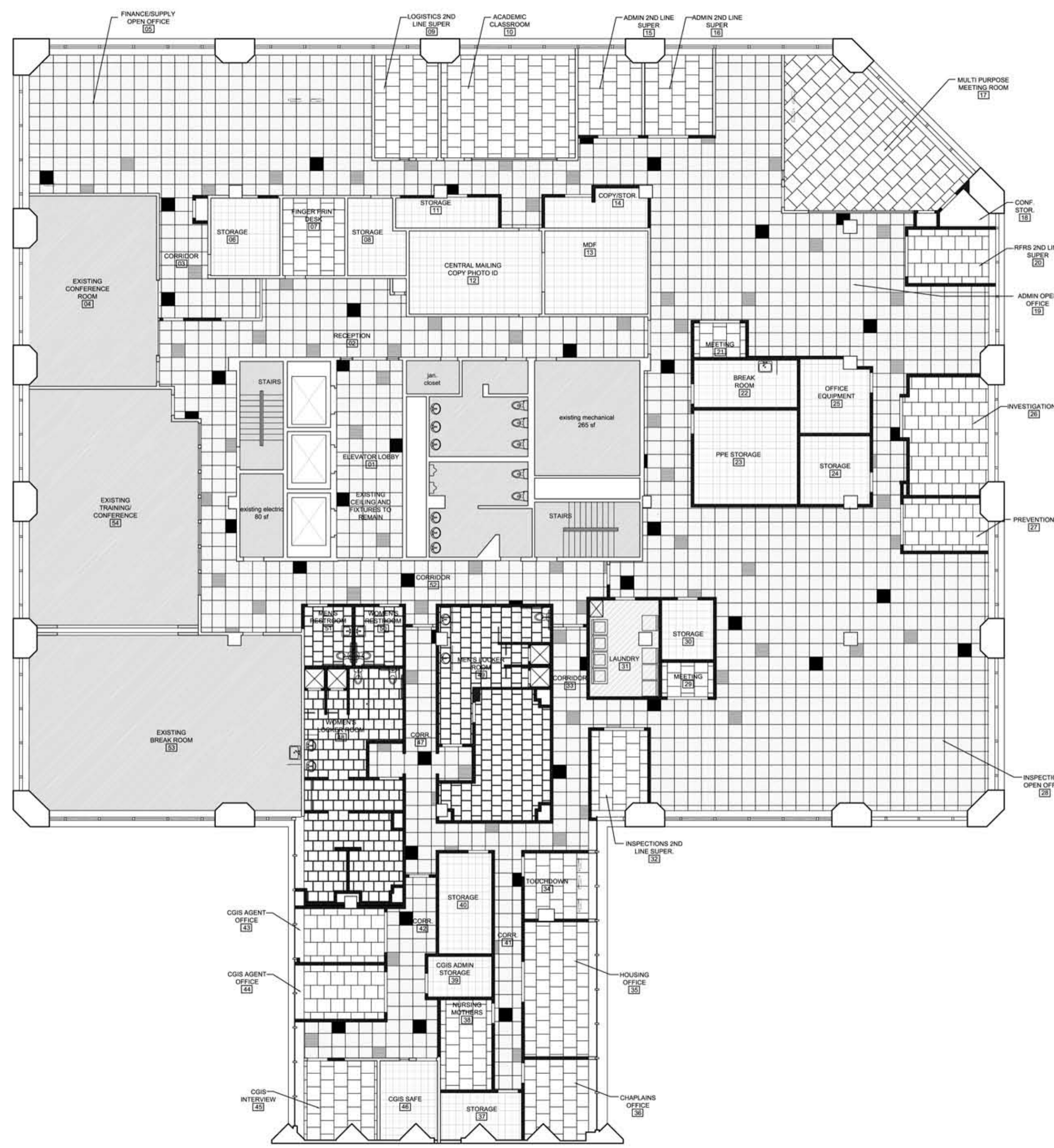
1 REFLECTED CEILING PLAN SCALE: 1/8"=1'-0"
