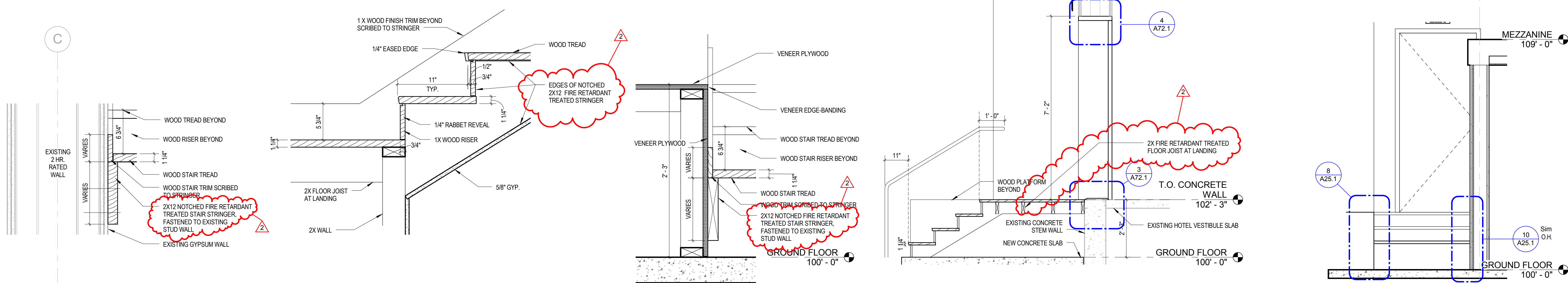
10 Stair Section A 1 1/2" = 1'-0" 9 STAIR SECTION B 1 1/2" = 1'-0" 8 STAIR SECTION C 1 1/2" = 1'-0" 7 STAIR SECTION 1 1/2" = 1'-0" 6 STAIR SECTION 2 1/2" = 1'-0"
