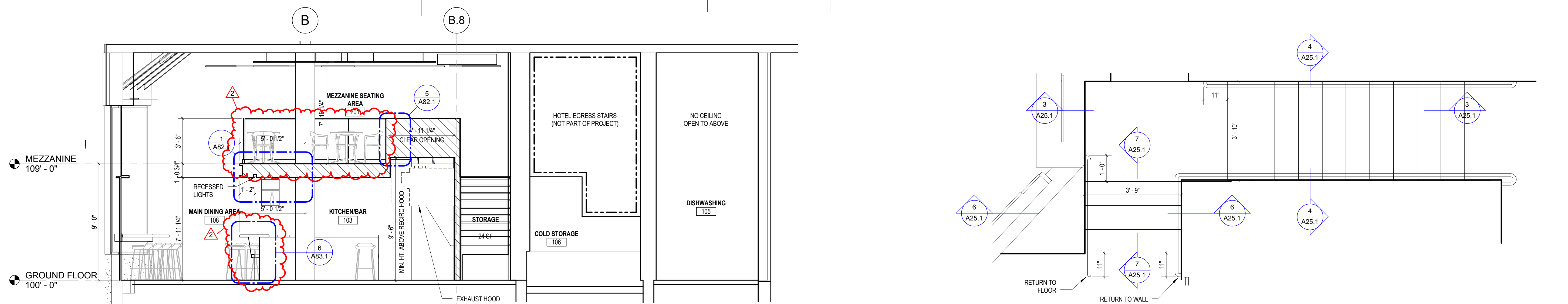
2 SECTION THROUGH CORRIDOR 1/4" = 1'-0" 1 STAIR PLAN 1/2" = 1'-0"
