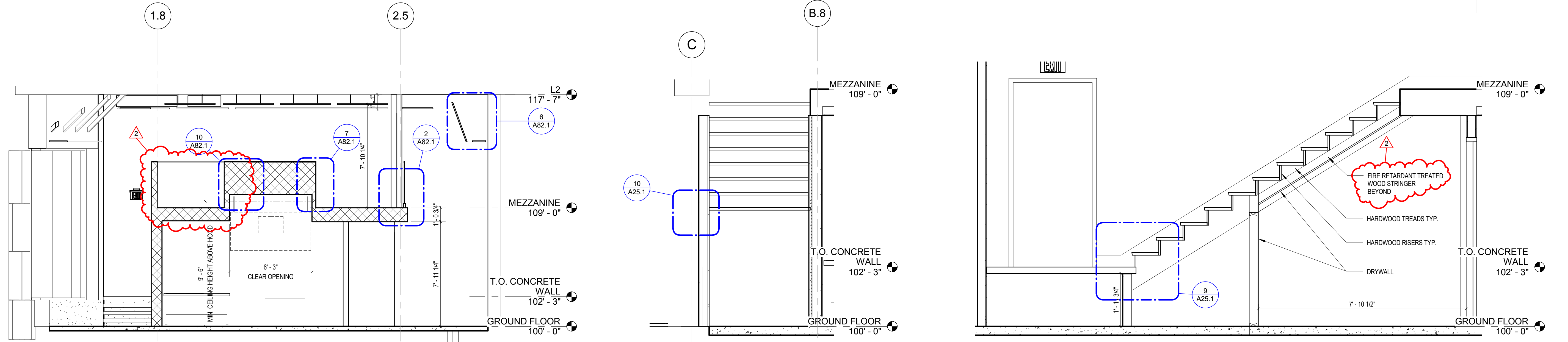
5 SECTION THROUGH KITCHEN 1/4" = 1'-0" 4 STAIR SECTION 4 1/2" = 1'-0" 3 STAIR SECTION 3 1/2" = 1'-0"
