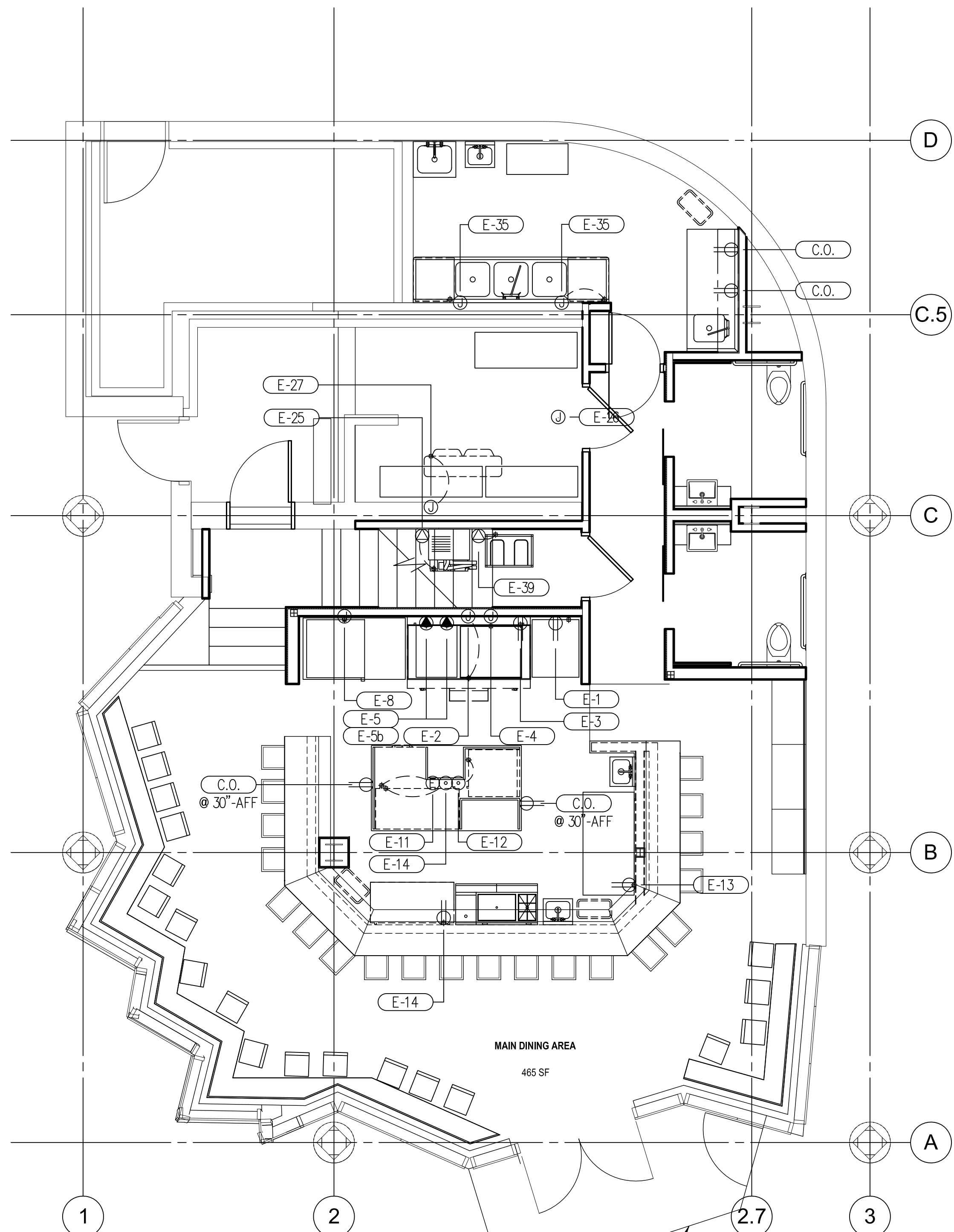
First Floor Foodservice Equipment Plan SCALE - 1/4" = 1' - 0"
