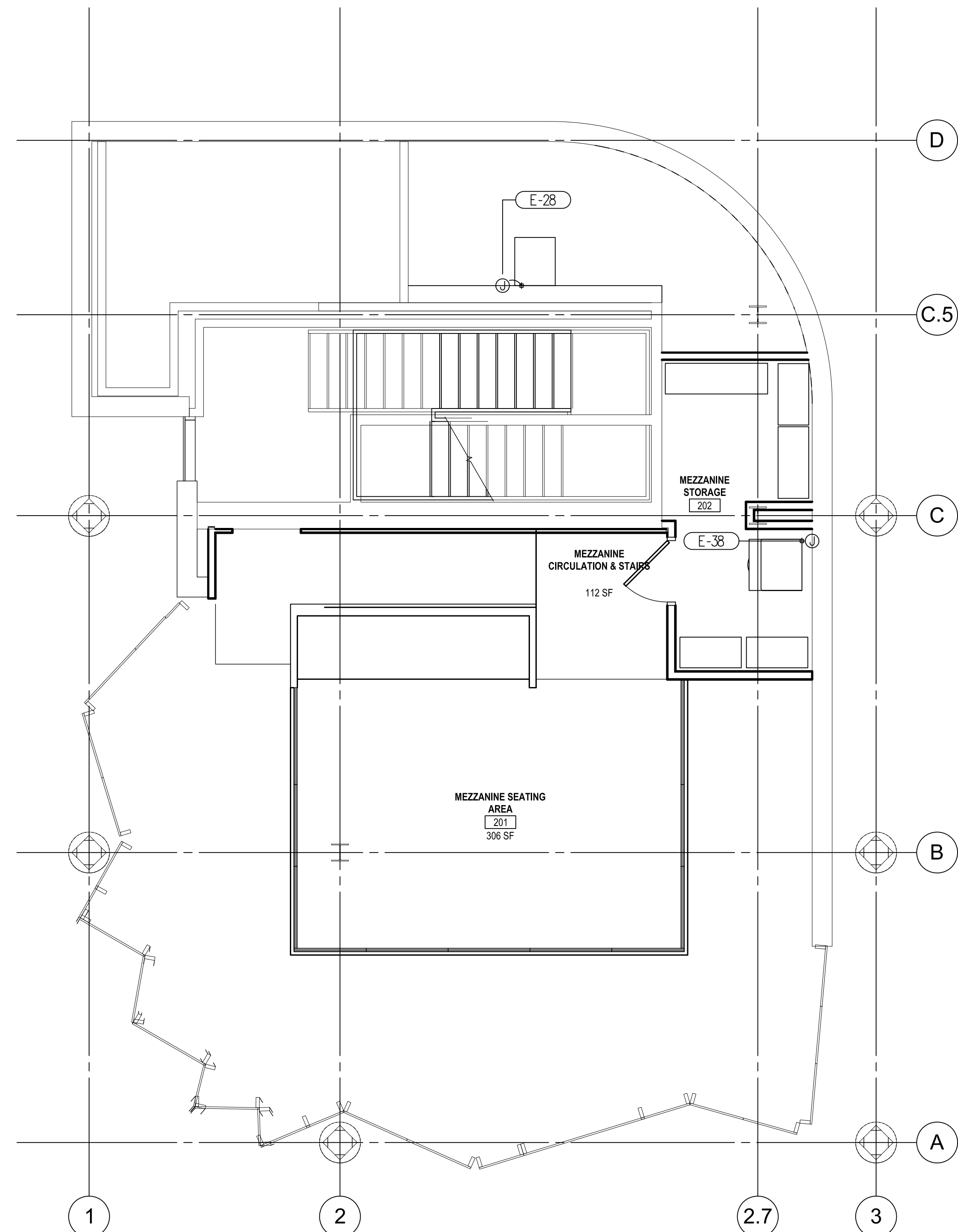
Mezzanine Foodservice Equipment Plan SCALE - 1/4" = 1' - 0"
