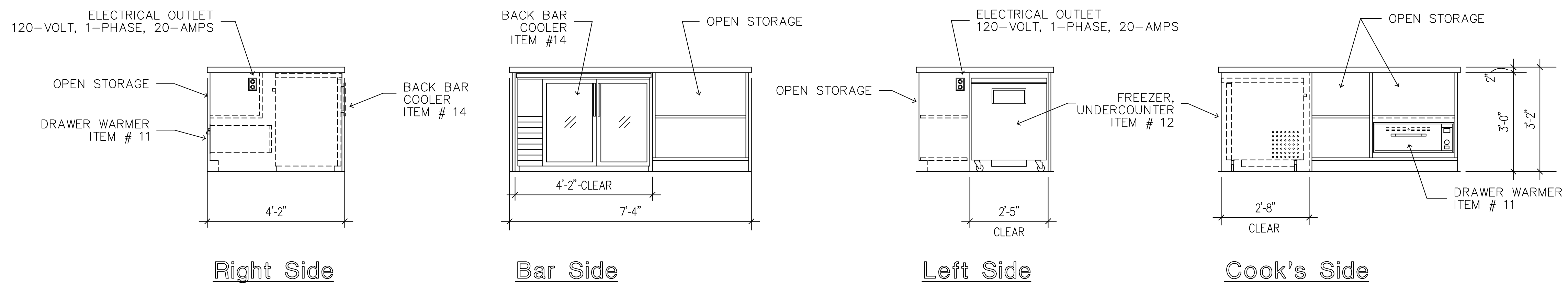
Chef's Island Work Counter Elevations SCALE - 1/2" = 1' - 0"
