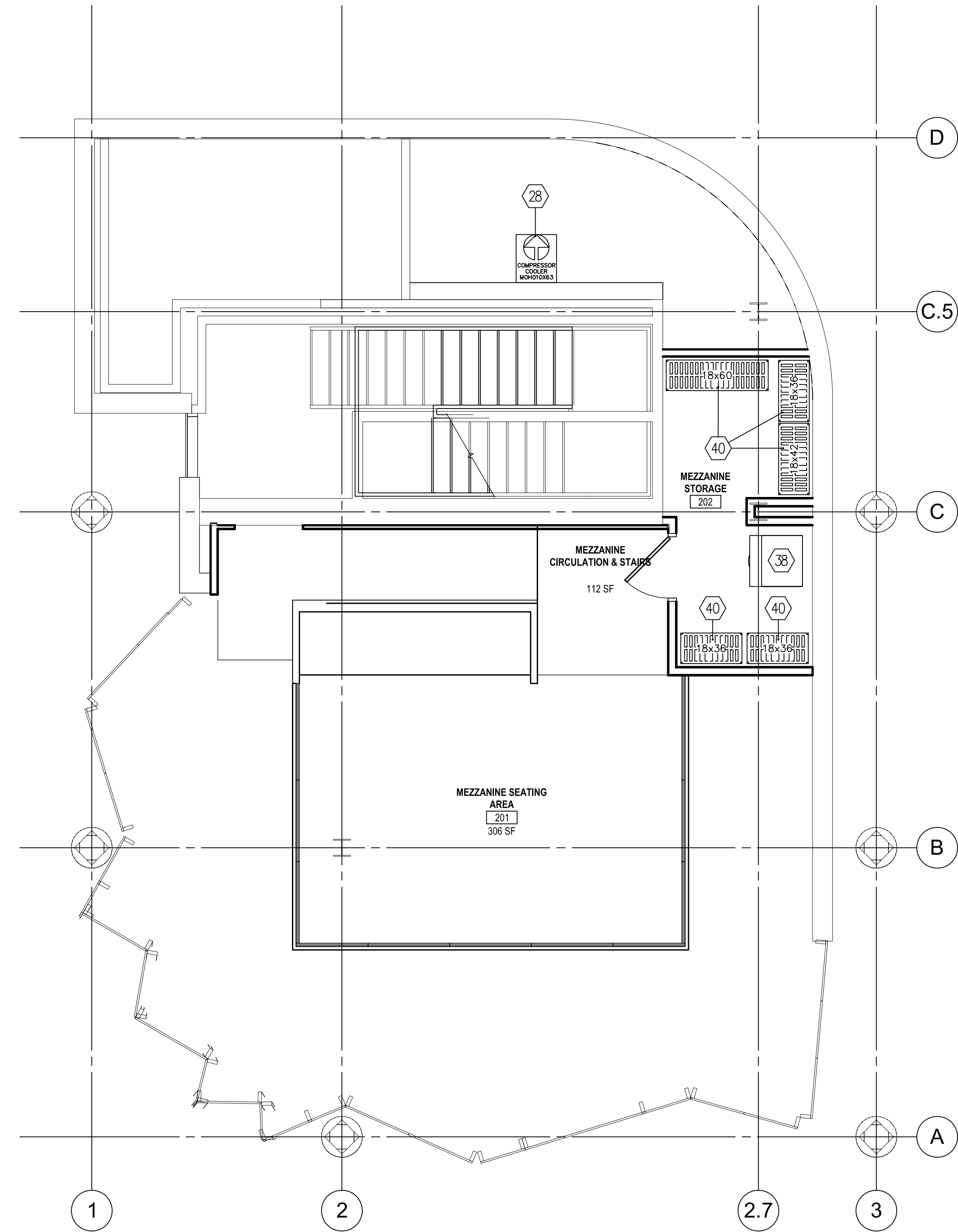
Mezzanine Foodservice Equipment Plan SCALE - 1/4" = 1' - 0"
