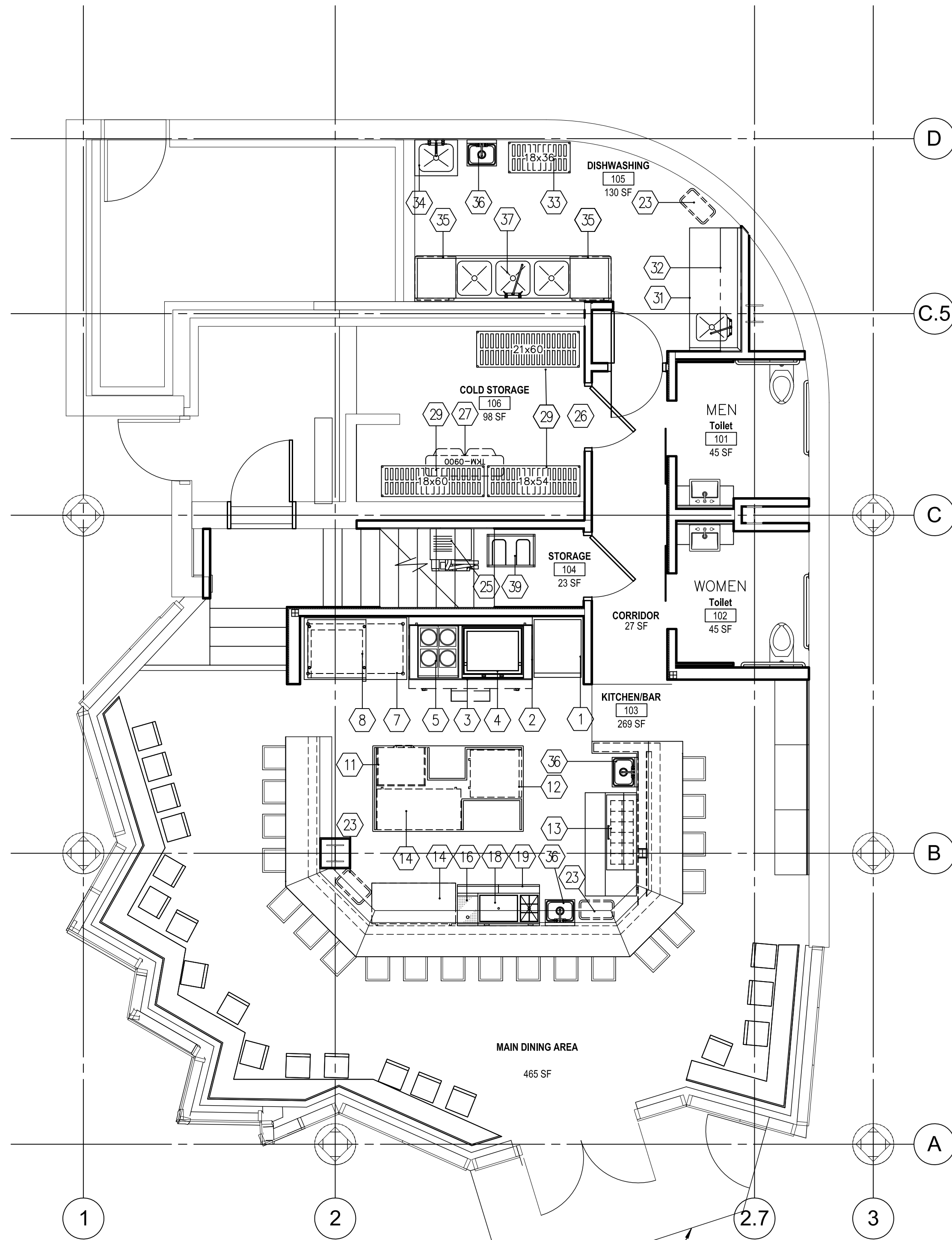
First Floor Foodservice Equipment Plan SCALE - 1/4" = 1' - 0"
