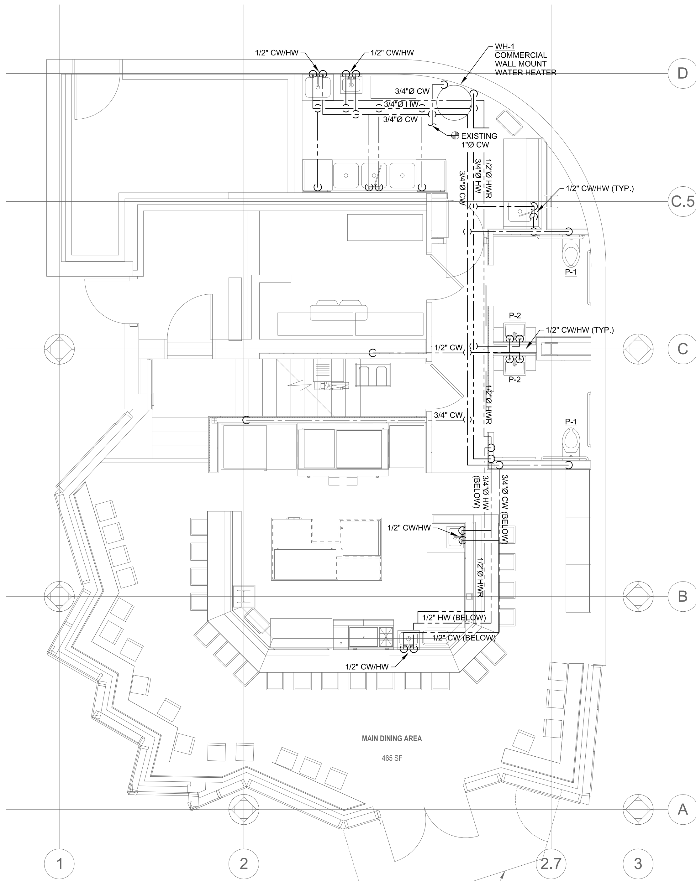
1 LOWER LEVEL - DOMESTIC PLUMBING LAYOUT SCALE: 1/4" = 1'-0"
