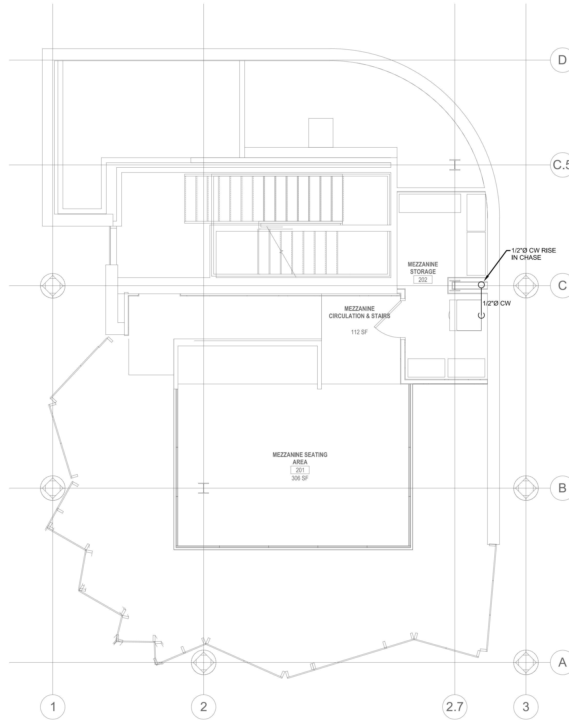
2 MEZZANINE - DOMESTIC PLUMBING LAYOUT SCALE: 1/4" = 1'-0"
