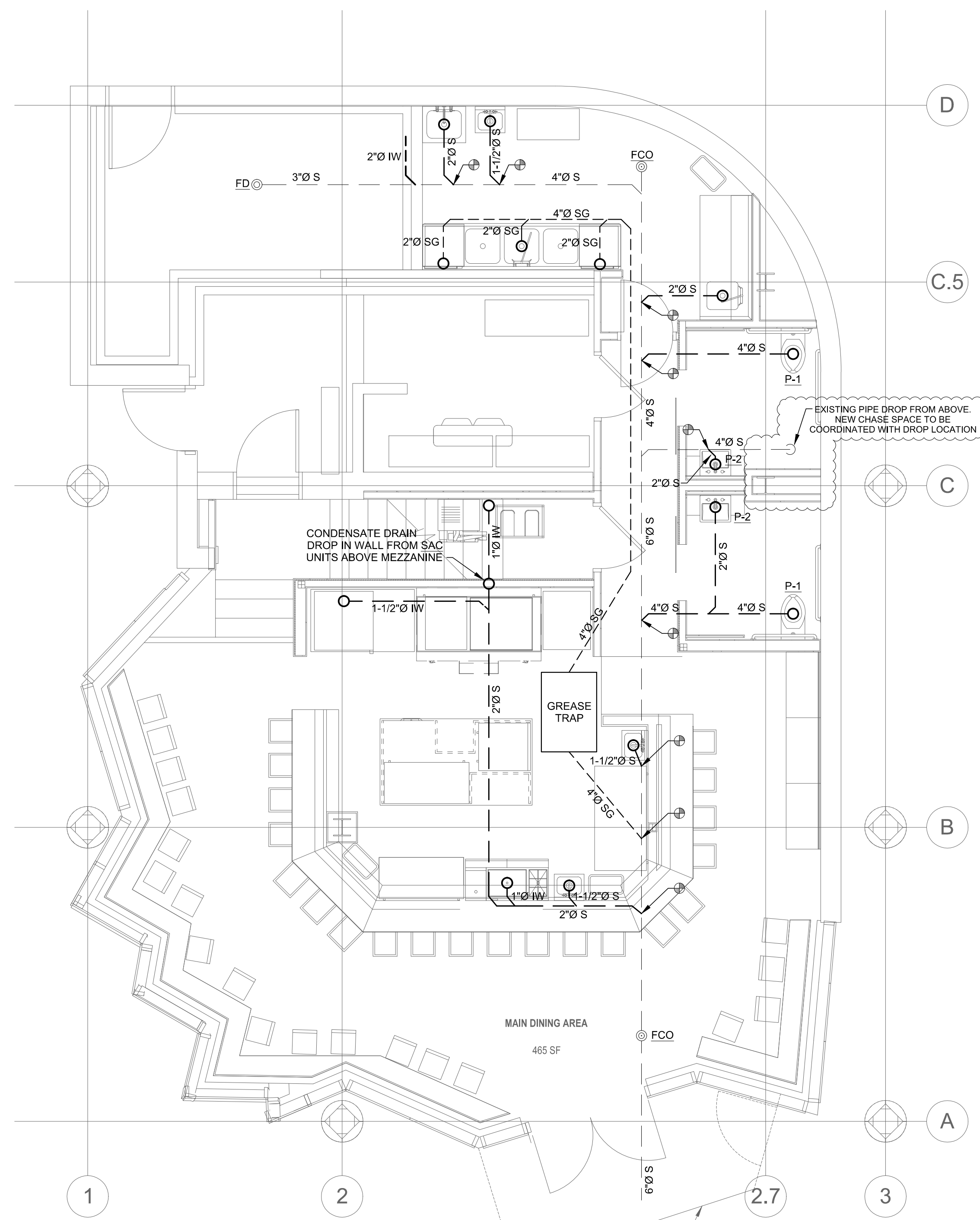
1 LOWER LEVEL - PLUMBING DRAINAGE LAYOUT SCALE: 1/4" = 1'-0"
