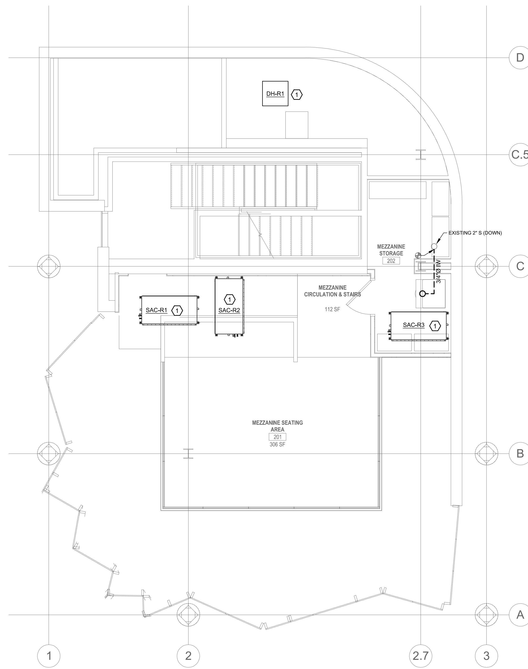
2 MEZZANINE - PLUMBING DRAINAGE LAYOUT SCALE: 1/4" = 1'-0"
