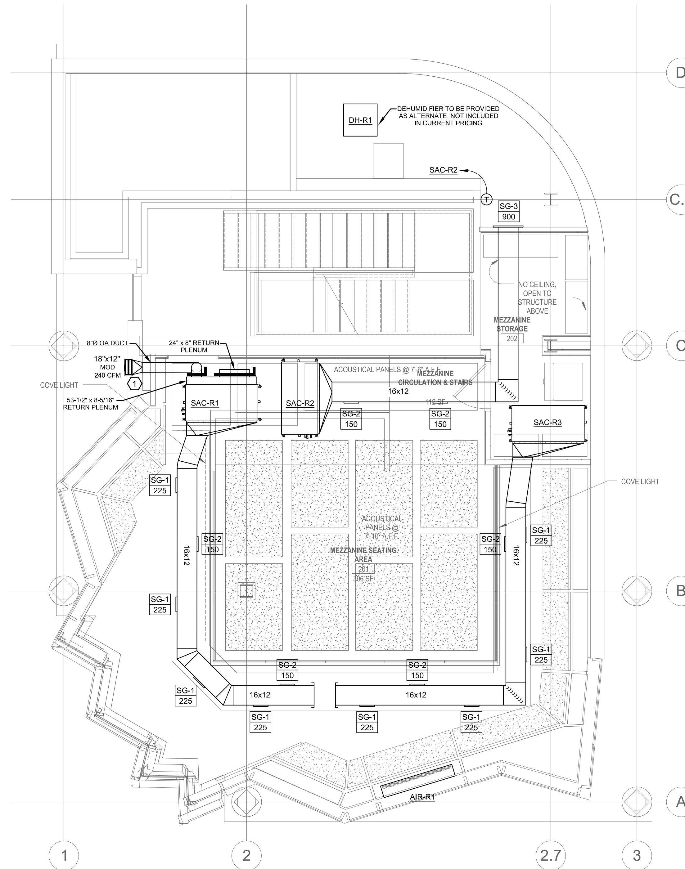
1 MEZZANINE - HVAC EQUIPMENT & DUCTWORK LAYOUT SCALE: 1/4" = 1'-0"
