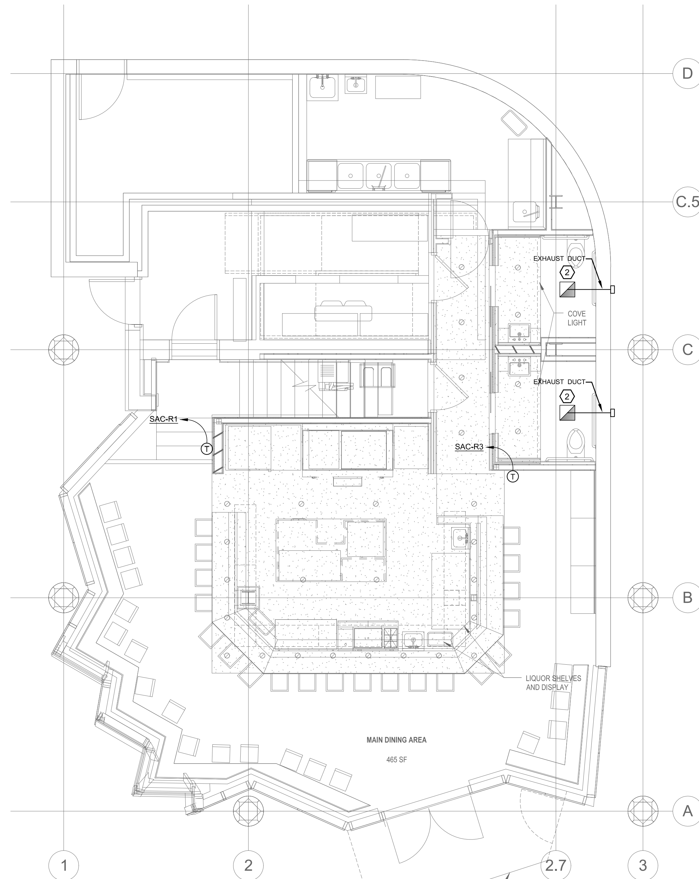
1 LOWER LEVEL - HVAC EQUIPMENT & DUCTWORK LAYOUT SCALE: 1/4" = 1'-0"
