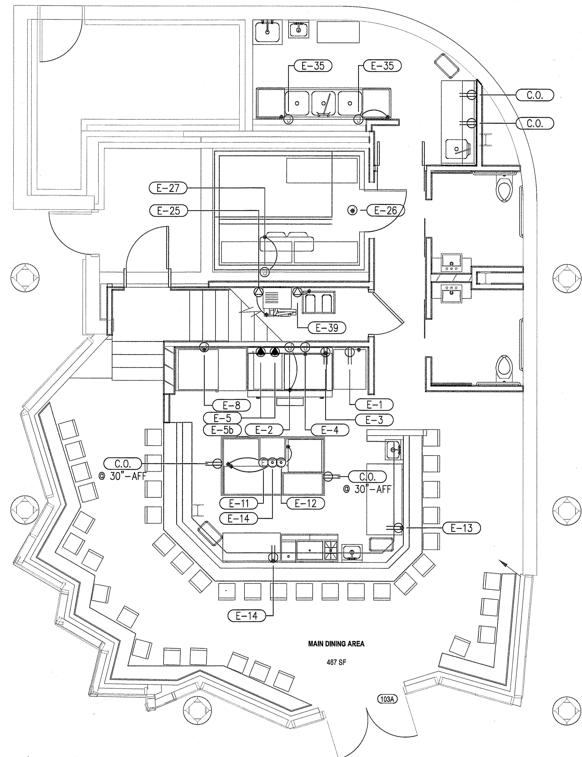
First Floor Foodservice Equipment Plan SCALE - 1/4" = 1' - 0"
