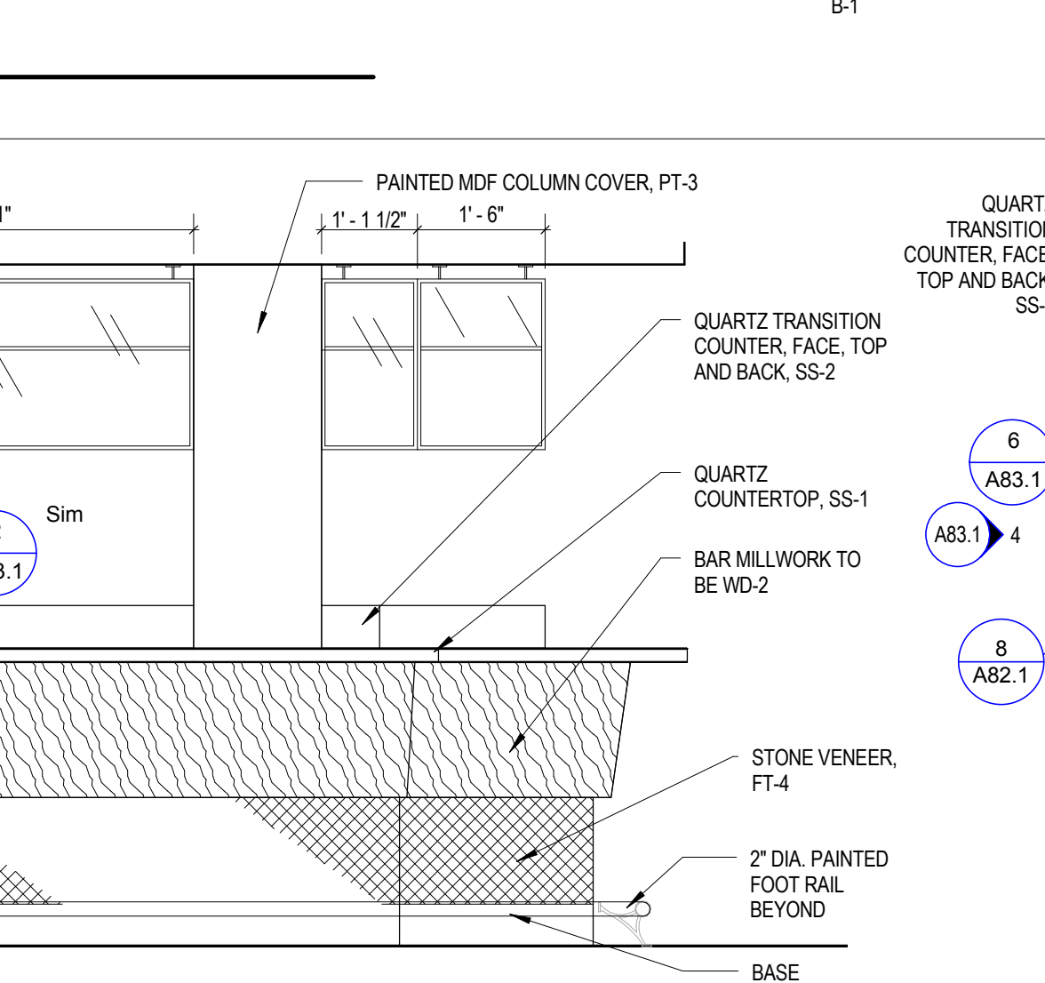
4 BAR ELEVATION EAST 1/2" = 1'-0"
