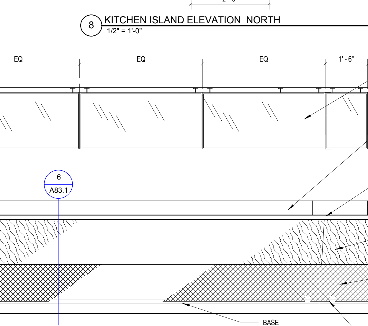
8 KITCHEN ISLAND ELEVATION NORTH 1/2" = 1'-0"
