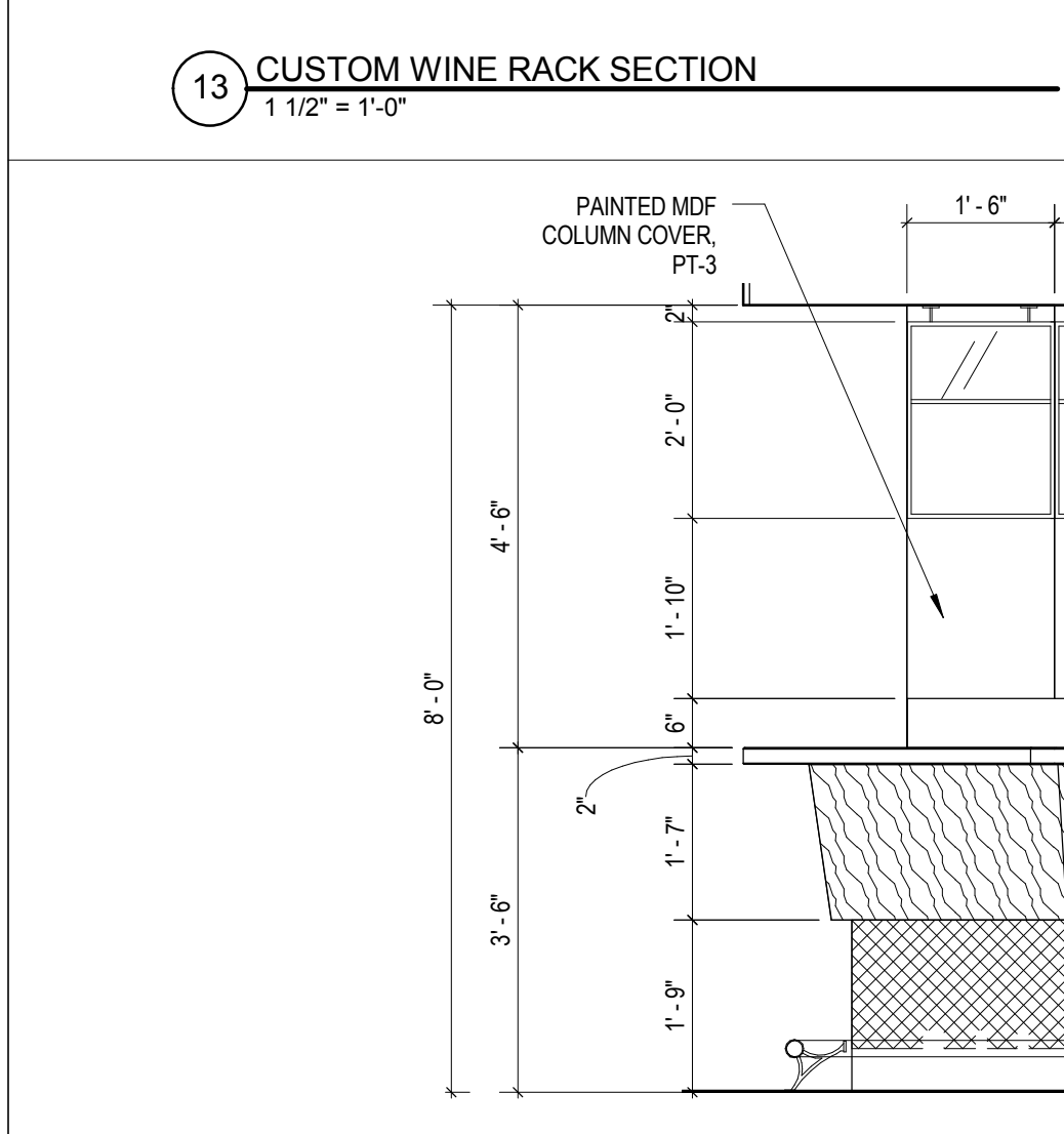
13 CUSTOM WINE RACK SECTION 1 1/2" = 1'-0"
