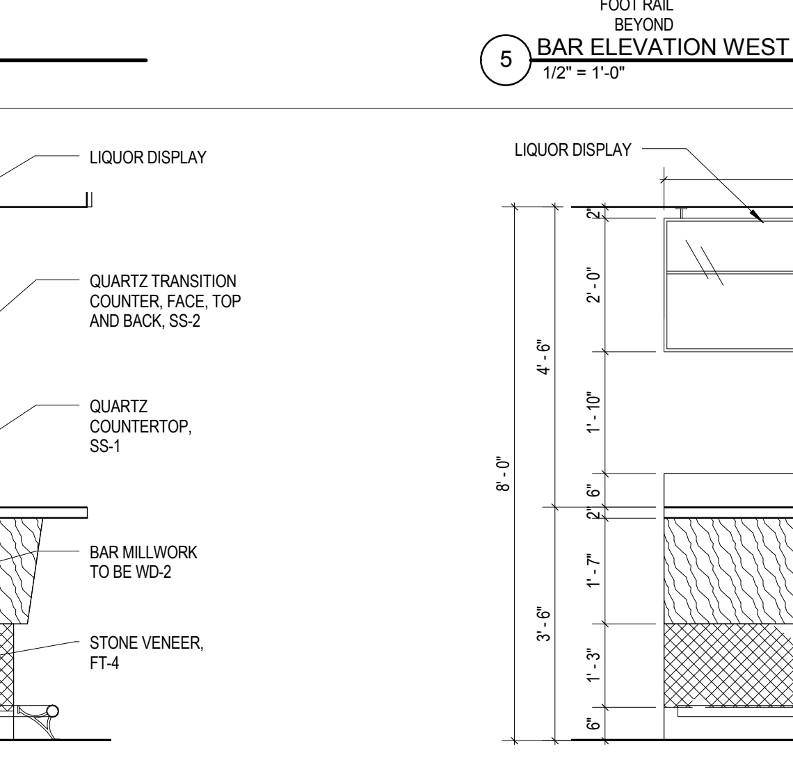
5 BAR ELEVATION WEST 1/2" = 1'-0"
