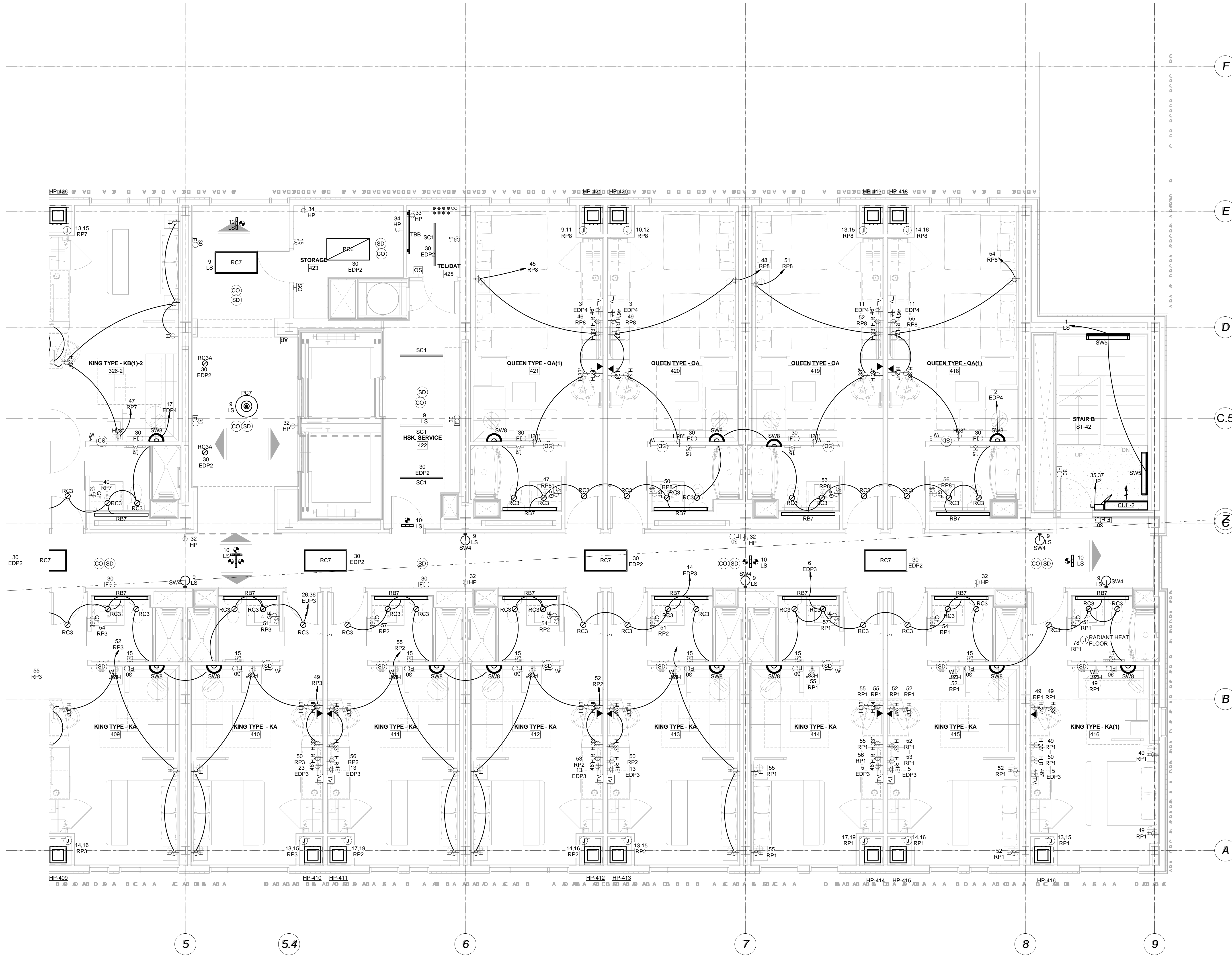
① Fourth Floor Electrical Plan-Part B 1/4" = 1'-0"
