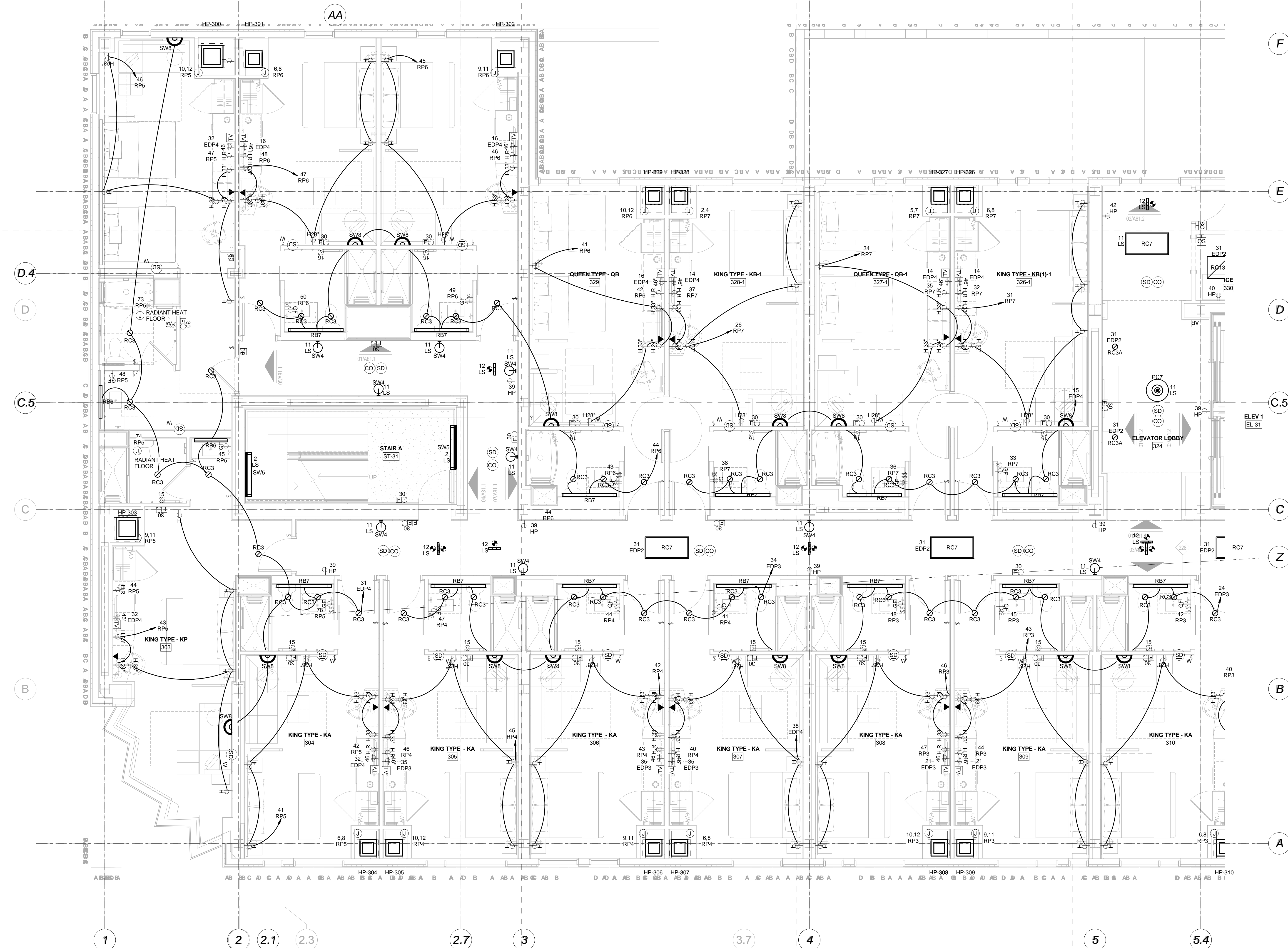
1 Third Floor Electrical Plan-Part A 1/4" = 1'-0"
