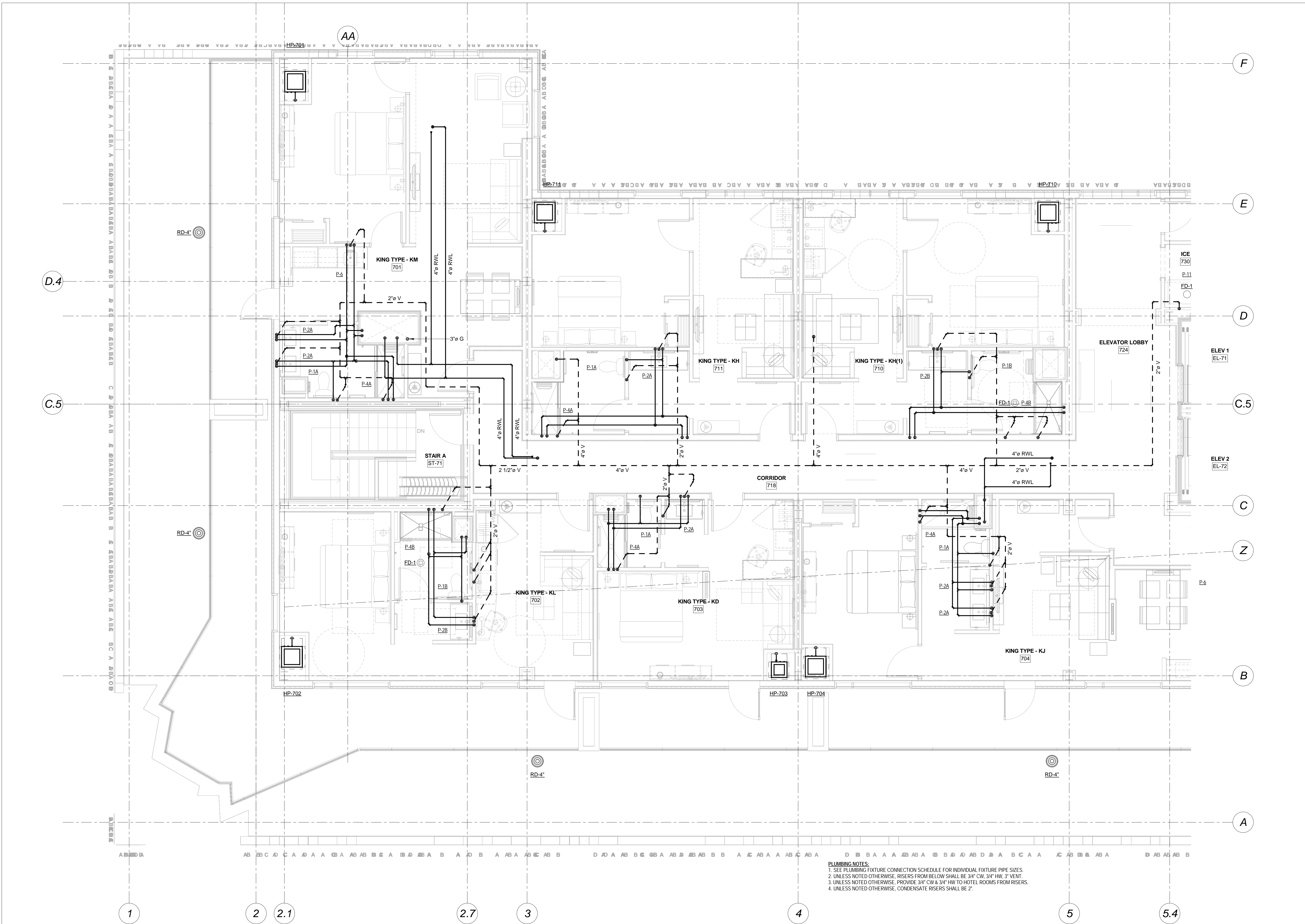
① Seventh Floor Plumbing Plan-Part A 1/4" = 1'-0"
