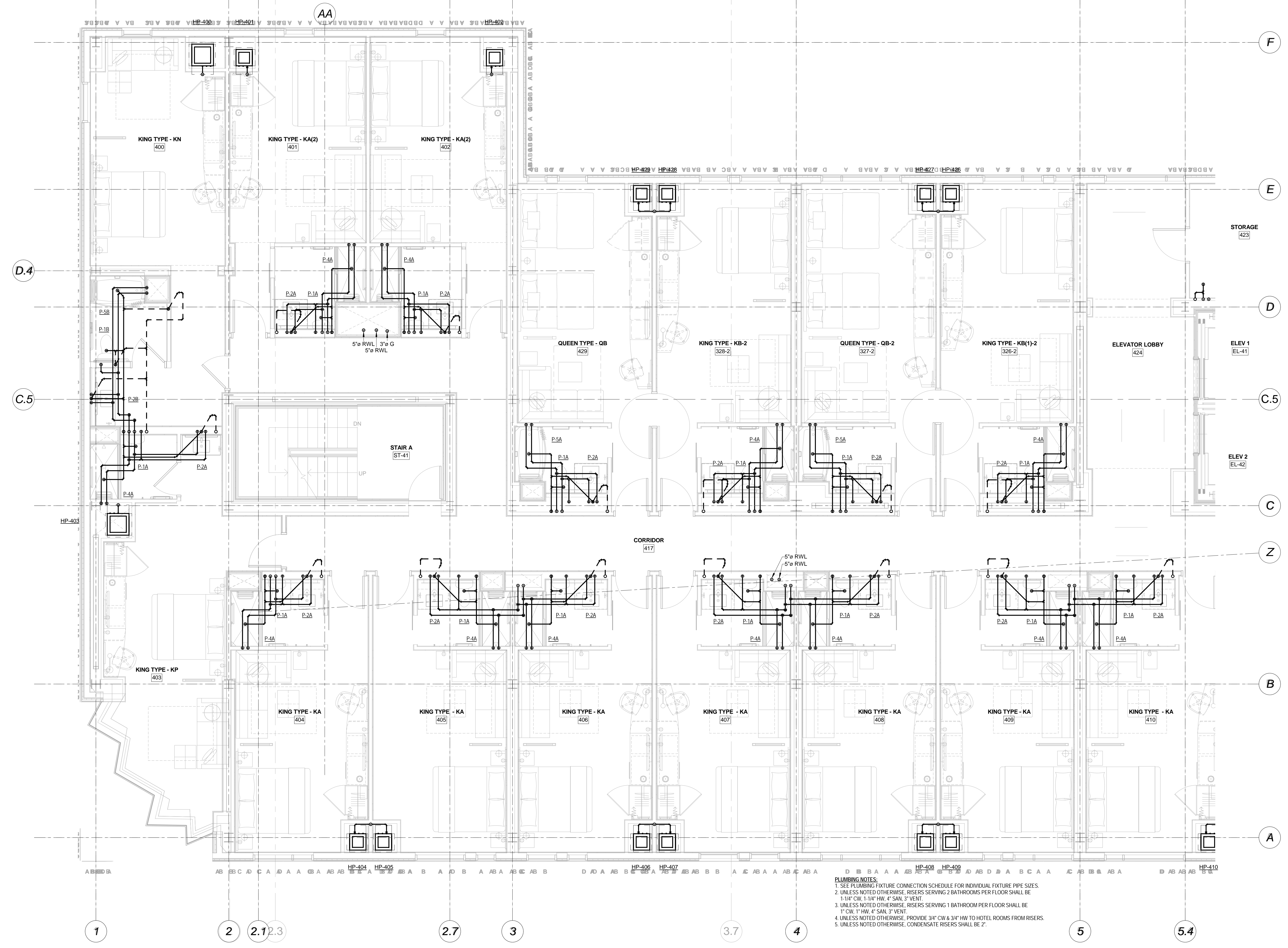
1 Fourth Floor Plumbing Plan-Part A 1/4" = 1'-0"
