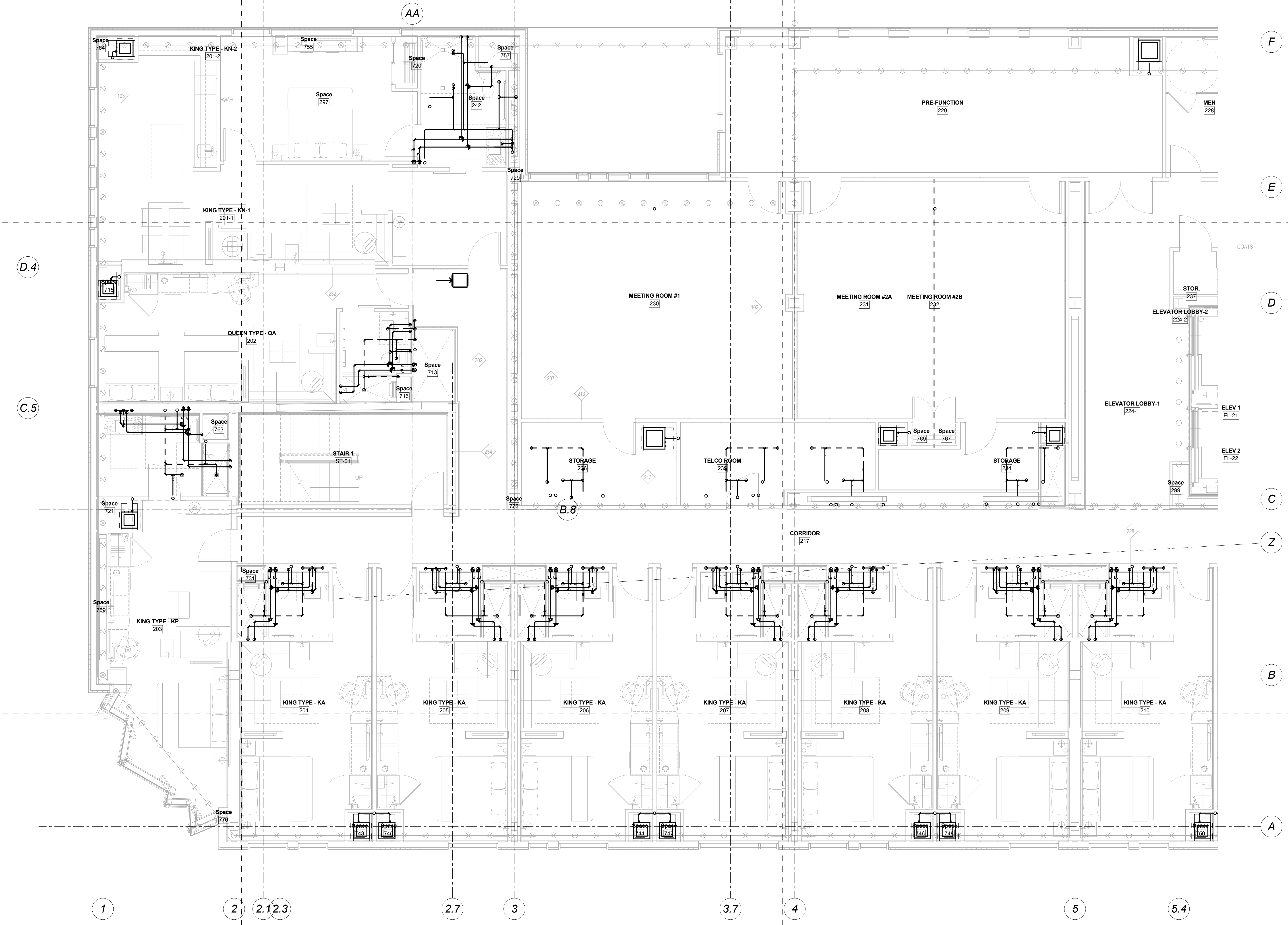
1 Second Floor Plumbing Plan-Part A 1/4" = 1'-0"
