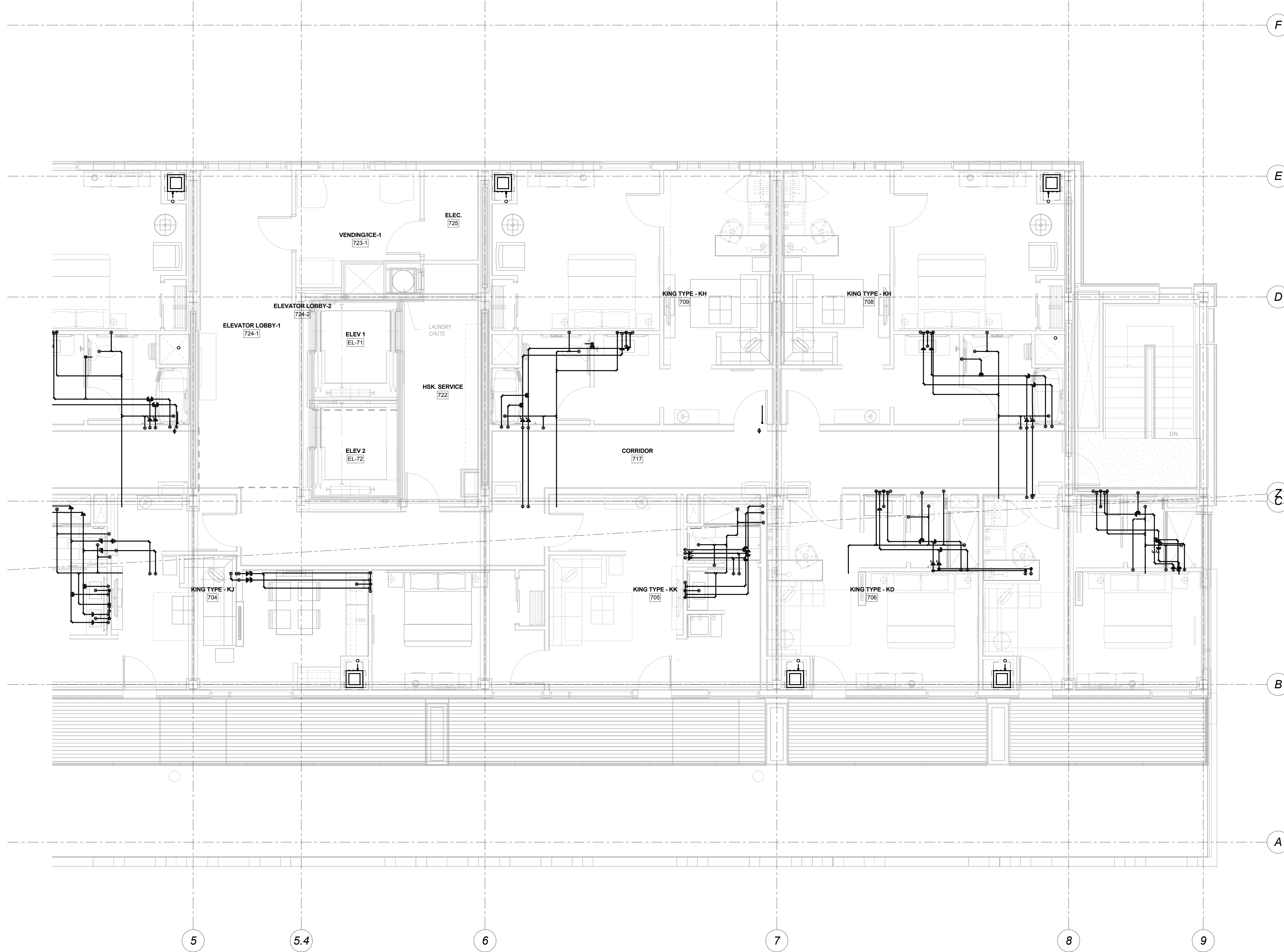
① Seventh Floor Plumbing Plan-Part B 1/4" = 1'-0"
