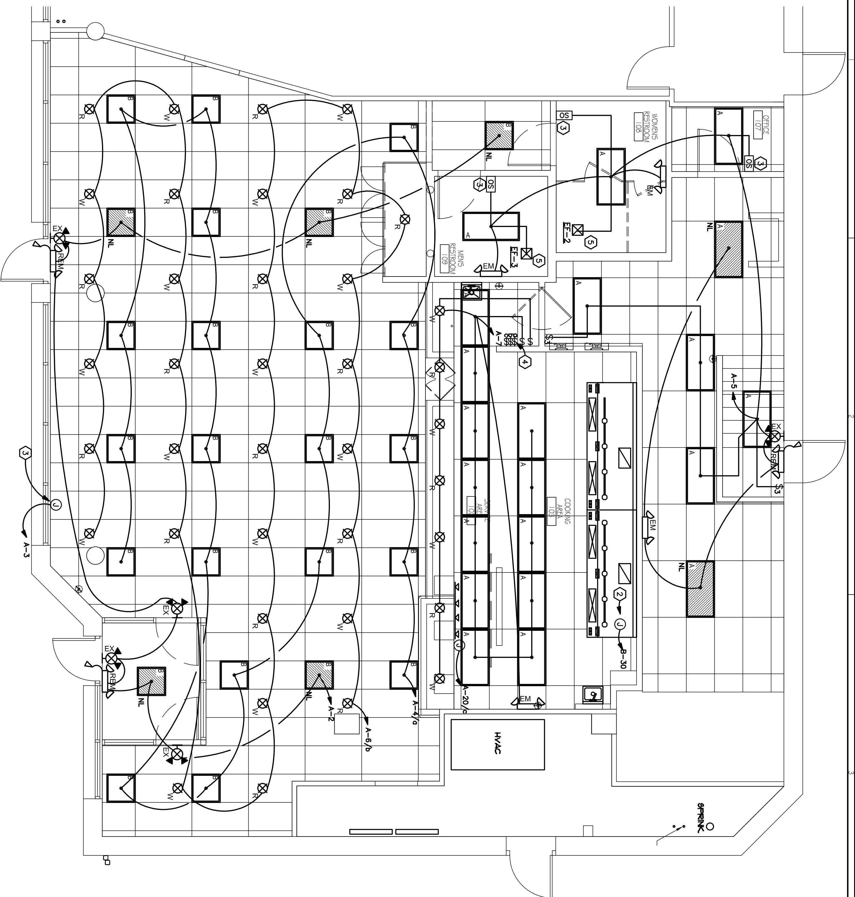
LIGHTING PLAN 1/4"=1'-0"
