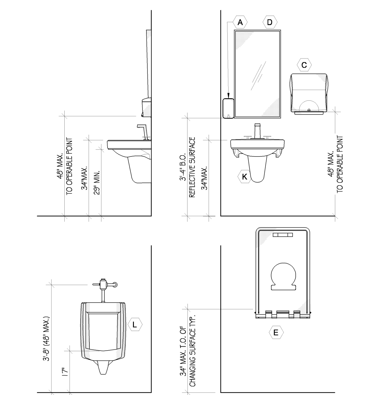
A4 REQUIRED ACCESSIBLE FIXTURE CLEARANCES
