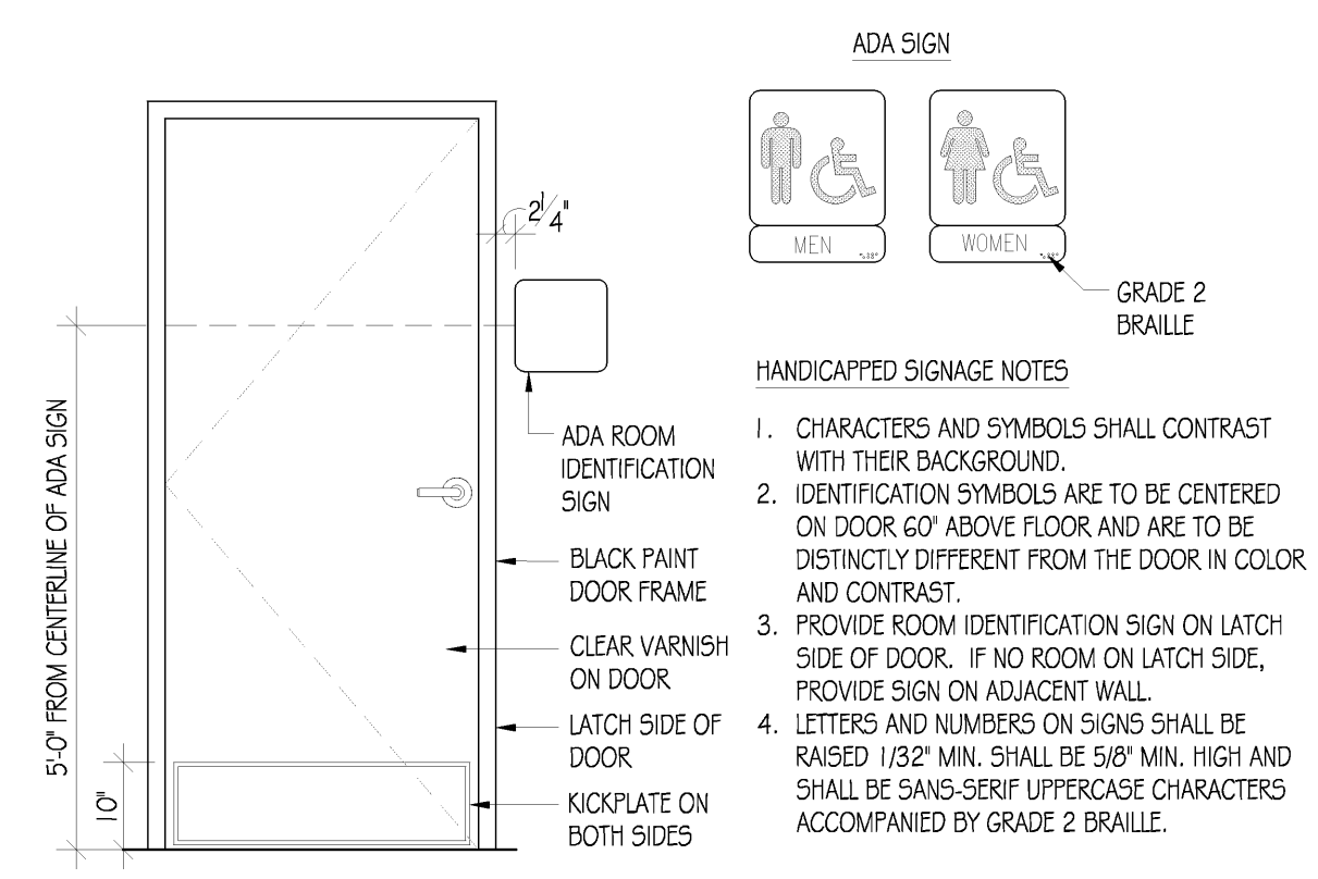
C2 ACCESSIBLE RESTROOM SIGNAGE DETAIL
