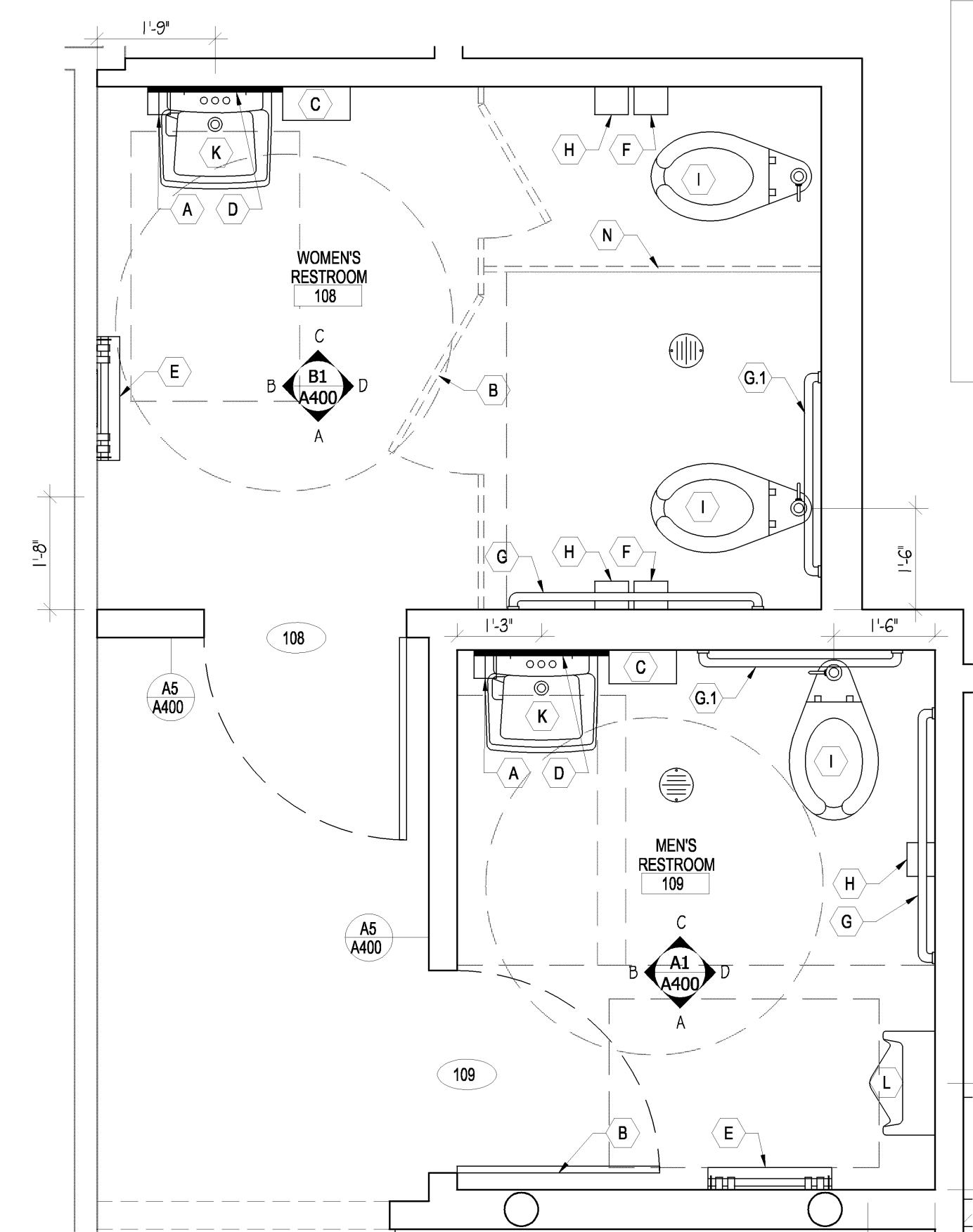
C1 ENLARGED RESTROOM PLAN
