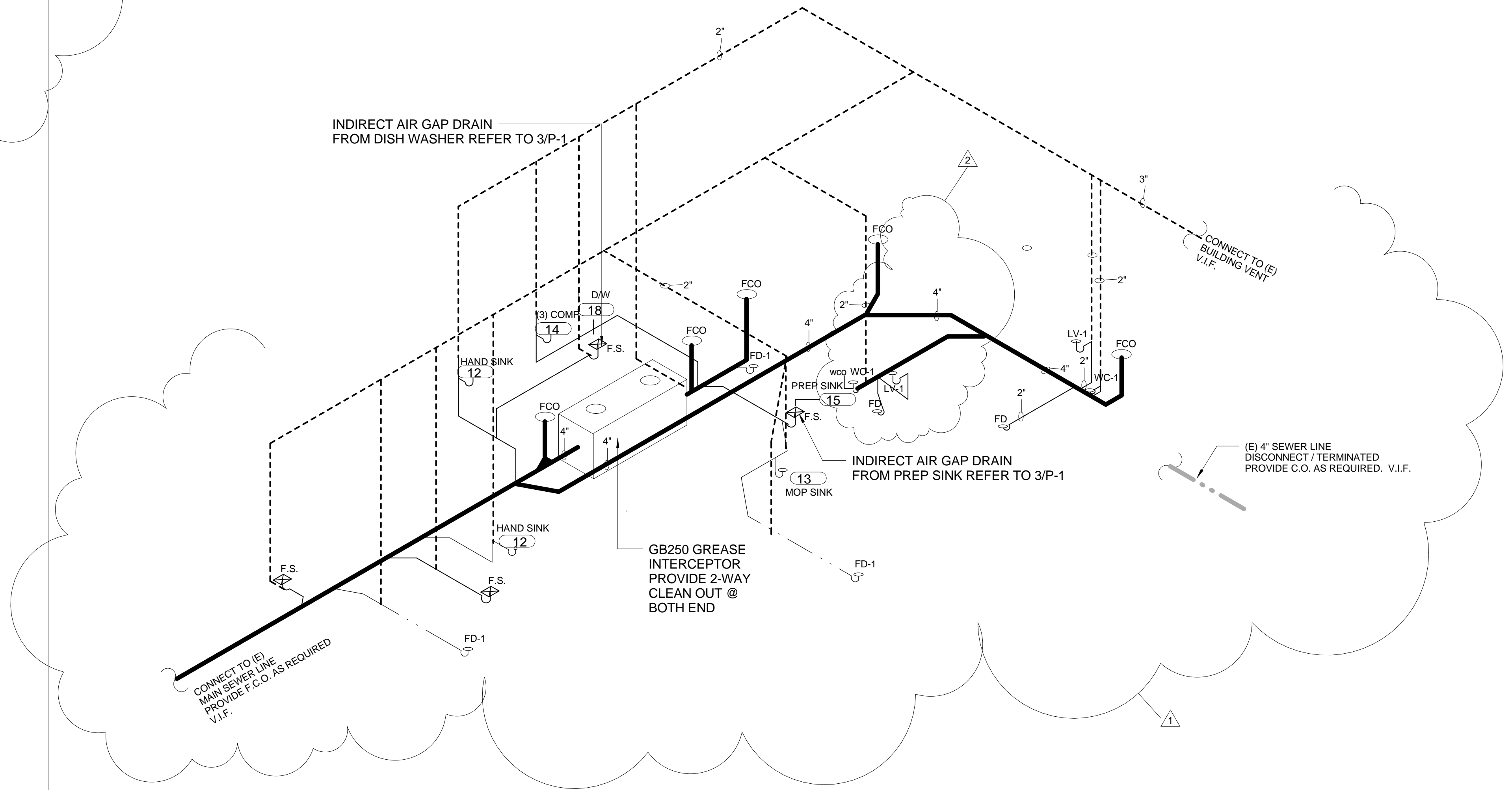
2 WASTE & VENT RISER DIAGRAM 1/4" = 1'-0"
