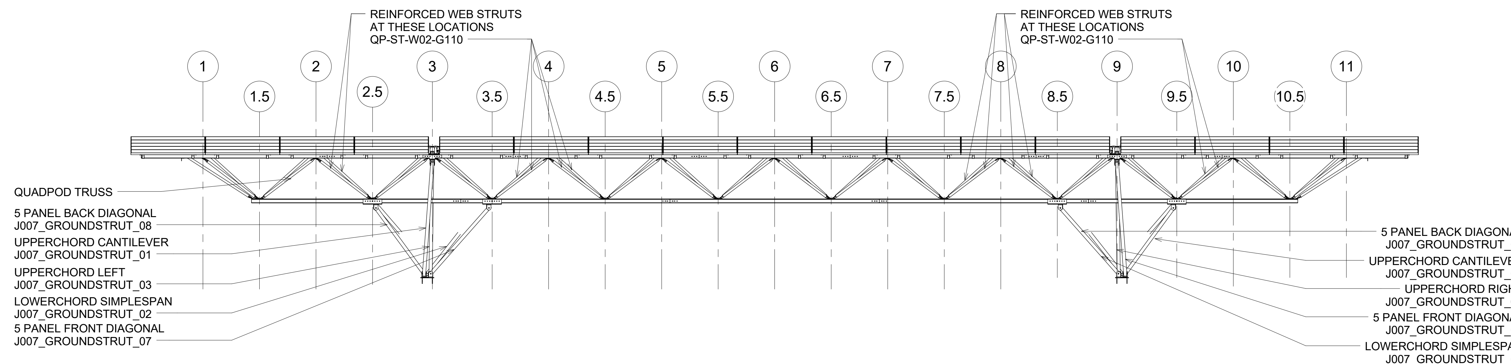
2 TRUSS ELEVATION - GROUND STRUT CONFIGURATION 3/16" = 1'-0"
