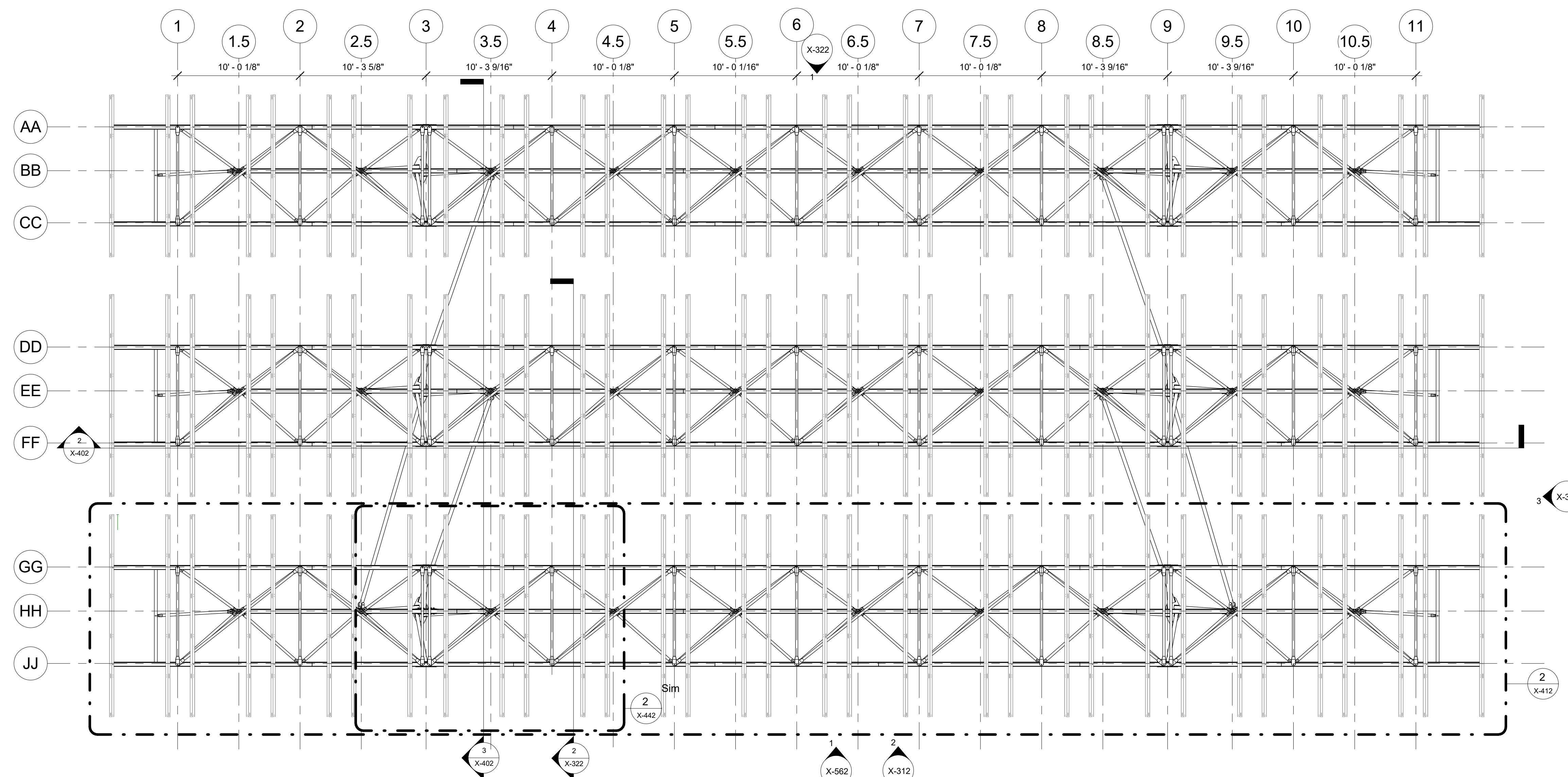
1 TRUSS PLAN - PAIR 3/16" = 1'-0"
