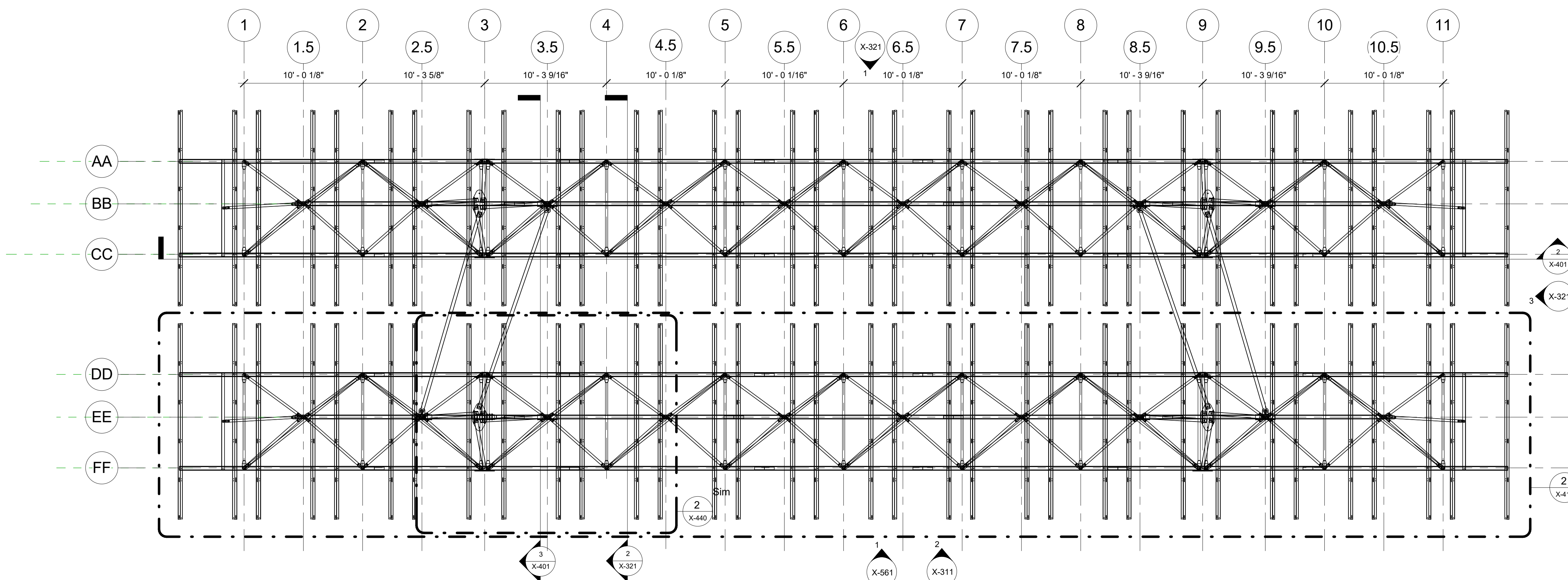
1 TRUSS PLAN - PAIR 3/16" = 1'-0"
