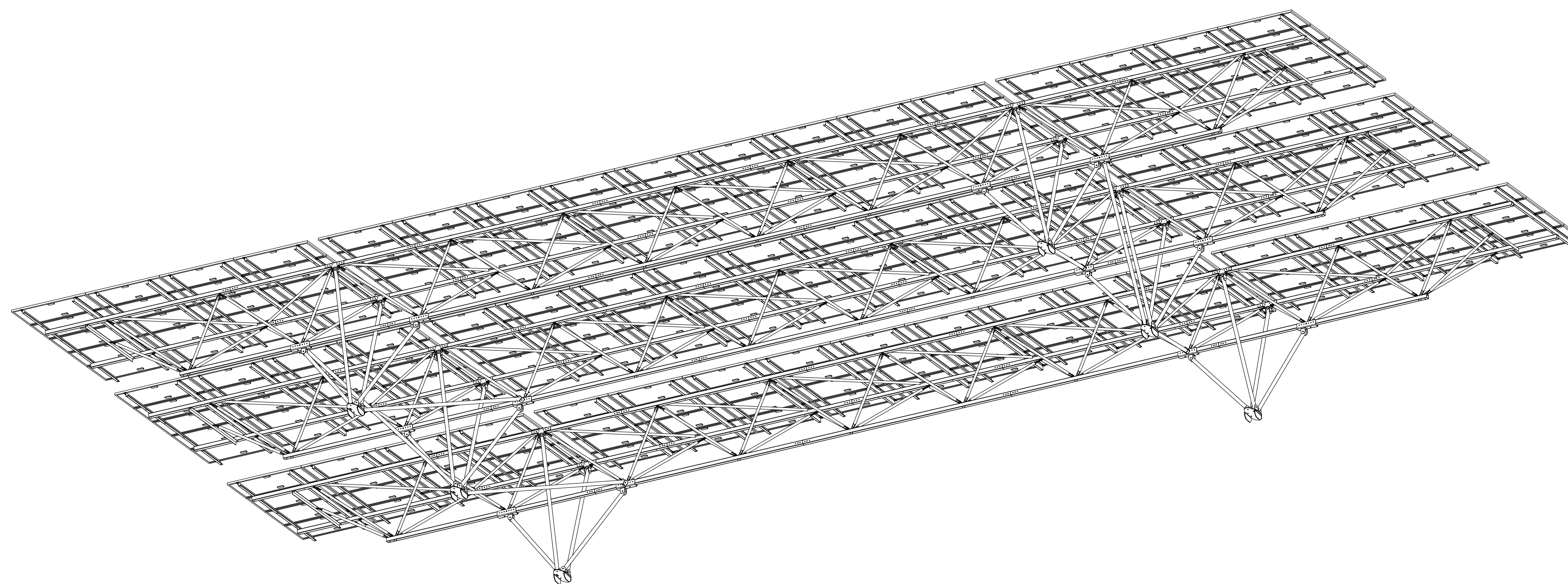
2 CONFIGURATION 2 - SYSTEM AXONOMETRIC - UNDER SIDE
