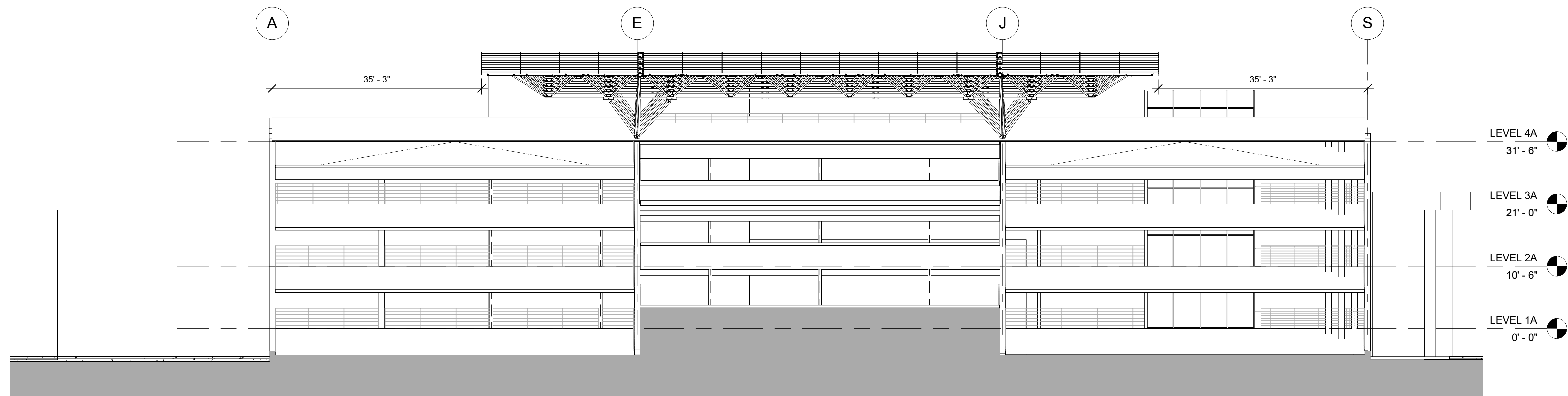
1 EAST-WEST SITE SECTION 3/32" = 1'-0"
