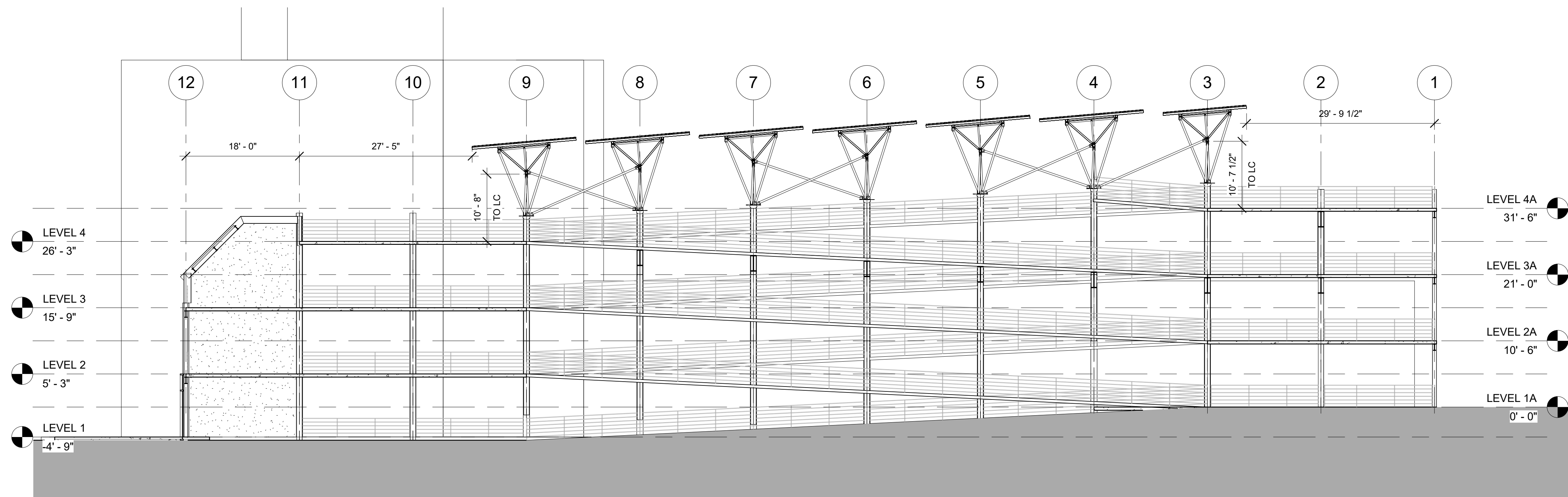
2 NORTH-SOUTH SITE SECTION 3/32" = 1'-0"
