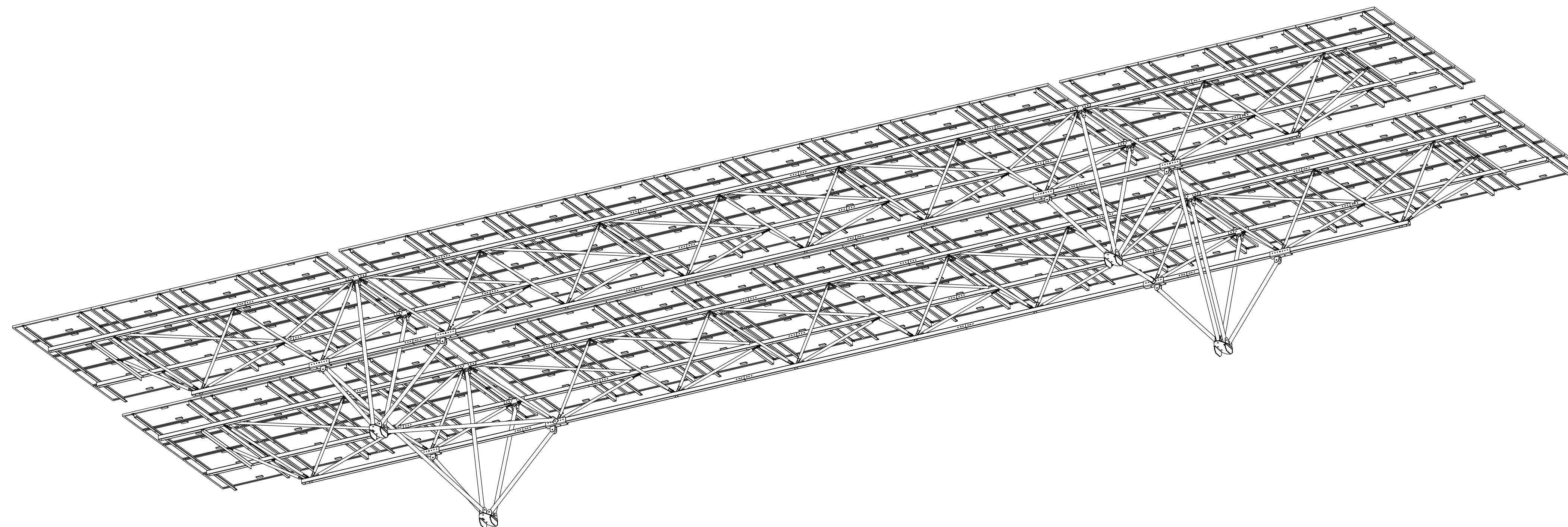
2 CONFIGURATION 1 - SYSTEM AXONOMETRIC - UNDER SIDE
