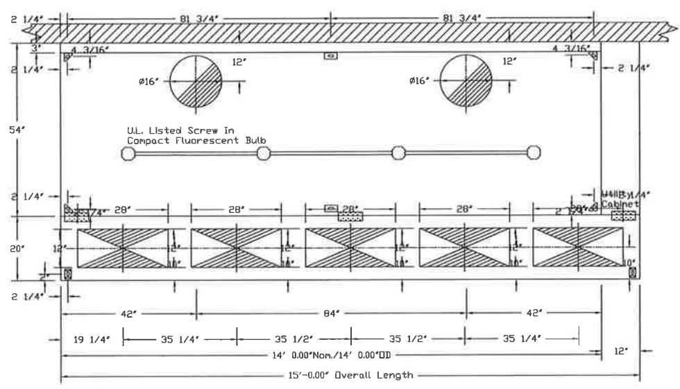
PLAN VIEW - Hood #1 14' 0.00" LONG 5424ND-2-PSP-F NOTE: Additional hanging angles provided for hoods 12' and longer.
