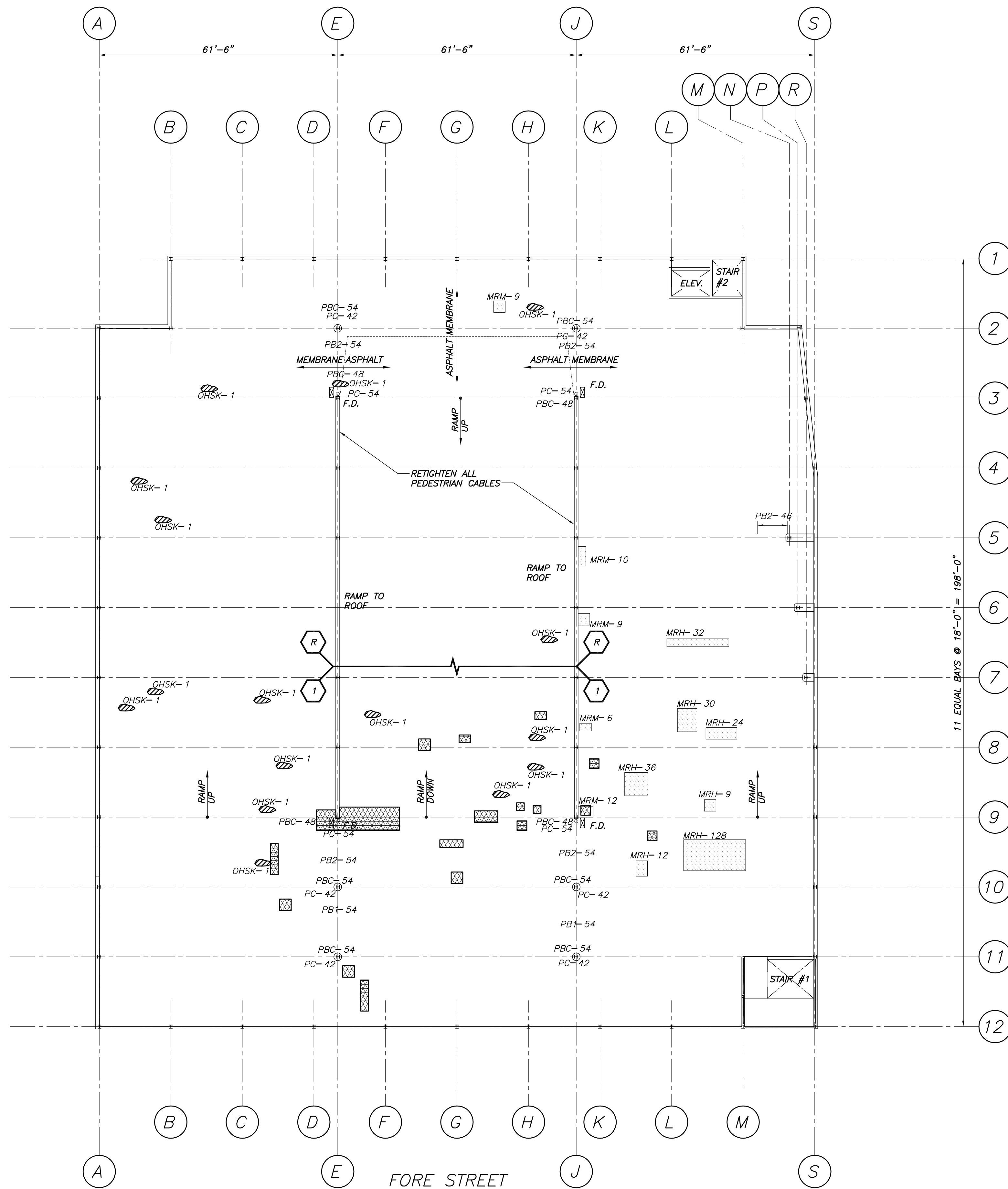
2ND SUPPORTED LEVEL SLAB PLAN 1/16"=1'-0"
