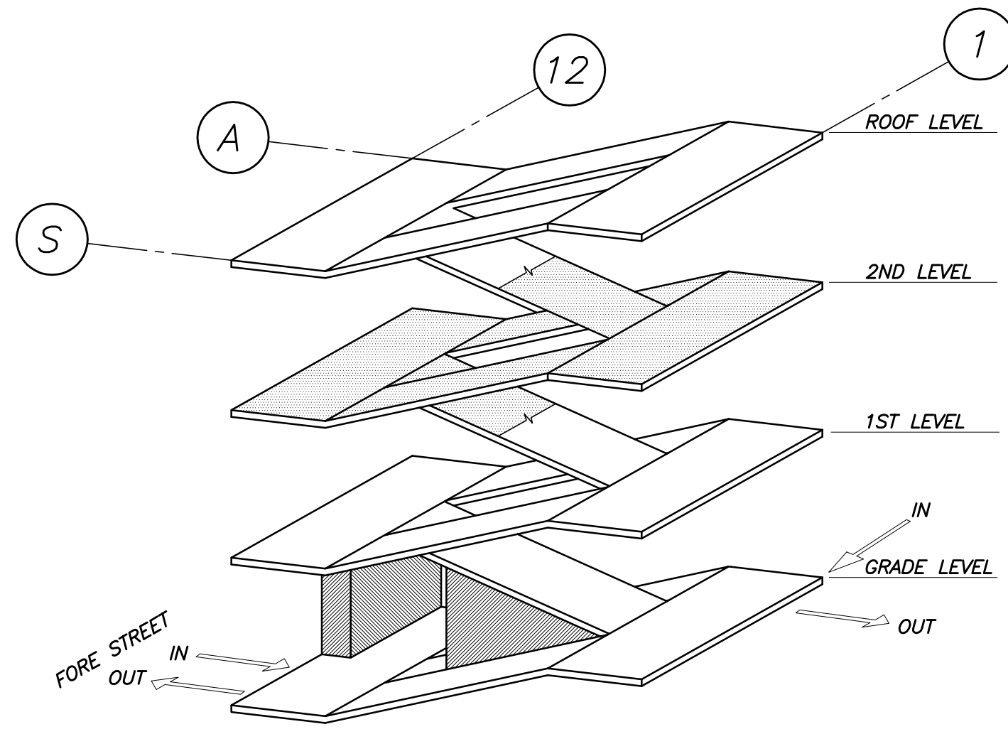
ISOMETRIC KEY
