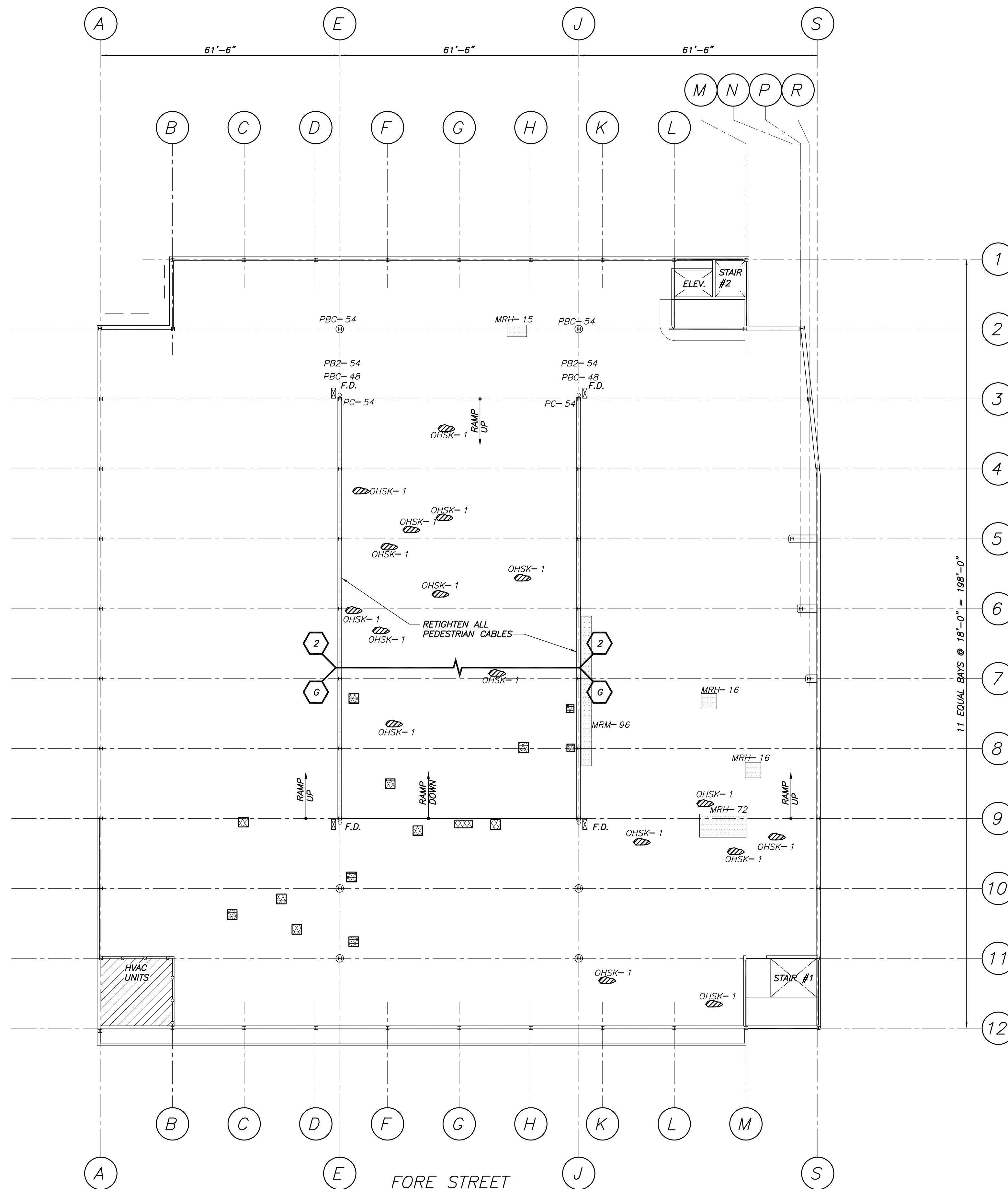
1ST SUPPORTED LEVEL SLAB PLAN 1/16"=1'-0"
