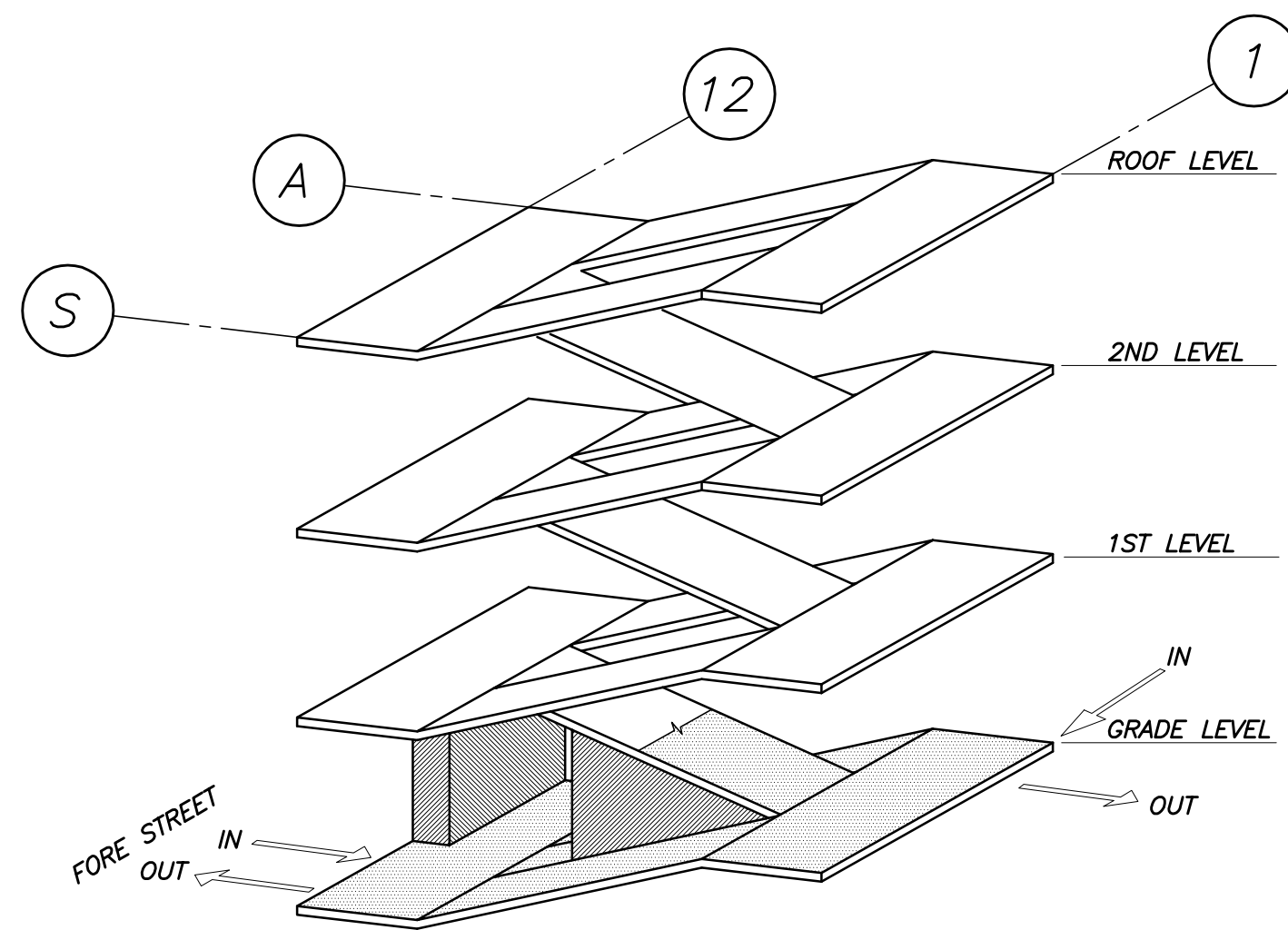
ISOMETRIC KEY
