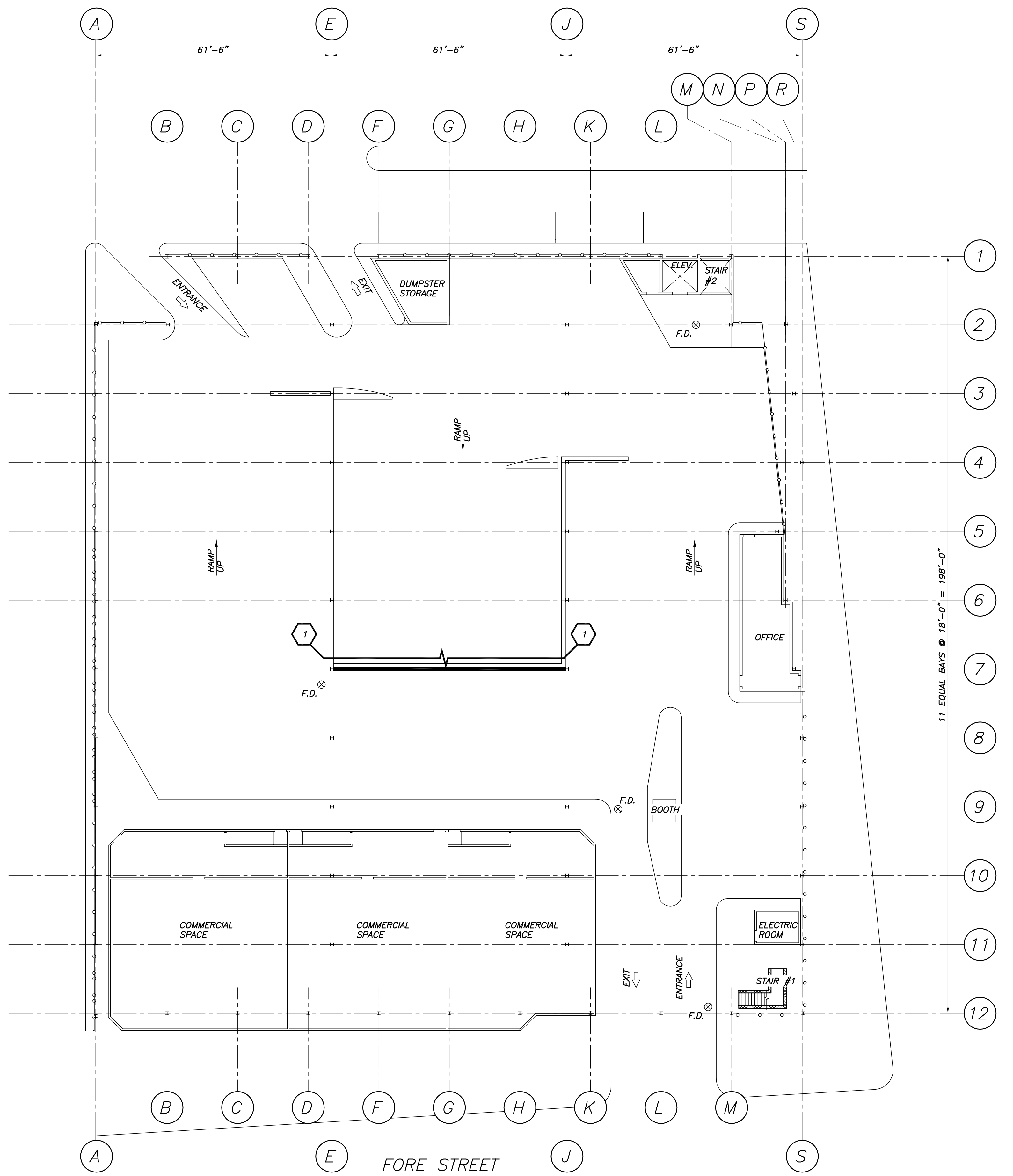
GRADE LEVEL SLAB PLAN 1/16"=1'-0"
