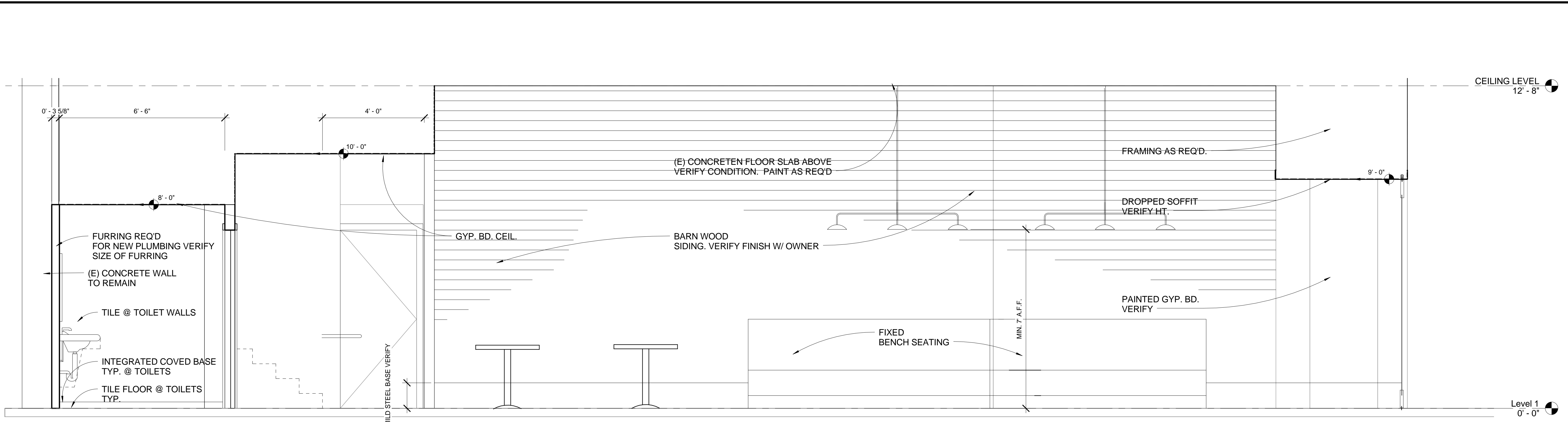
1 Section 2 1/2" = 1'-0"
