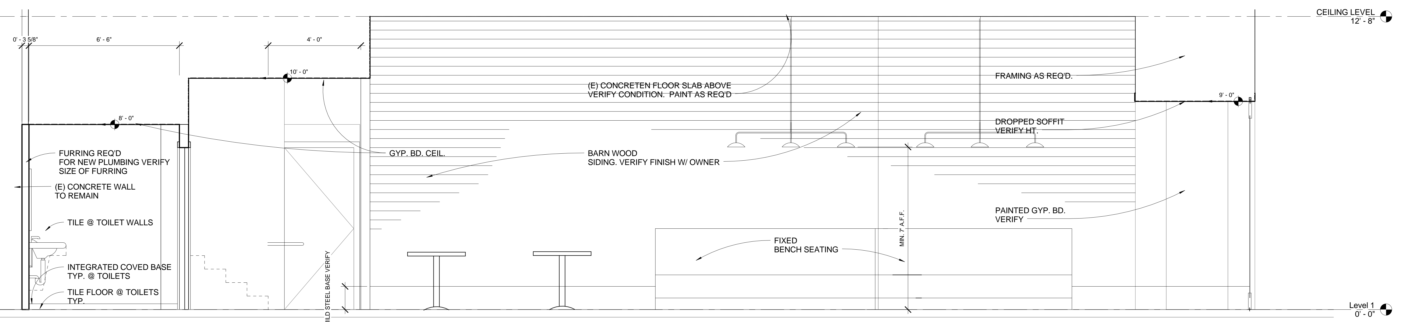
1 Section 2 1/2" = 1'-0"
