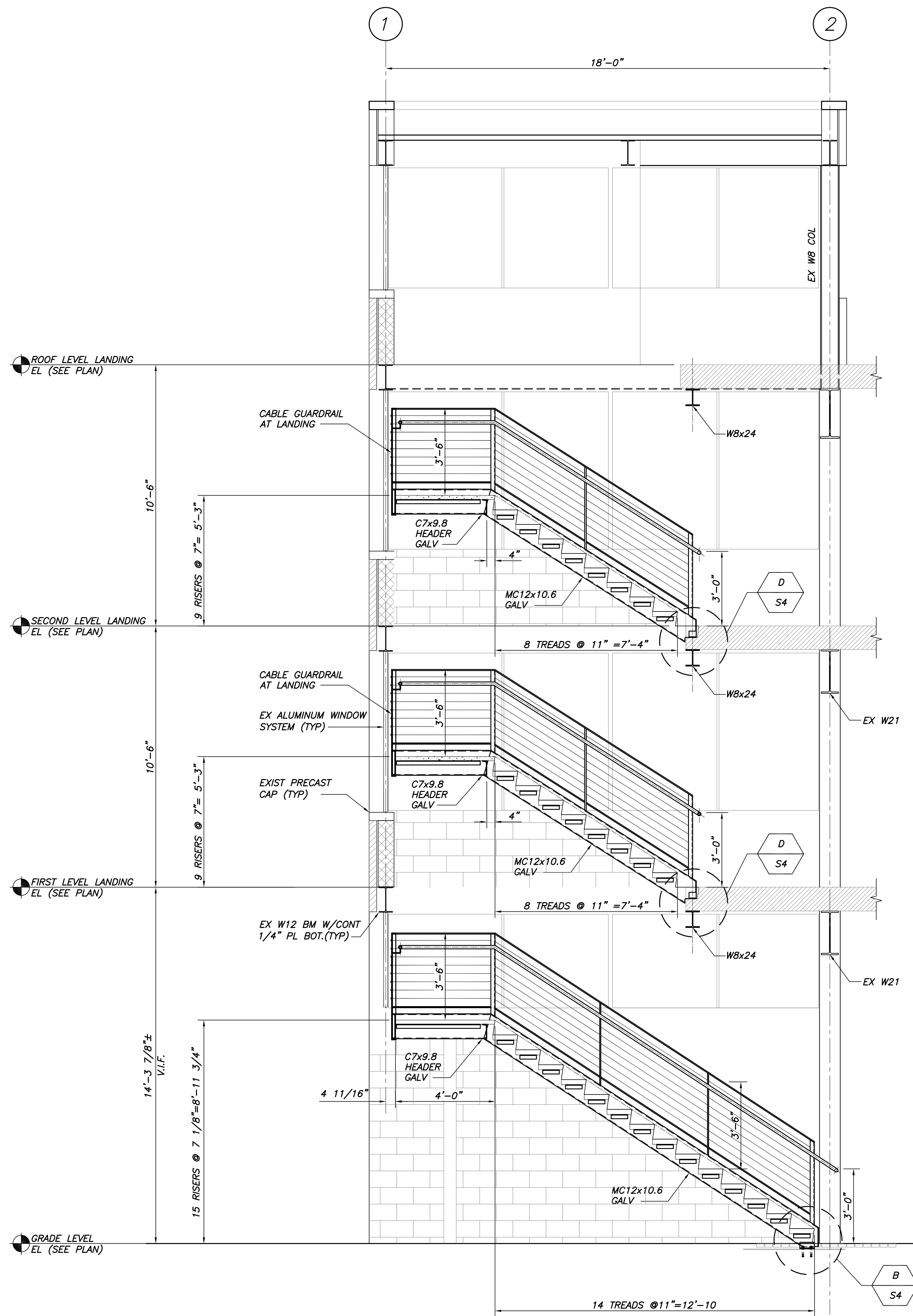
SECTION 2 3/8"=1'-0"
