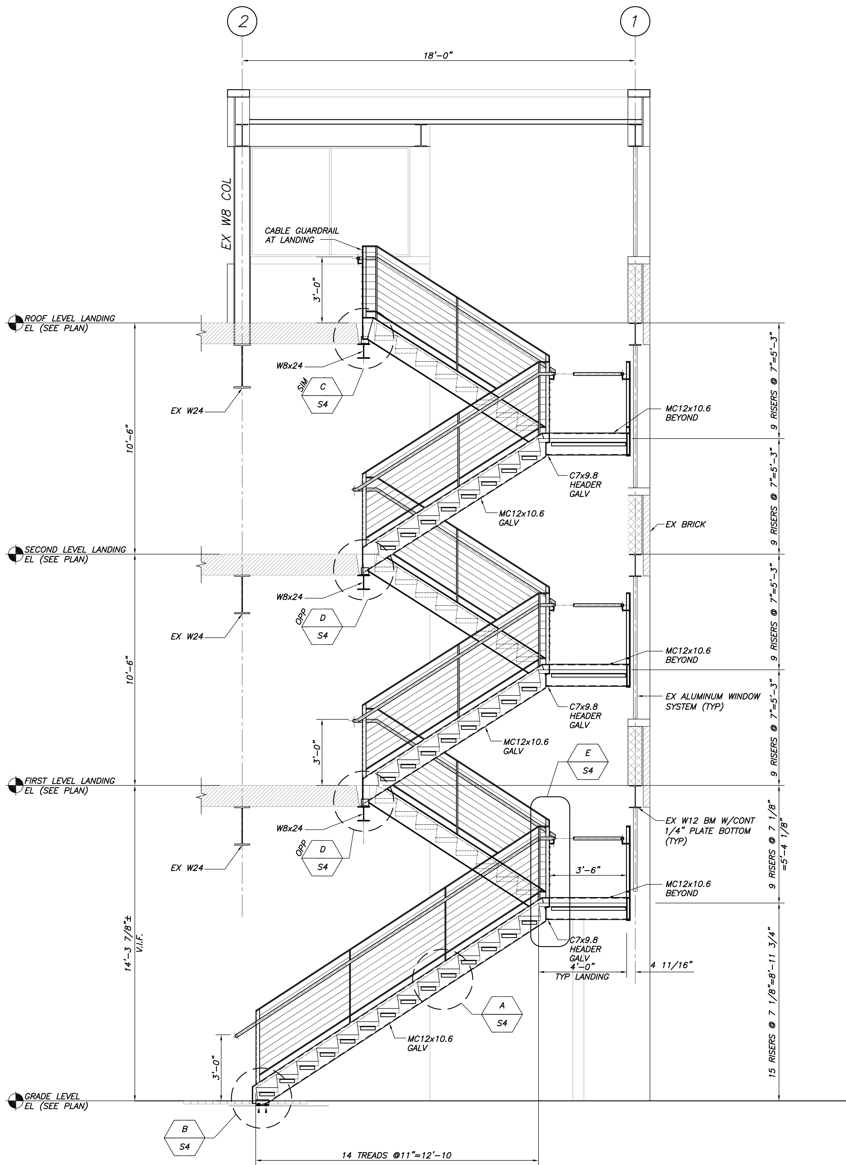
SECTION 1 3/8"=1'-0"
