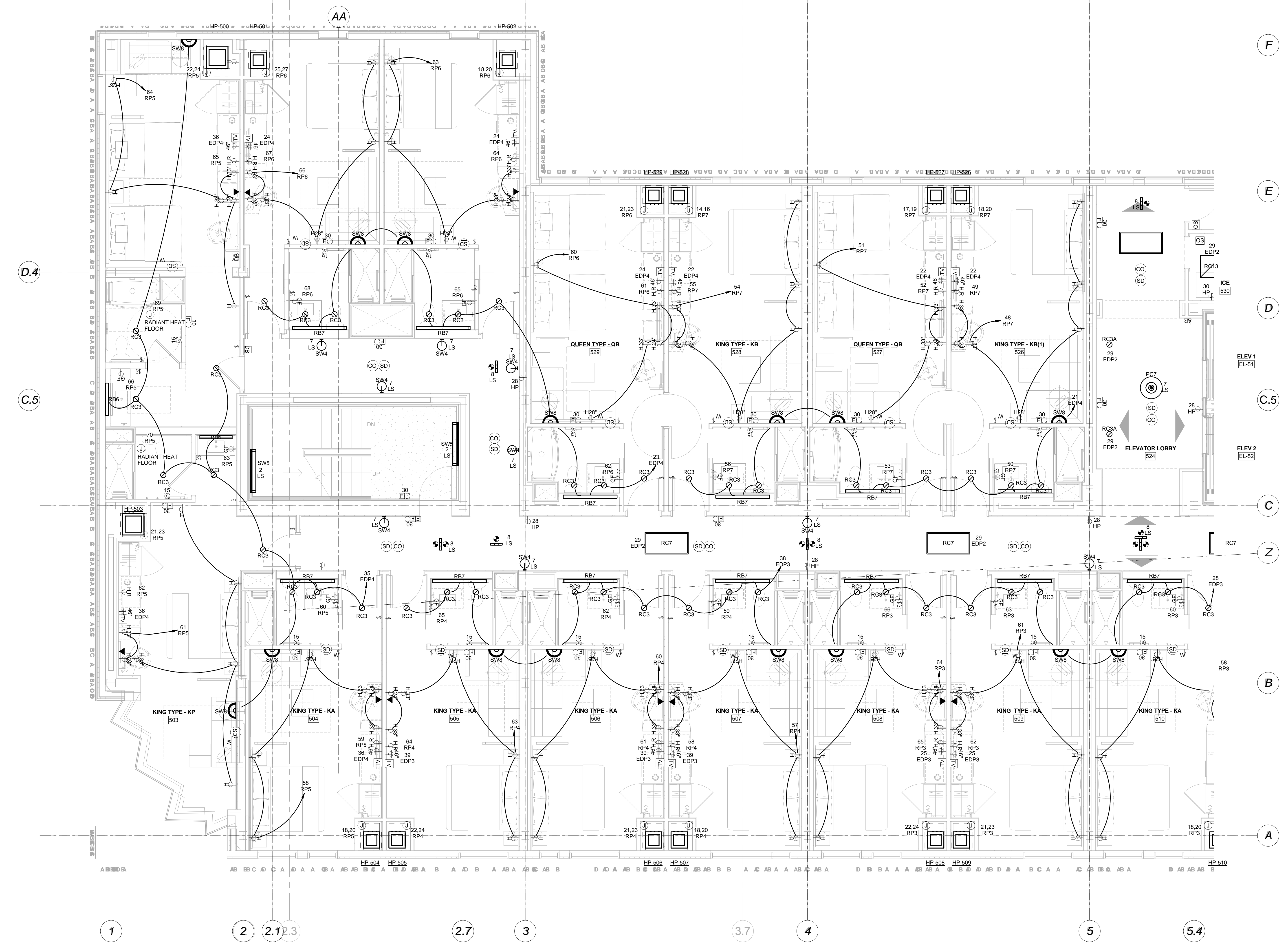
1 Fifth Floor Electrical Plan-Part A 1/4" = 1'-0"
