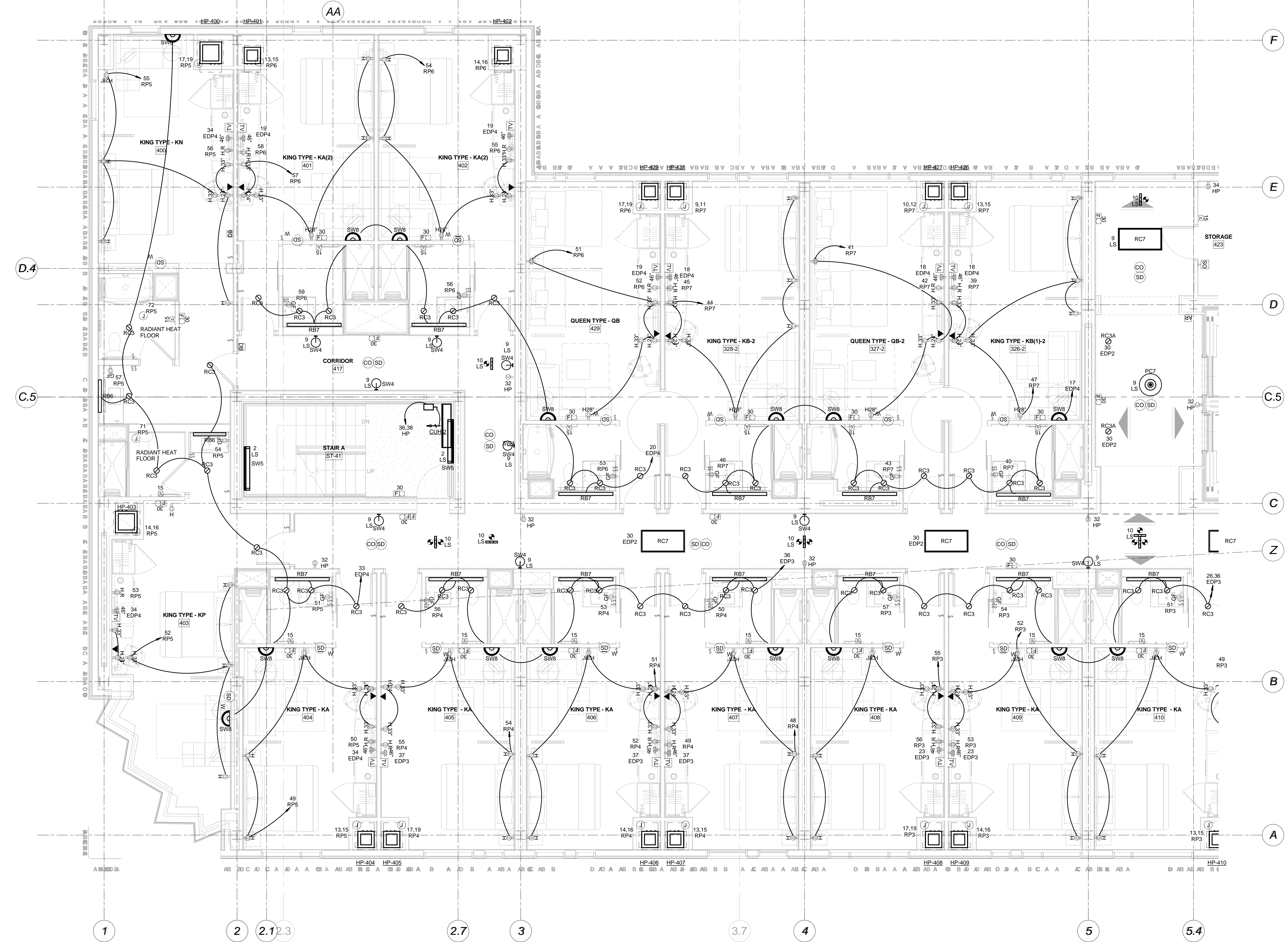
1 Fourth Floor Electrical Plan-Part A 1/4" = 1'-0"
