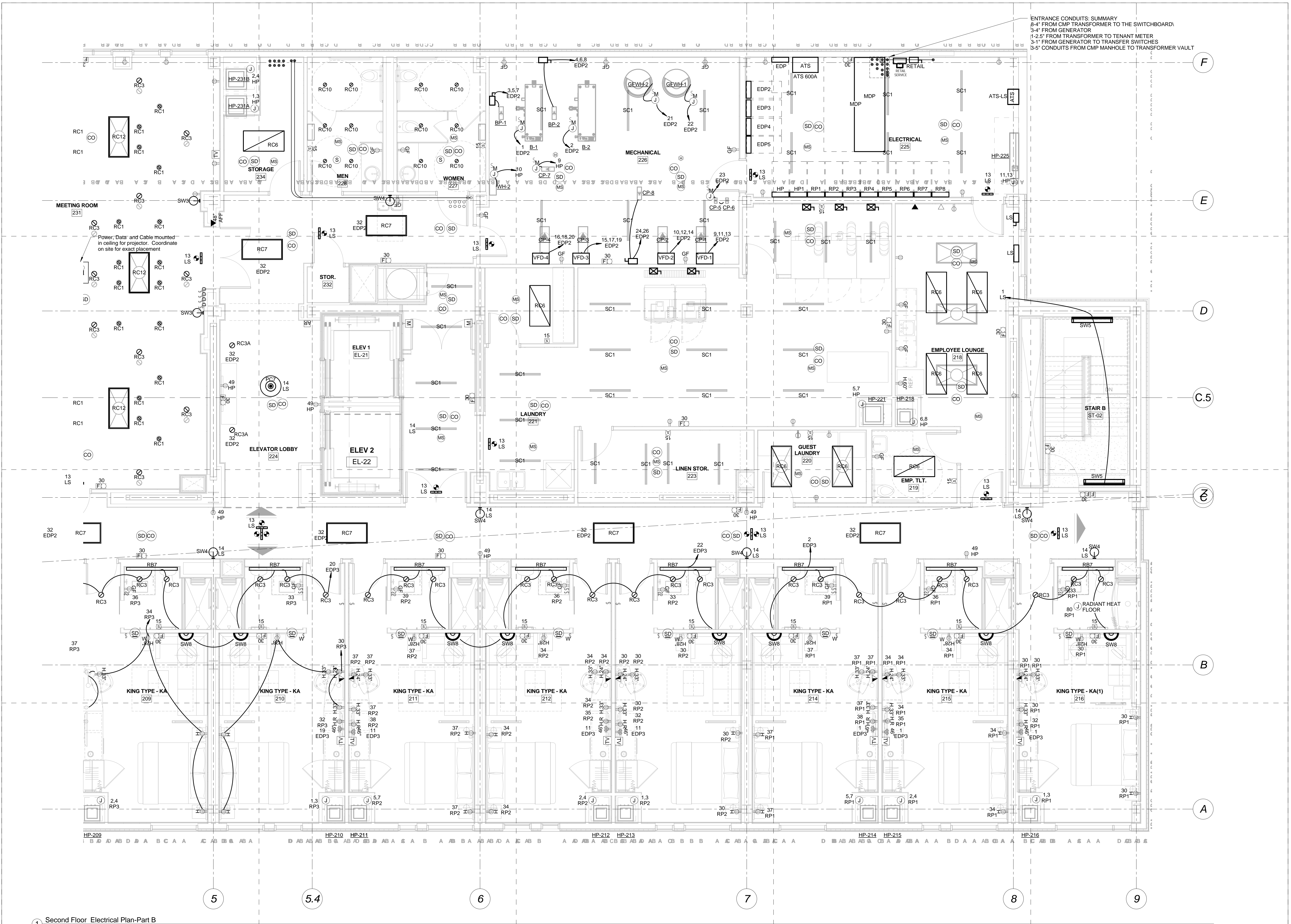
1 Second Floor Electrical Plan-Part B 1/4" = 1'-0"
