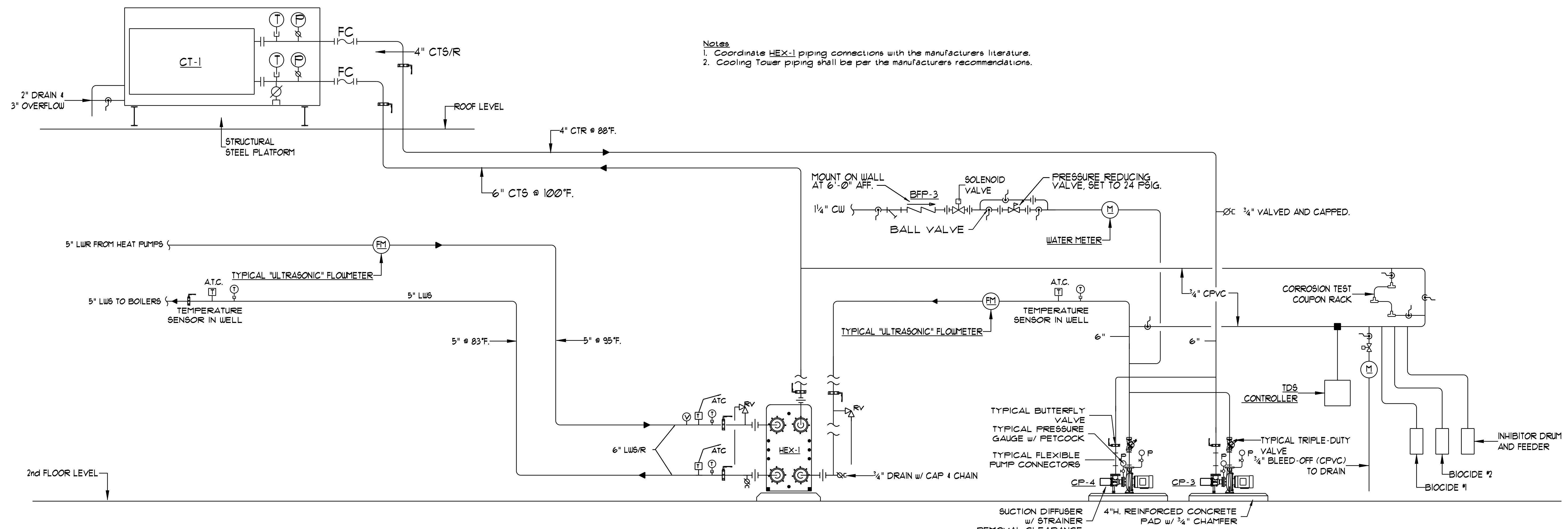
COOLING TOWER / HEX-1 PIPING SCHEMATIC AND DETAIL NTS
