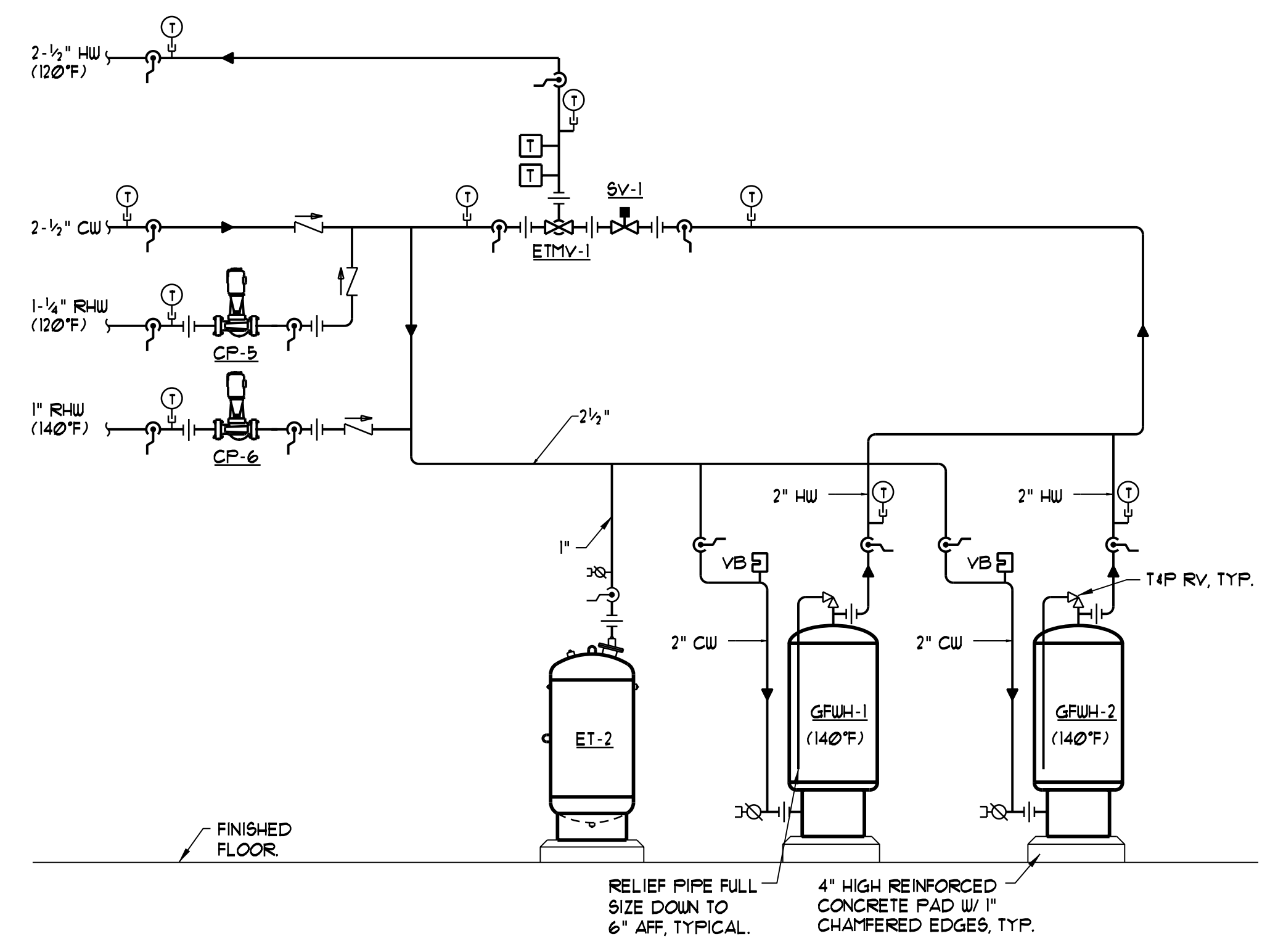
DOMESTIC HOT WATER PIPING SCHEMATIC NTS
