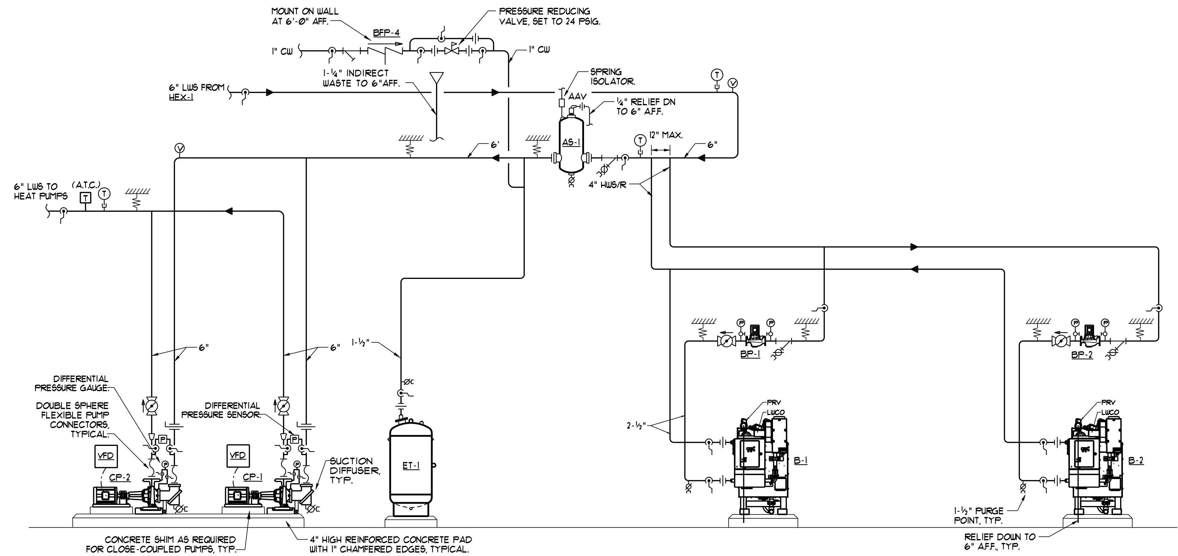
BOILER PIPING SCHEMATIC NTS
