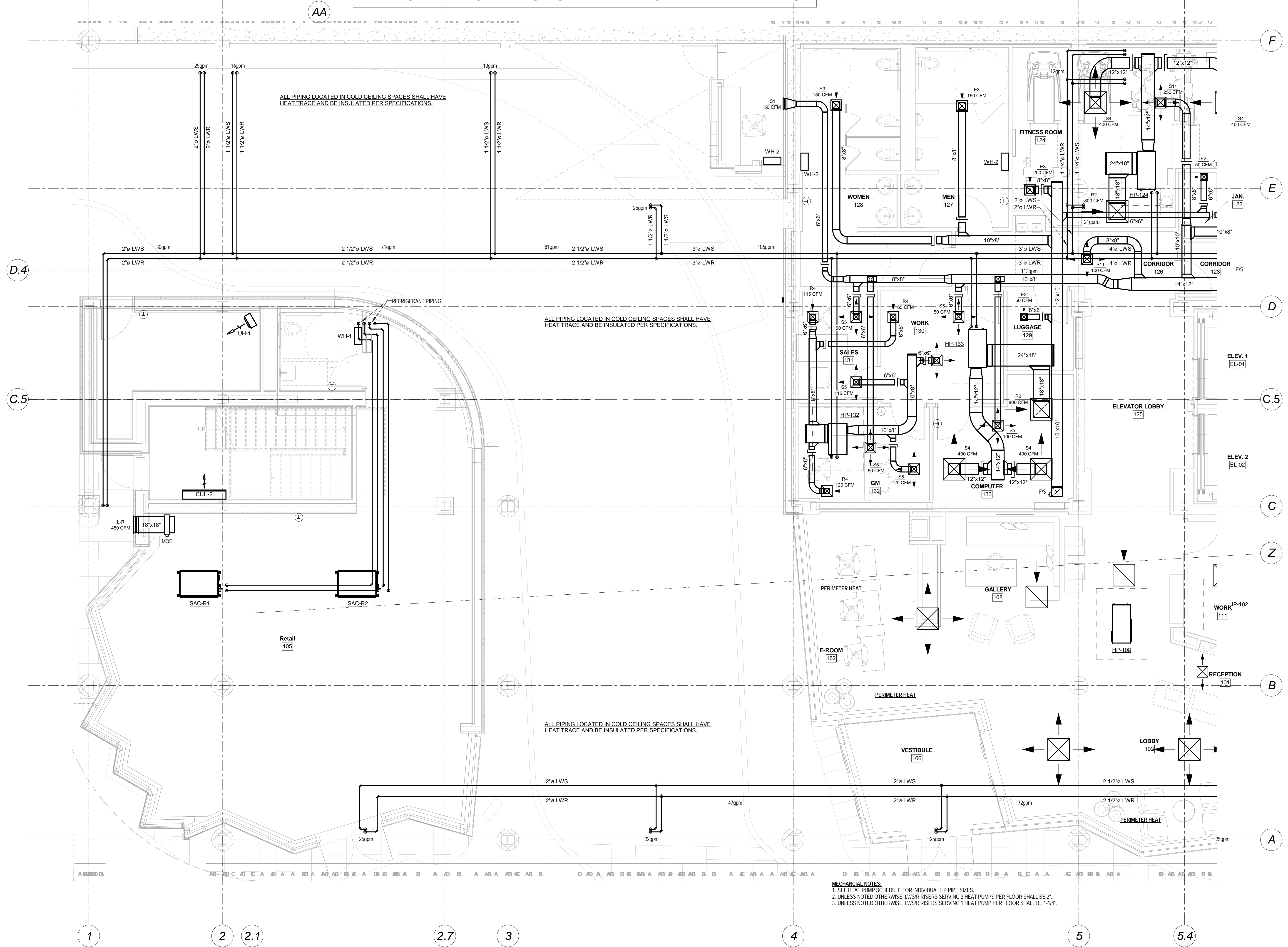
1 First Floor HVAC Plan - Part A 1/4" = 1'-0"
