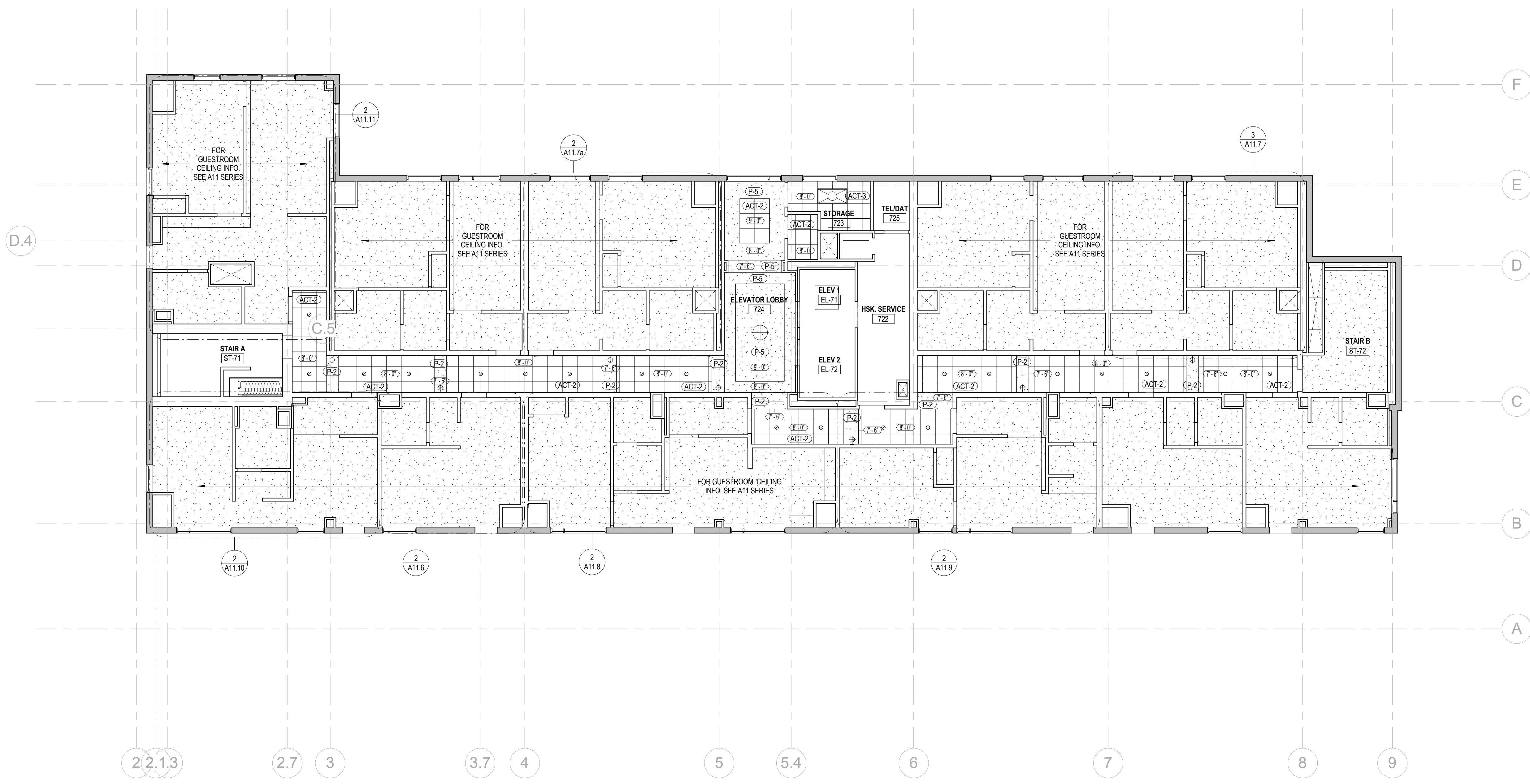
1 RCP-Level 7 1/8" = 1'-0"
